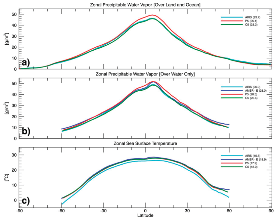
FIG. 6. Latitudinally averaged PWV (a) over both land and ocean and (b) over ocean only, and (c) SST. Note that AMSR-E has results only over ocean. Values in parentheses indicate corresponding global mean.
