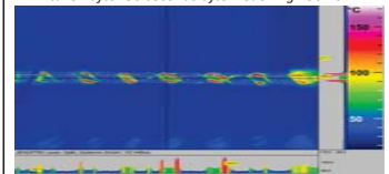
Figure 6. One Wraps/Inch Thermal Profile. Picture taken after 30 seconds after reaching 150 °C.
