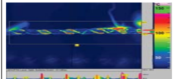
Figure 5. Two Wraps/Inch Thermal Profile. Picture taken after 30 seconds after reaching 150 °C.
