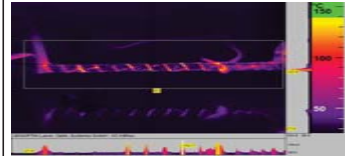
Figure 4. Three Wraps/Inch Thermal Profile. Picture taken after 30 seconds after reaching 150 °C.
