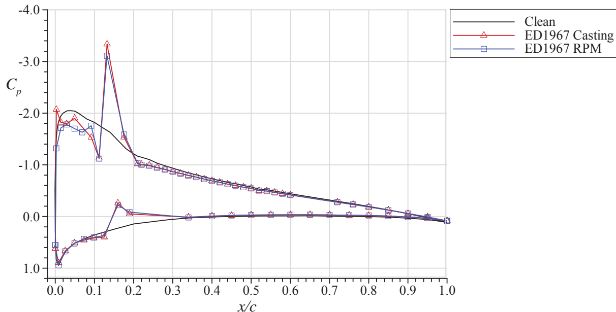
Figure 18. Pressure distribution comparison for the ED1967 spanwise-ridge ice shape with casting and RPM simulations on the NACA 23012 airfoil at \alpha = 6.2 deg., Re = 1.8 \times 10^6 and M = 0.18 .
