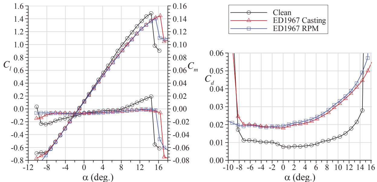
Figure 17. Aerodynamic performance comparison for the ED1967 spanwise-ridge ice-shape casting and RPM simulations on the NACA 23012 airfoil at Re = 1.8 \times 10^6 and M = 0.18 .
