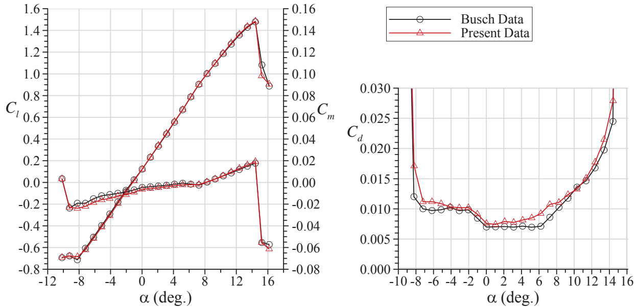
Figure 9. Clean NACA 23013 airfoil aerodynamic performance comparison for the present data with past results from Busch 14 at Re = 1.8 \times 10^6 and M = 0.18 .
