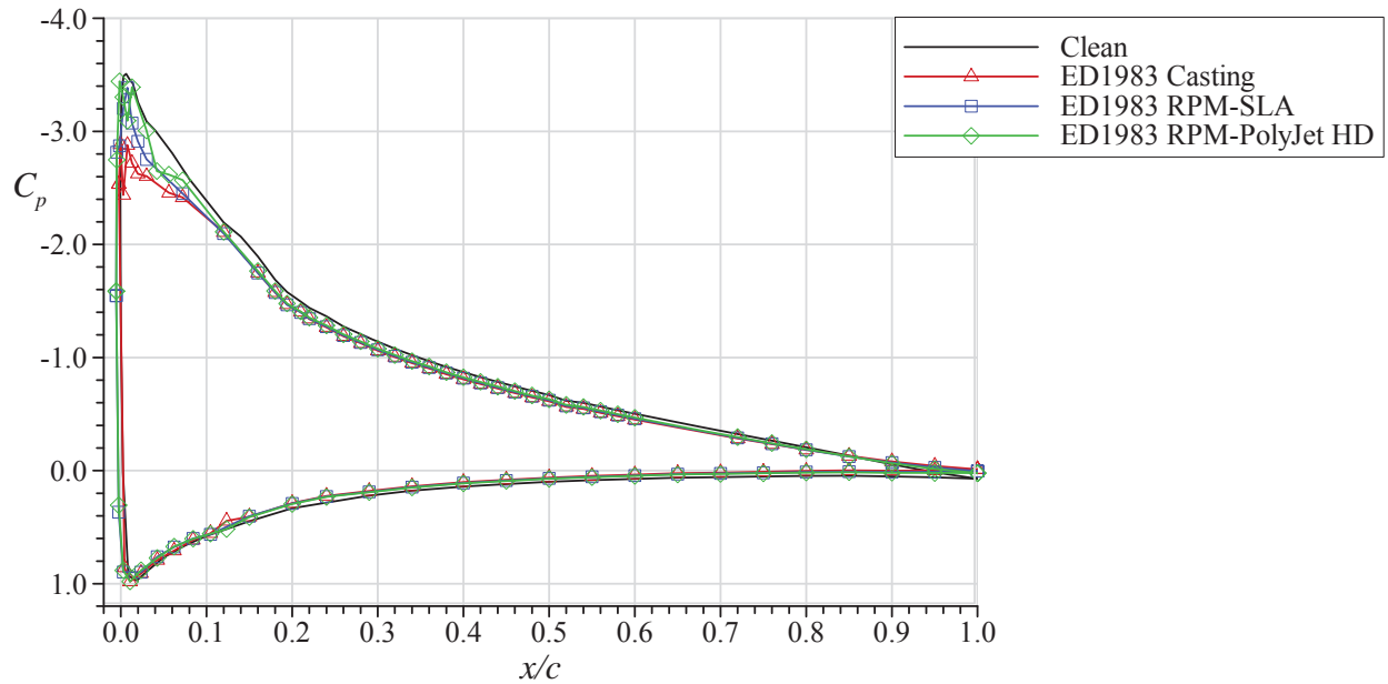
Figure 13. Pressure distribution comparison for the ED1983 roughness with casting and RPM simulations on the NACA 23012 airfoil at \alpha = 9.3 deg., Re = 1.8 \times 10^6 and M = 0.18 .
