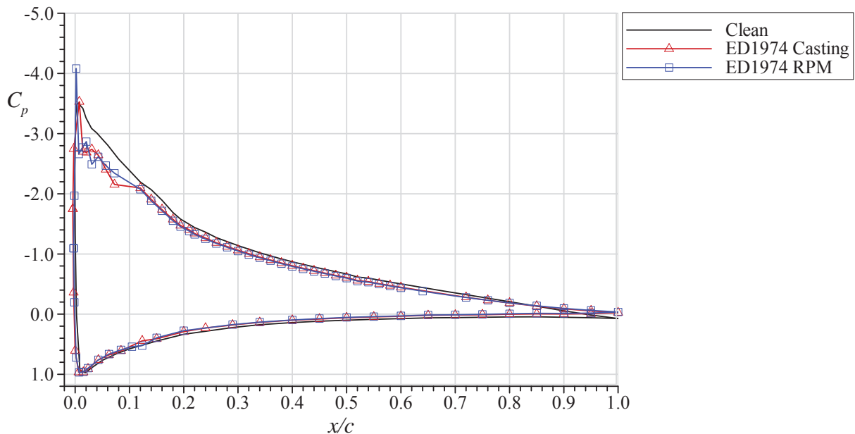
Figure 11. Pressure distribution comparison for the ED1974 roughness with casting and RPM simulations on the NACA 23012 airfoil at \alpha = 9.3 deg., Re = 1.8 \times 10^6 and M = 0.18 .
