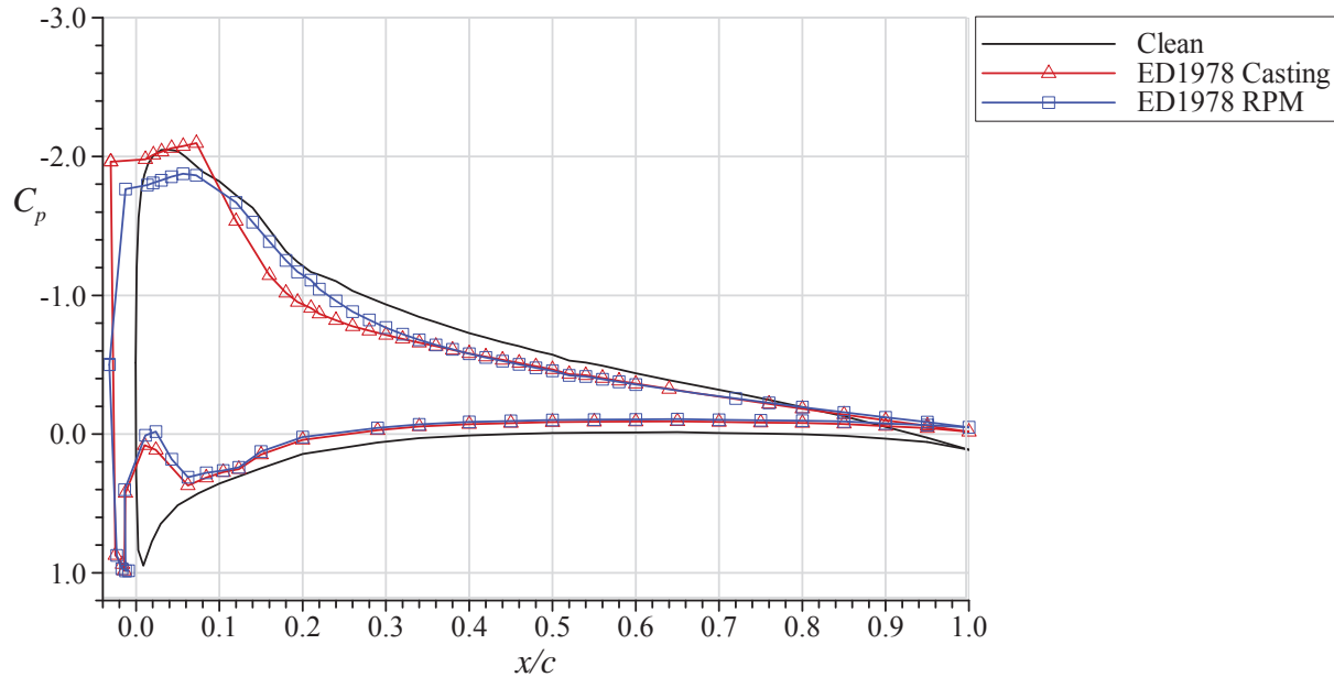
Figure 20. Pressure distribution comparison for the ED1978 horn ice shape with casting and RPM simulations on the NACA 23012 airfoil at \alpha = 6.2 deg., Re = 1.8 \times 10^6 and M = 0.18 .
