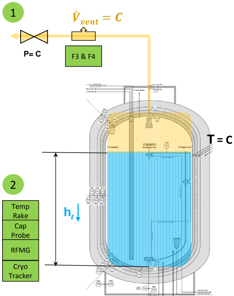
Boil-off Test
