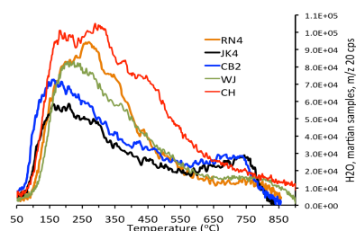
Figure 1. Sample \text{H}_2\text{O} EGA-MS traces.
