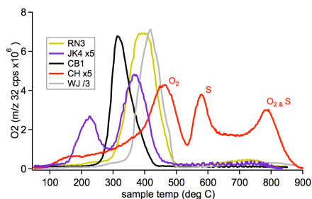
Figure 3. Sample O 2 EGA-MS traces.
