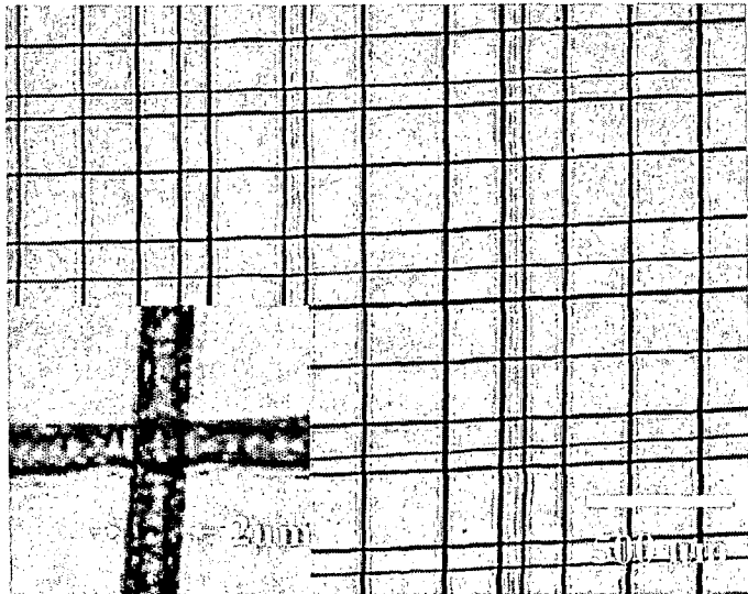
(2) CNT-Polyimide fiber mat
