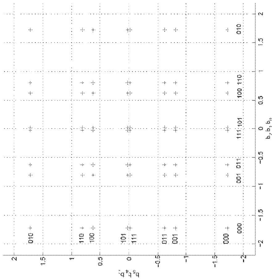
QAM-64 constructed from 2 orthogonal FAM-8 optimized for PDC=1.5 bits/dimension
