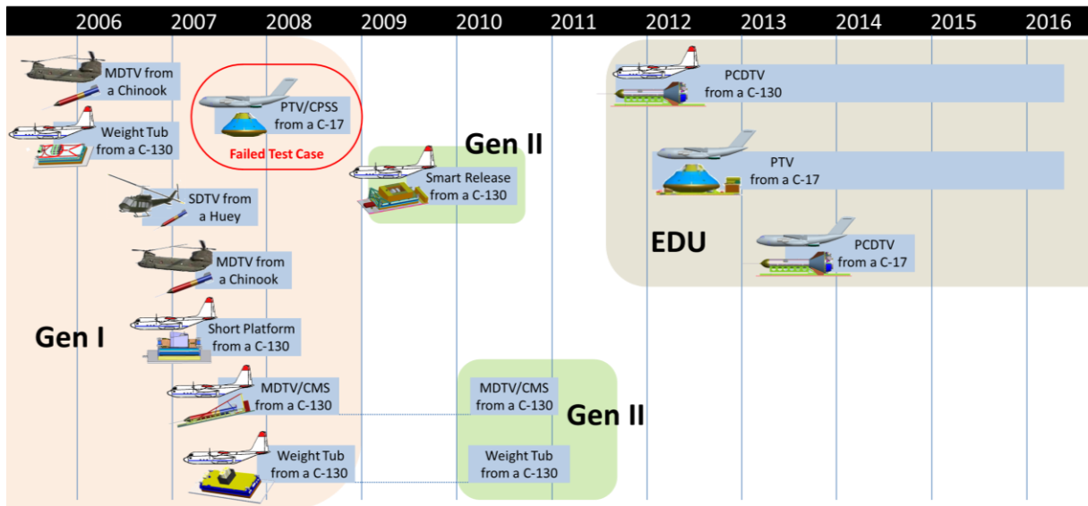
Figure 1. Evolution of CPAS test vehicles and techniques.
