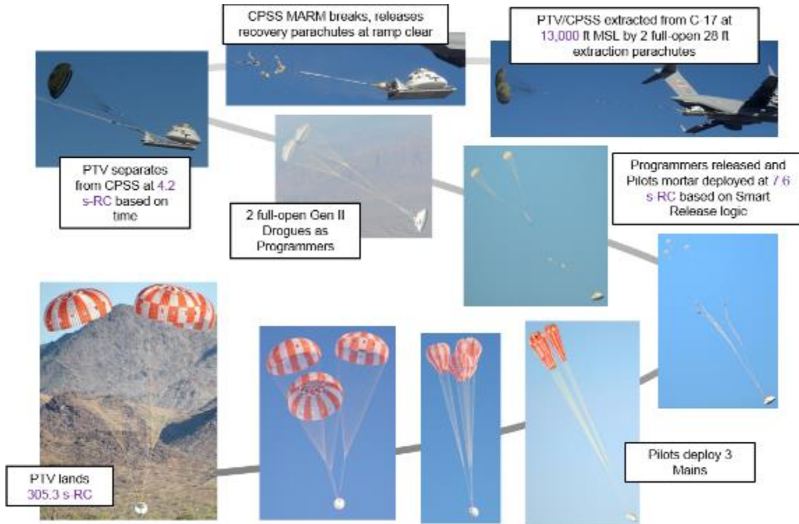
Figure 13. CDT-3-13 PTV concept of operations.
