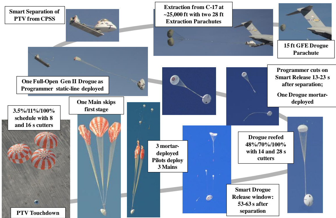
Figure 9. CDT-3-9 PTV concept of operations.
