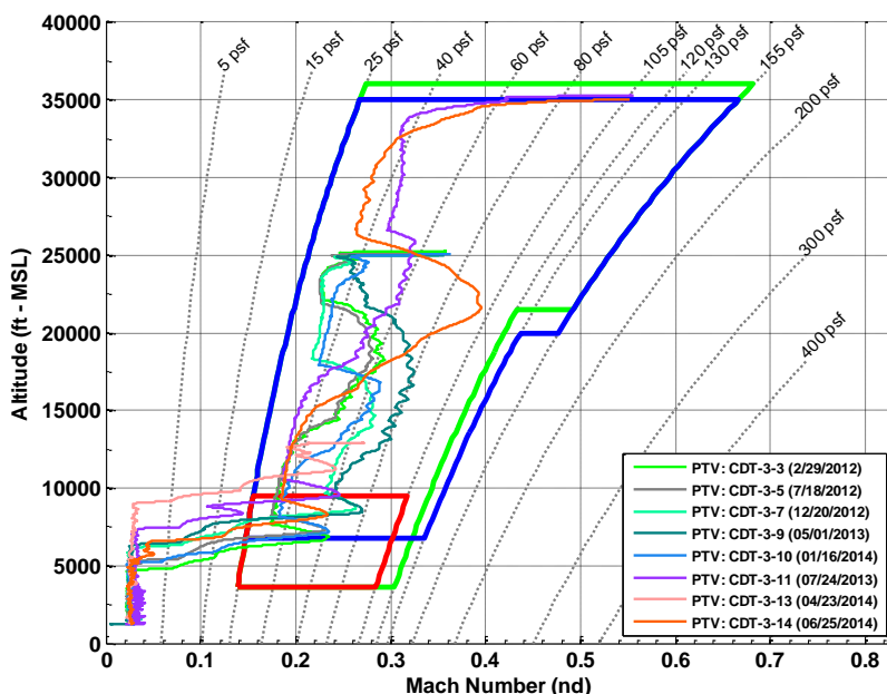
Figure 6. PTV Drop Test Trajectories.
