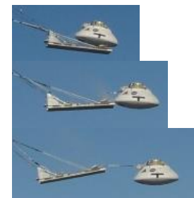
Figure 9. Stable PTV Orientation through Off-Nominal Reposition.
