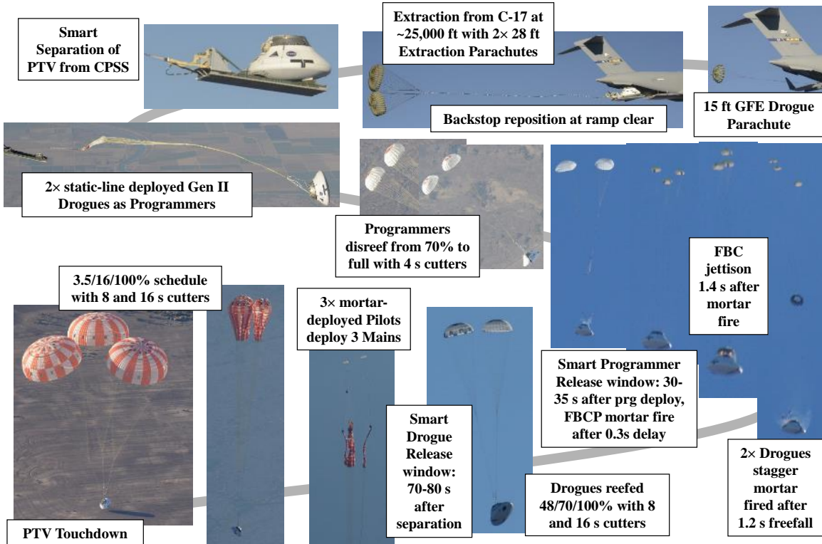
Figure 10. CDT-3-10 PTV concept of operations.
