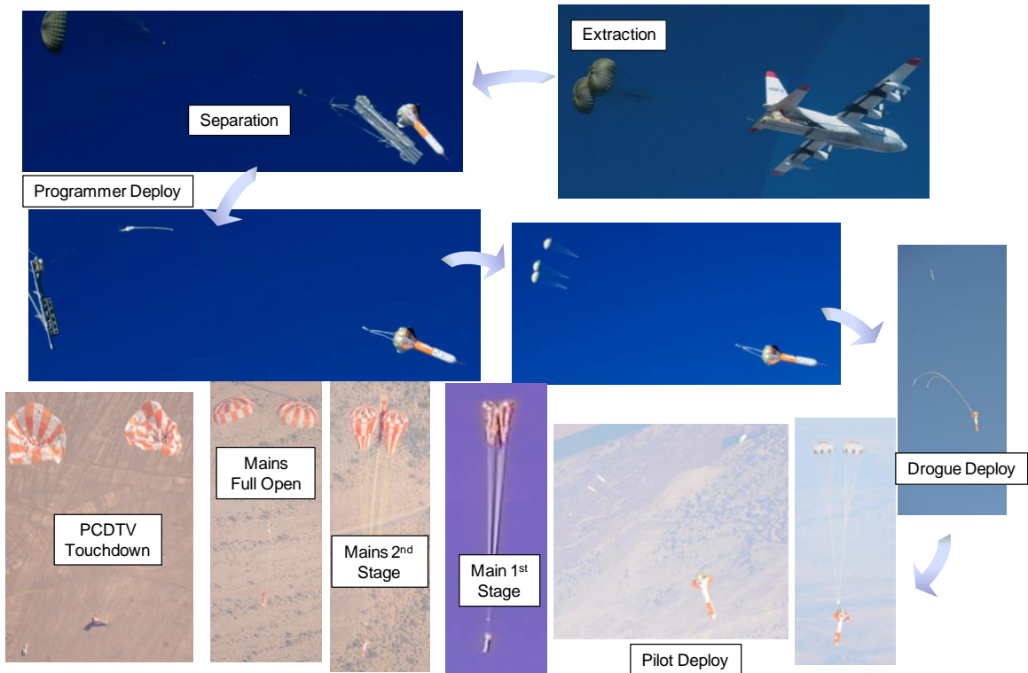
Figure 8. CDT-3-8 PCDTV concept of operations.
