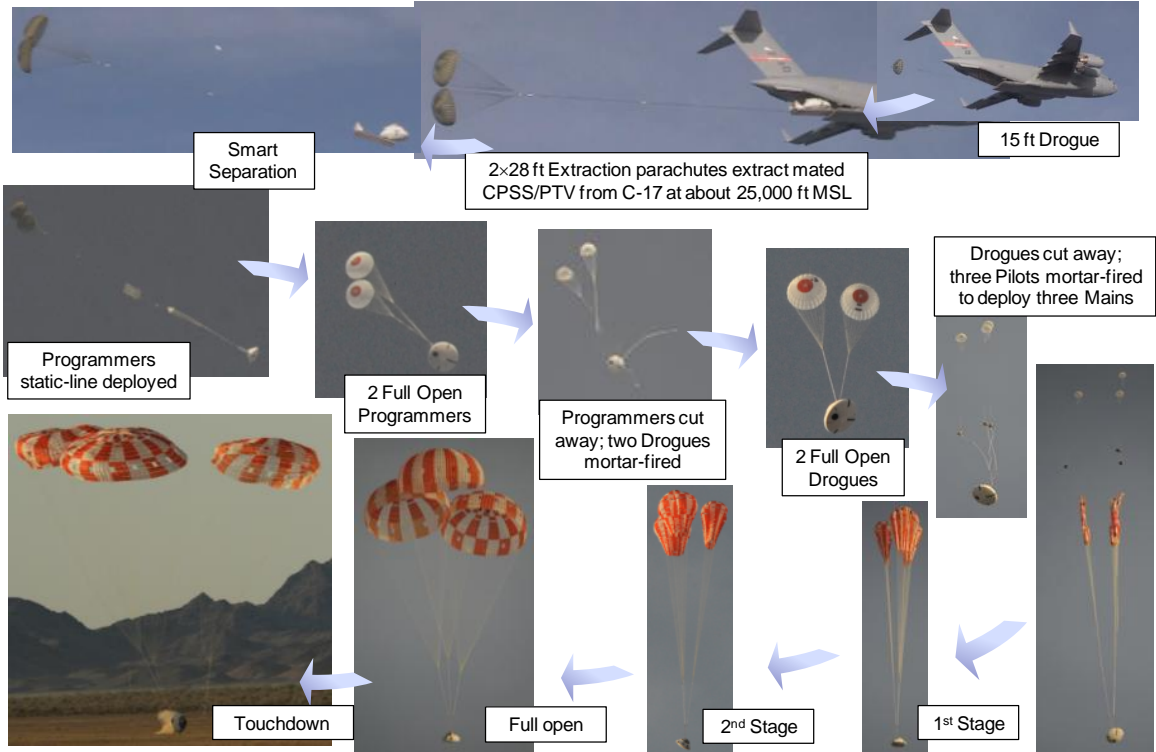
Figure 3. CDT-3-3 PTV concept of operations.
