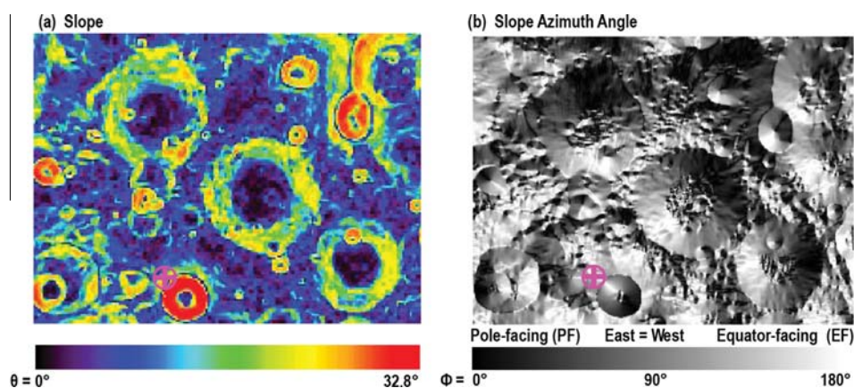
Fig. 3. Maps of south polar topographic slope and slope azimuth angle used to classify and segment the epithermal neutron, illumination and temperature maps. (a) Slope \theta is in degrees of inclination from the local horizontal plane. (b) Slope azimuth angle \phi defines the slope aspect's angular deviation in degrees from the pole-facing direction. Slope azimuth angle ranges from pole-facing \phi = 0 ( black ) to equator-facing directions \phi = 180 ( white ). The south pole is at the pink+ . Epithermal, illumination and temperature map pixels are averaged as a function of slope and slope azimuth angle.
