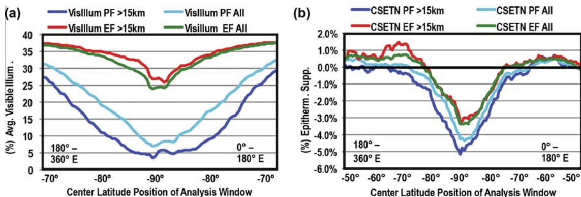
Fig. 7. Latitude profiles of the LOLA Average Visible Illumination and CSETN epithermal neutron rates for equator-facing and pole-facing slopes. Averaged equator-facing and pole-facing rates were derived within a sliding 10°-wide analysis window. (a) The available LAVI map was correlated to topography between 65°S and 90°S and (b) CSETN correlation was analyzed between 45°S and 90°S latitude. All results show the averages of both LAVI and epithermal neutron rates for all pole-facing (light blue) and equator-facing pixels (green). The average bias in hydrogen concentration of \sim 23 ppmw hydrogen is indicated by the \sim 1\% contrast in the epithermal rates on poleward and equator-facing slopes. The polar epithermal neutron flux contrast is enhanced to >2\% for Large-scale slopes, >45 ppm. The contrast enhancement is attributable to the increased signal-to-noise and detectability of Large pole-facing slopes, suggesting a widespread hydration effect.
