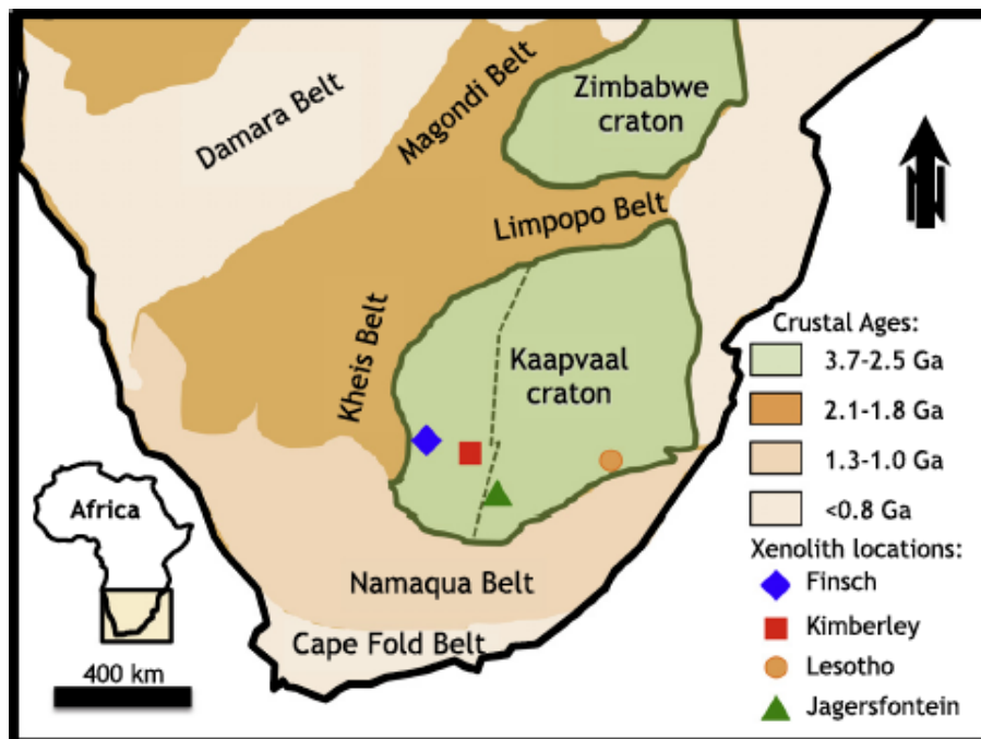
Figure 2.– Location of the Kaapvaal craton. Finsch, Kimberley, Lesotho, and Jagersfontein are diamond mines. The magma that brings up diamonds, called kimberlite, also brings up pieces of the mantle (from 100- to 200-km depth) it passes through on its way to the surface. These pieces of mantle, called xenoliths, are being analyzed for water in the present study.
