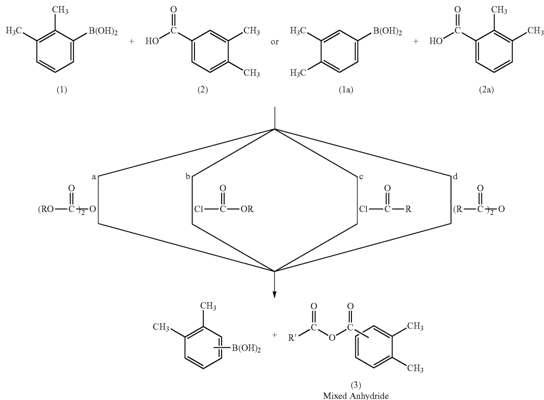
Scheme III Synthesis of a-BTDA and a-6FDA
