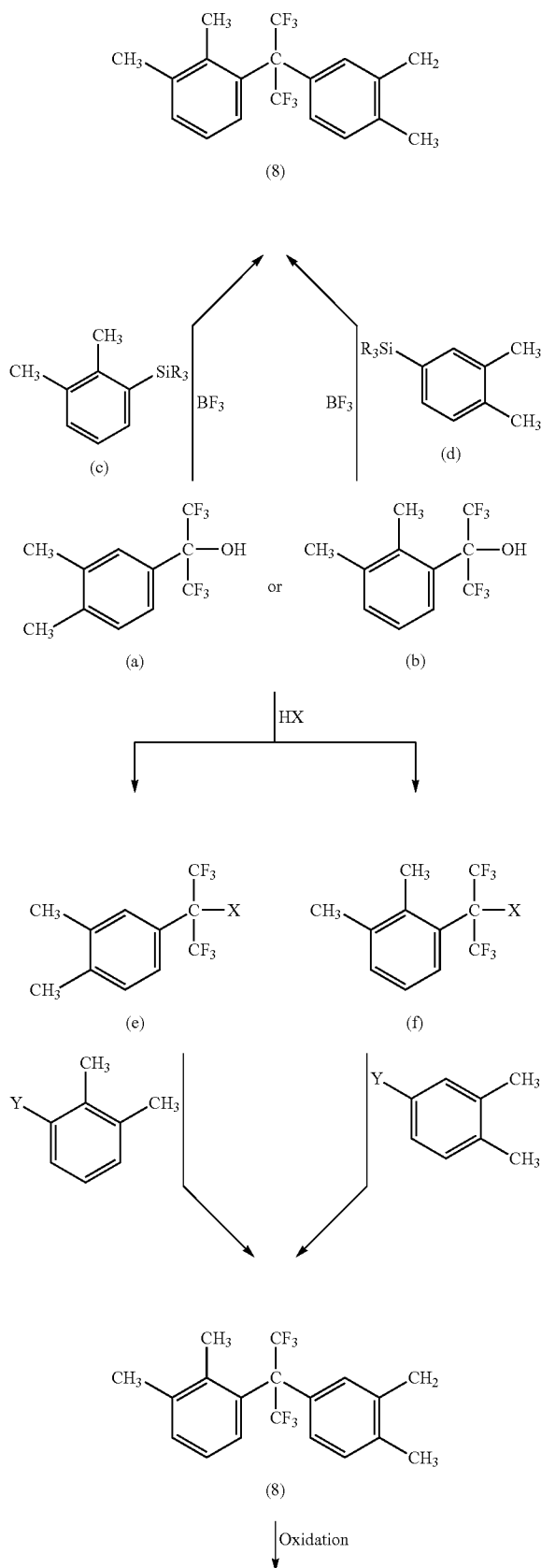
Scheme IV Alternative Synthesis of a-6FDA
