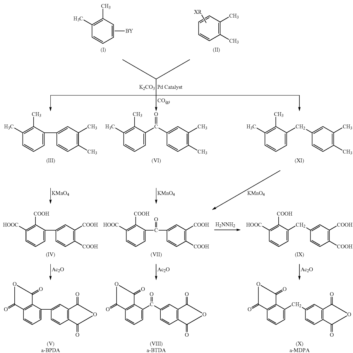
Scheme I Synthesis of Asymmetric Dianhydrides from o-xylene Derivatives
