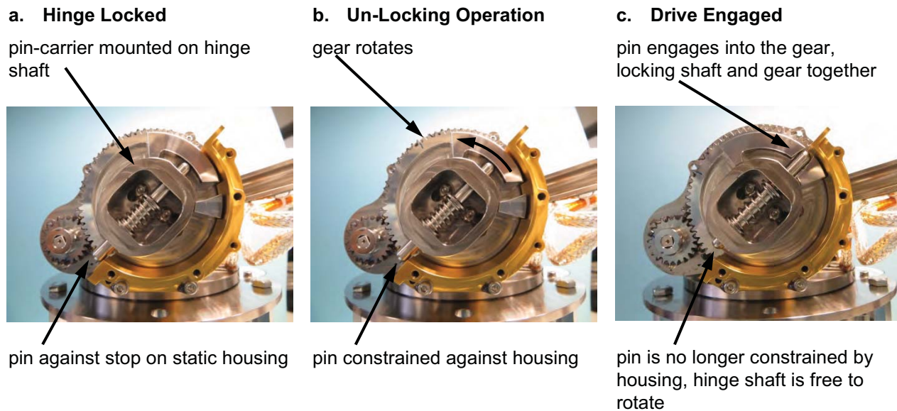
Figure 6. Solar Array Deployment Lock Operation Method
