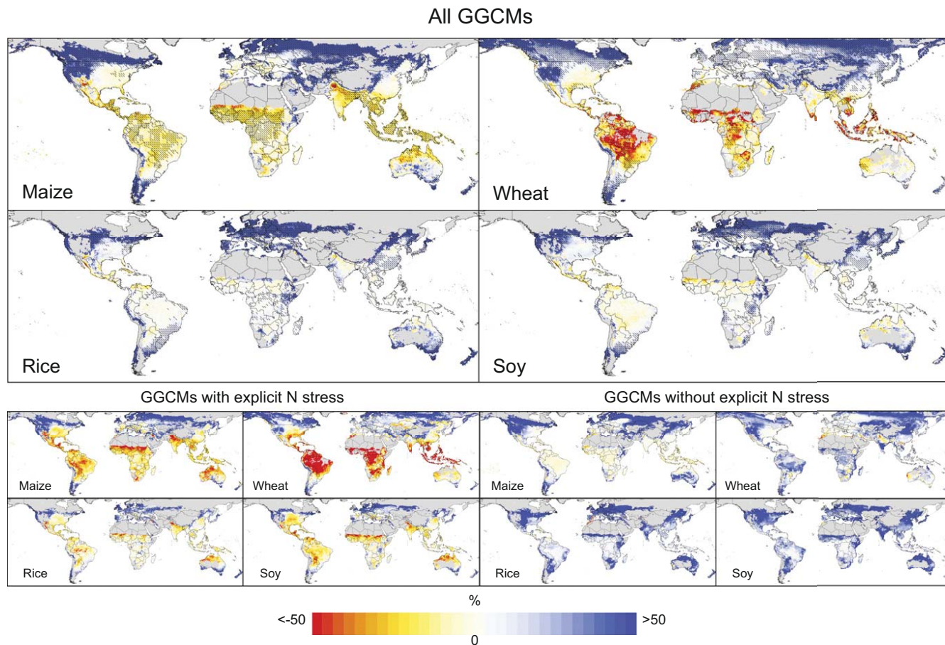
Fig. 3. Median yield changes (%) for RCP8.5 (2070–2099 in comparison to 1980–2010 baseline) with CO 2 effects over all five GCMs \times seven GGCMs (6 GGCMs for rice) for rainfed maize (35 ensemble members), wheat (35 ensemble members), rice (30 ensemble members), and soy (35 ensemble members). Hatching indicates areas where more than 70% of the ensemble members agree on the directionality of the impact factor. Gray areas indicate historical areas with little to no yield capacity. The bottom 8 panels show the corresponding yield change patterns over all five GCMs \times four GGCMs with nitrogen stress (20 ensemble members from EPIC, GEPI, pDSAT, and PEGASUS; except for rice which has 15) ( Left ); and 3 GGCMs without nitrogen stress (15 ensemble members from GAEZ-IMAGE, LPJ-GUESS, and LPJmL).
