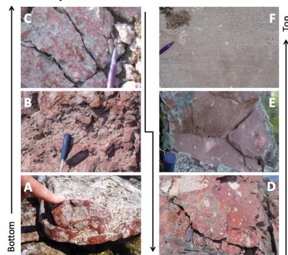
Fig. 2. Stratigraphy of impactites at the West Clearwater Lake impact structure. A) Fractured basement; B) Monomict lithic breccia; C) Impact melt-bearing lithic breccia; D) Clast-rich fine-grained impact melt rock; E) Clast-
