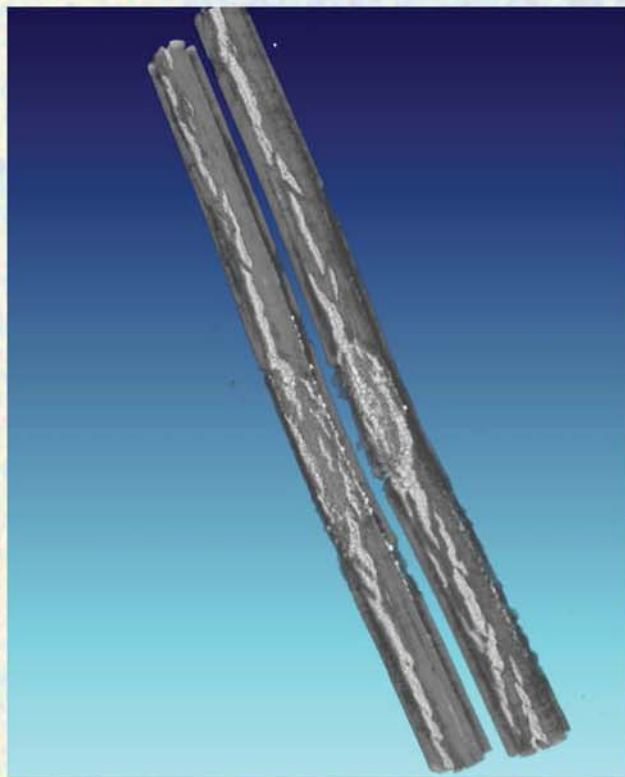
VHP overload sample post-healing (SMA reinforcements)
