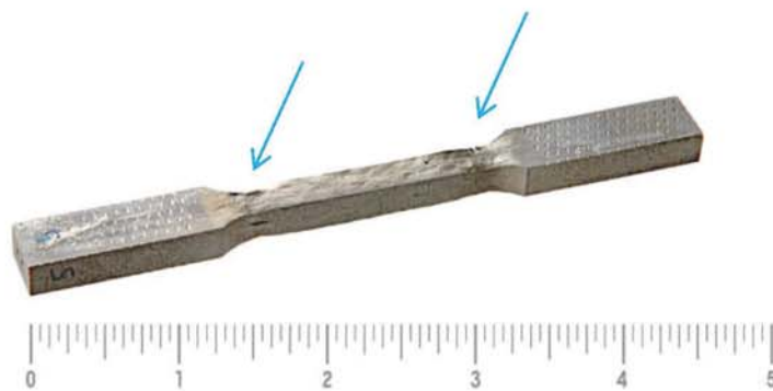
VHP overload sample pre-healing
