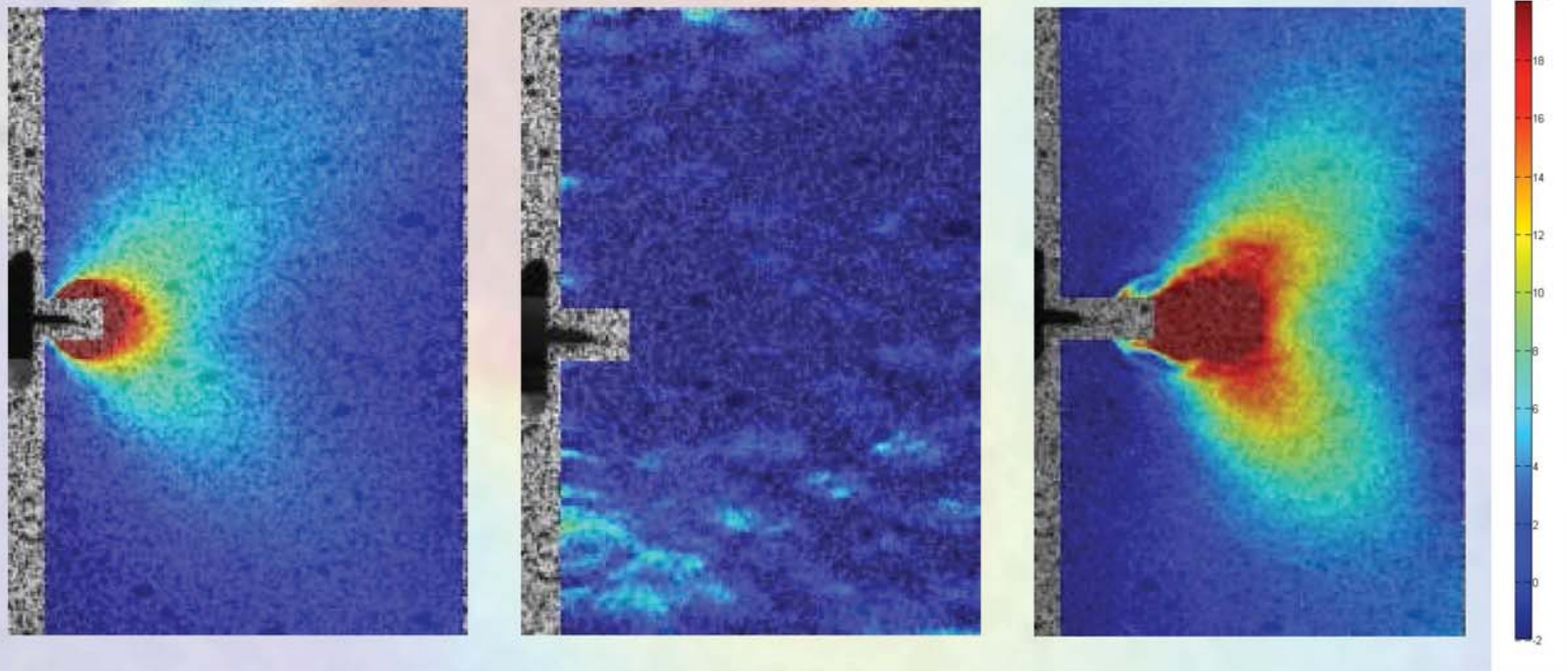
VIC strain field data of ESE(T) FCG specimen pre- and post-healing treatment.
