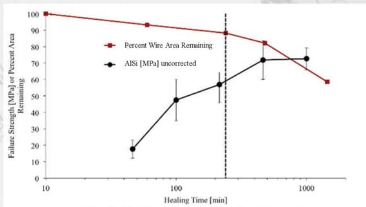
Optimization of healing treatment
