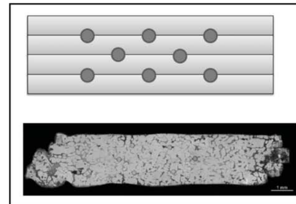
Small-scale multi-ply Al-Cu-Si specimen
