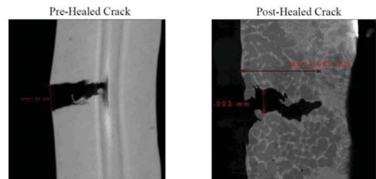
VHP overload sample pre- and post-healing
