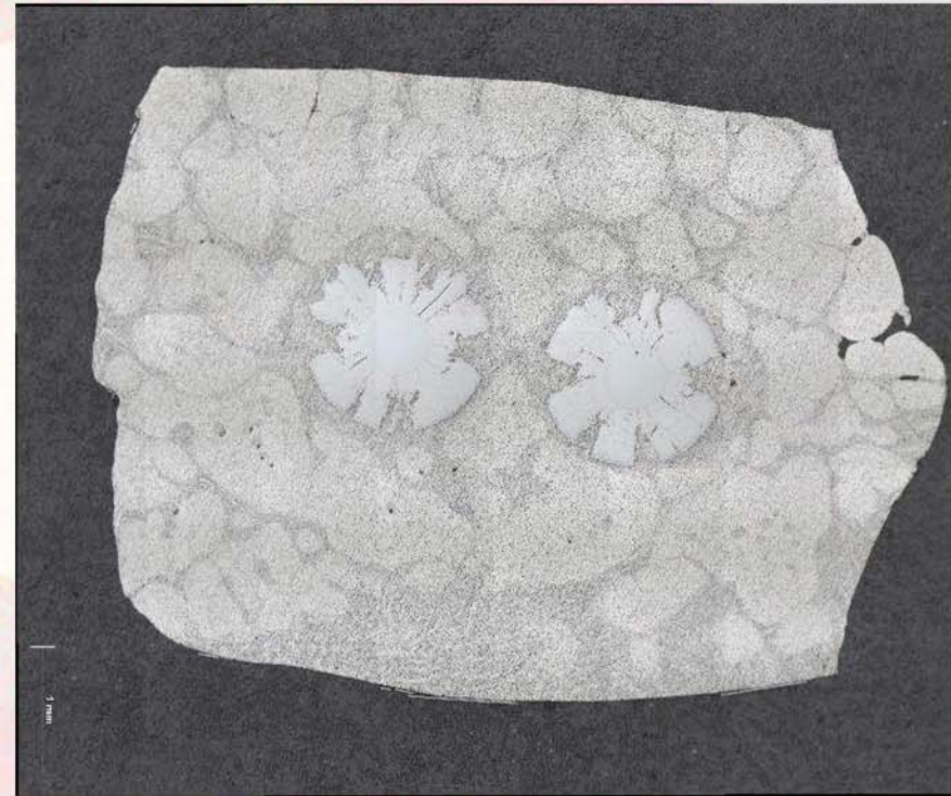
Metallographic specimen of VHP overload sample post-healing
