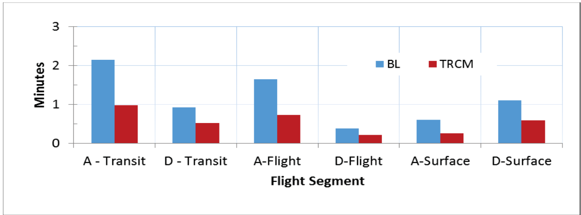
Figure 17. Day-to-day standard deviations at JFK
