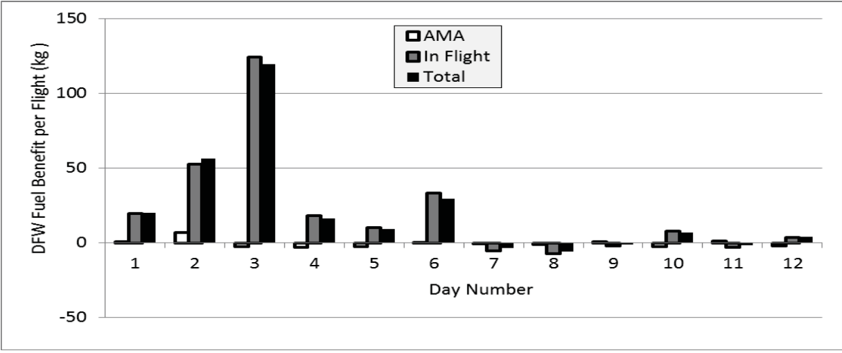
Figure 25. Fuel use benefit per flight for in-flight and AMA segments, and total
