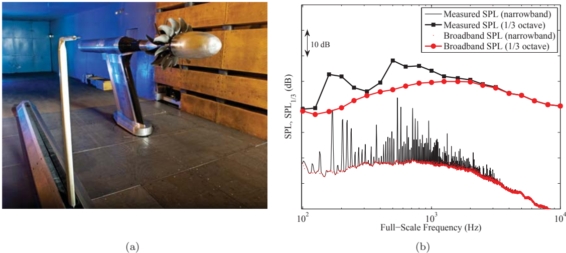
Figure 1. Illustration of broadband contribution to total noise measured from a scaled CROR model equipped with F31/A31 historical baseline blade set: (a) image of experimental CROR wind tunnel setup, (b) acoustic spectrum taken in-line with aft rotor pitch change axis for the case of \Omega_1 = \Omega_2 = 6436 RPM. More details of this testing condition provided in Table 1.
