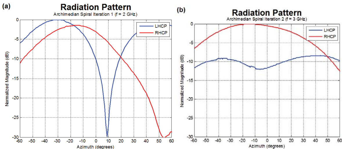
Fig. 5. Experimental and simulated (a) radiation pattern Archimedean spiral antenna v1 at a frequency of 2.0 GHz. The (b) radiation pattern of the Archimedean spiral with an embedded back reflecting plane is shown at a frequency of 3.0 GHz.
