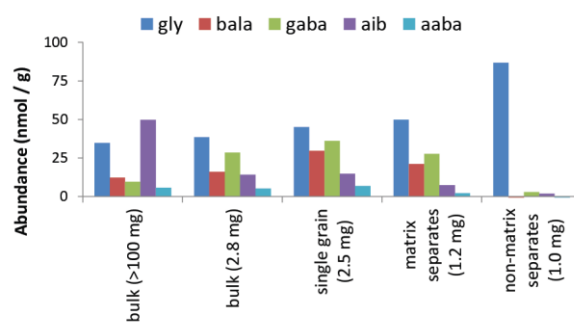
Figure 2. Comparison of selected amino acid abundances in samples from the Murchison meteorite. Amino acid abbreviations are: gly = glycine, bala = \beta -alanine; gaba = \gamma -amino-n-butyric acid, aib = \alpha -aminoisobutyric acid, aaba = \alpha -amino-n-butyric acid.
