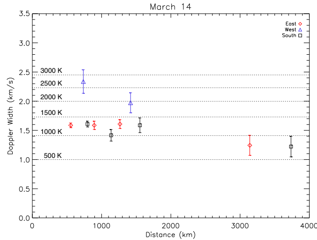
Figure 6. On 14 March 2009, Doppler width as a function of distance off the limb of the Moon (lunar phase angle \sim 41^\circ ). Observations off the west terminator intersect the Moon's shadow; Doppler widths measured in the west below 1800 km are broader than their counterparts in the east and south. Horizontal lines of constant temperature in steps of 500 K are included for comparison.
