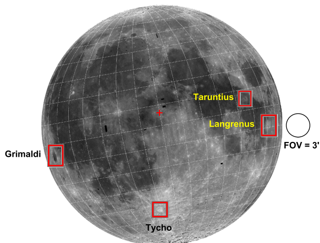
Figure 1. Observations were made in right ascension (east and west) and declination (south) out to two lunar radii above the lunar limb. Craters Grimaldi (68.3°W, 5.5°S), Tarantius (46.5°E, 5.6°N), Langrenus (61.1°E, 8.9°S), and Tycho (11.1°W, 43.4°S) were used as absolute reference points. The lunar highlands region near 0°W, 5°N was used as our “Moon center” (indicated by the cross sign in the figure). (Moon image credit: M. Robinson, Northwestern University).
