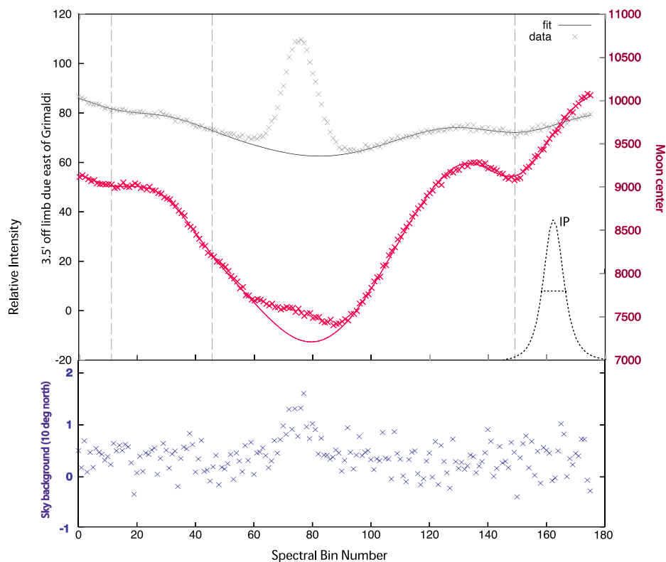
Figure 4. Sample Na spectra 3.5 arc min off the east limb (gray) and centered on the Moon (red); a sky background scan 10° north of the Moon (blue) is also included for comparison. Fits to the lunar data (solid lines) include three terrestrial H 2 O lines at 5889.637, 5890.090, and 5890.227 Å (indicated by vertical dashed lines in the figure), two components for the Na emission (5889.9386 and 5889.9584 Å S-resolved hyperfine fine structure components in a 3:5 ratio), and a solar Na Fraunhofer feature at 5889.9509 Å. Note that Na emission is detected against the sunlit lunar surface (red). Integration times were 300 s for the east limb and sky background spectra; the Moon-centered spectrum was obtained in 60 s. The abscissa is in spectral bin number where 1 bin = 0.2144 km/s; red wavelengths are to the left. At a wavelength of 5890 Å the 180 bins pictured above correspond to a spectral interval of 0.76 Å (0.00421 Å per bin). A representative instrumental profile, located near spectral bin 160, is included for comparison (full width at half maximum (FWHM) ~1.7 km/s).
