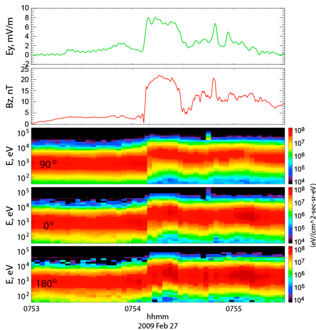
Figure 6. Color-coded parallel and perpendicular differential electron energy fluxes (in \text{eV}/\text{s}/\text{cm}^2/\text{sr}/\text{eV} ) as functions of time and energy obtained by THD at x \approx -11 R_E . The first panel shows the electric field component E_y , and the second panel the magnetic field component B_z .
