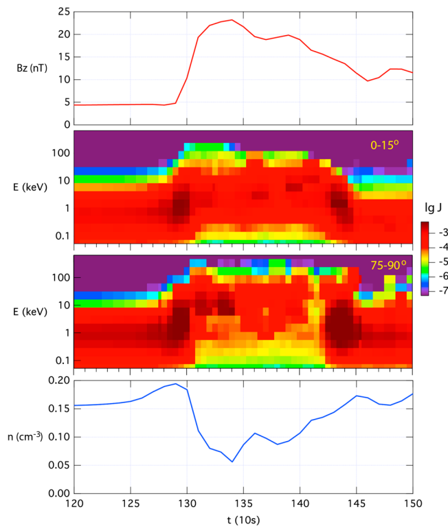
Figure 5. Simulated parallel and perpendicular electron fluxes as functions of time and energy at x = -10.5, y = 0, z = 0 . (top) The magnetic field B_z and (bottom) the plasma density n at this location.
