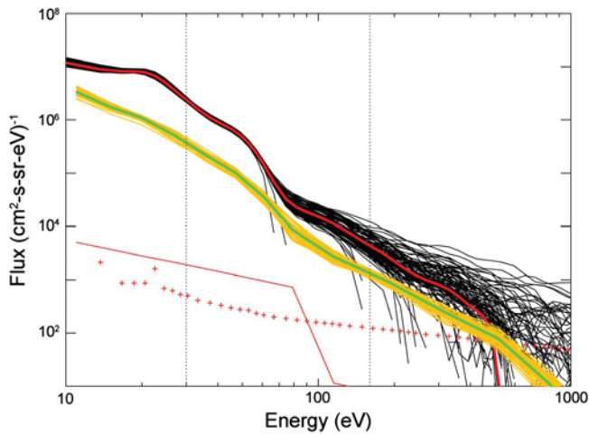
Figure 9. Photoelectron spectra acquired on the FAST satellite at Earth (black) and on the MGS satellite at Mars in the pitch angle range 0–30° on 20 September 2005. The average Earth spectrum is shown in red, and the average Mars spectrum is shown in green. The red plus symbols show the 1 standard deviation uncertainty in the average Earth flux value based on the number of counts detected. The solid red line at the bottom is the instrument background of the Mars electron detector. The vertical dotted lines are at 30 and 110 eV as they are in Figure 6.
