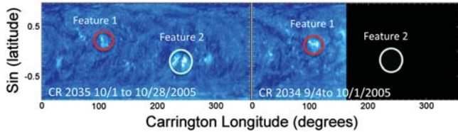
Figure 1. Data from the SOHO 17.1 nm imager for two Carrington rotations. Data are presented as a function of the sine of solar latitude and Carrington longitude. Note that in this format time goes from right to left. SOHO data were not available before 15 September as indicated by the lack of data in Carrington rotation 2034 from longitudes 360–160.
