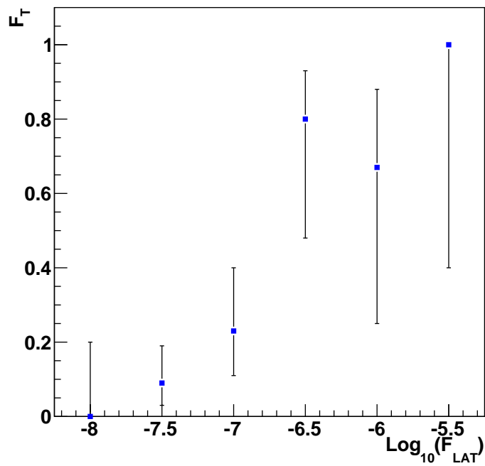
Figure 6: The fraction F_T (see text) of Fermi-LAT pulsars seen by Milagro as a function of half-decade bins of the integrated Fermi-LAT flux ( photons \text{cm}^{-2}\text{s}^{-1} ) in the energy range from 100 MeV to 100 GeV.
