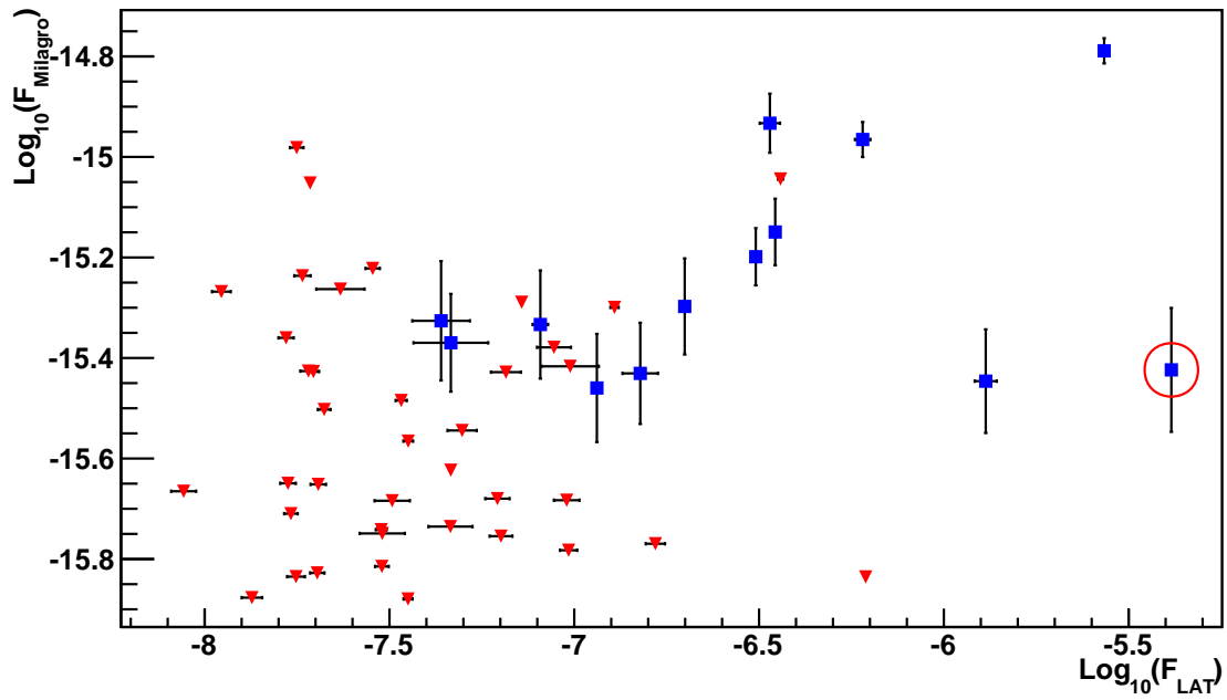
Figure 5: The horizontal axis is the Fermi-LAT flux ( \text{photons s}^{-1}\text{cm}^{-2} ), integrated over the energy range from 100 MeV to 100 GeV. The vertical axis is the Milagro flux derived at 35 TeV ( \text{photons TeV}^{-1}\text{s}^{-1}\text{cm}^{-2} ), assuming all targets are point sources. Red data points are Milagro upper limits of candidates that failed the \lambda = 0.01 FDR cut. Blue data points are the Milagro flux derived for the candidates that passed the \lambda = 0.01 FDR cut. The Milagro flux/flux limits used in this plot were derived assuming the targets are point sources. However, some of these objects are extended sources, for which the point source flux would underestimate the total flux. Geminga is a specific example and it is circled in red.
