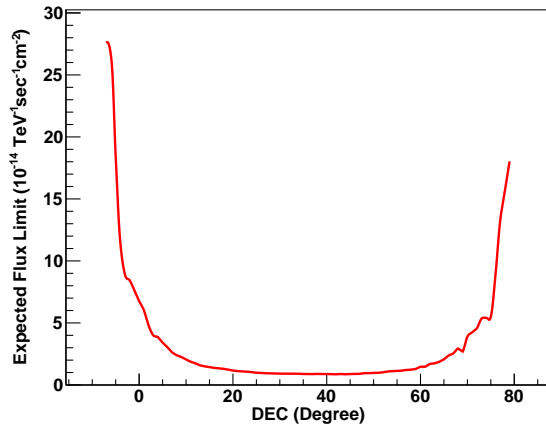
Figure 2: The expected 95% confidence level upper limit on the flux for extragalactic sources corresponding to zero excess derived at 7 TeV for each declination band of the Milagro sky maps made with spectral assumption dN/dE \propto E^{-2.0} e^{-\frac{E}{57\text{eV}}} .
