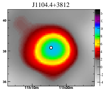
Figure 3: This map shows the 5^\circ \times 5^\circ (25 minutes \times 5 ^\circ ) region around Mkn 421. The LAT source position is marked by a white dot. This map is made with the spectral optimization dN/dE \propto E^{-2.0} e^{-\frac{E}{57\text{eV}}} and the data have been smoothed using a Gaussian function. The color of a bin shows the statistical significance (in standard deviations) of that bin. The horizontal axis is right ascension in hours and the vertical axis is declination in degrees.
