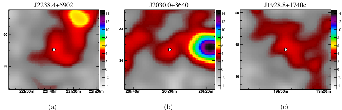
Figure 4: These maps show the 5^\circ \times 5^\circ (25 minutes \times 5^\circ ) region around 2FGL J2238.4+5902, 2FGL J2030.0+3640 and 2FGL J1928.8+1740c. The LAT source positions are marked by white dots. These maps are made with the spectral optimization dN/dE \propto E^{-2.6} and the data have been smoothed using a Gaussian function. The color of a bin shows the statistical significance (in standard deviations) of that bin. The horizontal axis is right ascension in hours and the vertical axis is declination in degrees.
