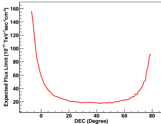
Figure 1: The expected 95% confidence level flux upper limit for Galactic sources corresponding to zero excess derived at 35 TeV for each declination band of the Milagro sky maps made with spectral assumption dN/dE \propto E^{-2.6} .
