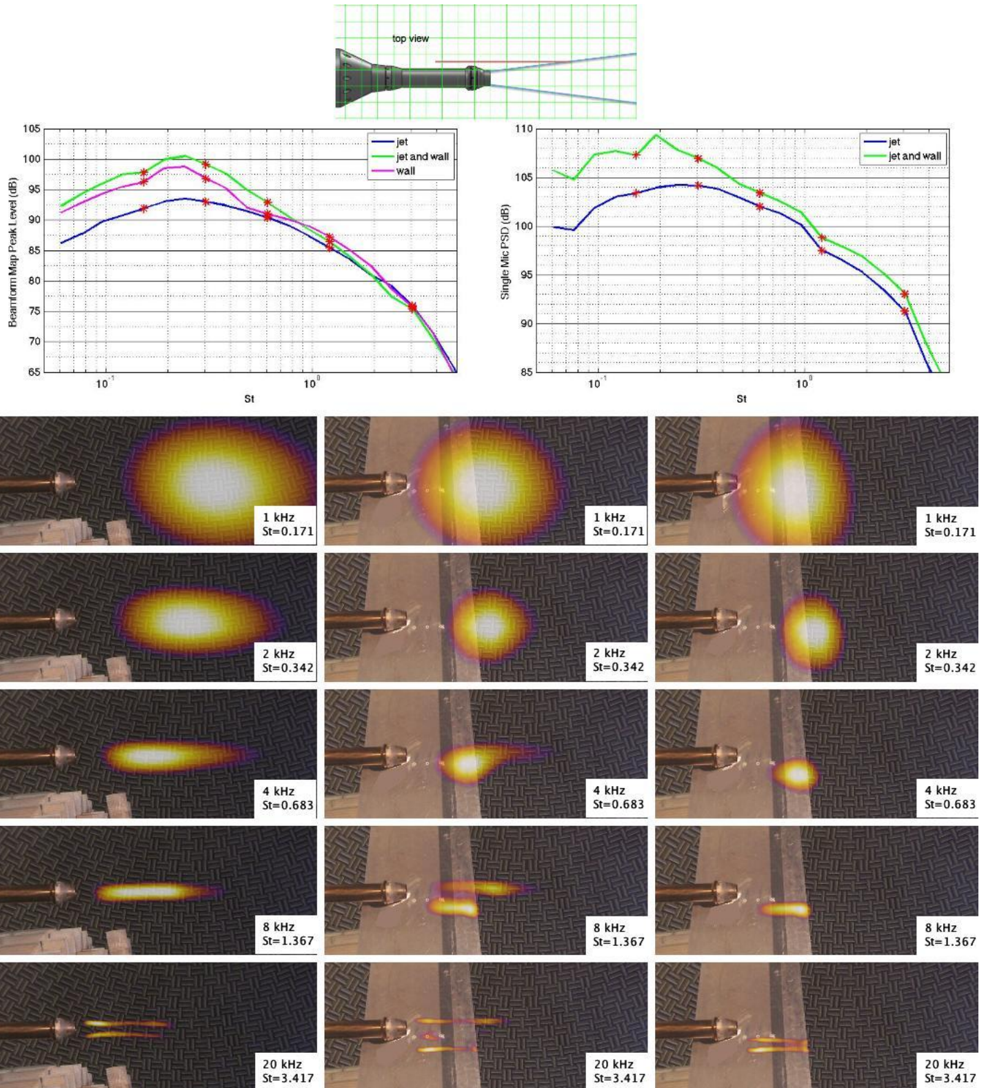
Figure 23. Beamform map peak spectra (upper left), single mic spectra (upper right) and beamform maps (bottom) for the bare jet and the 5D reflecting surface located 1D from the jet centerline for the SMC000 nozzle at setpoint 7. The beamform maps are bare jet (left column), jet/surface combination (center), and surface alone (right).
