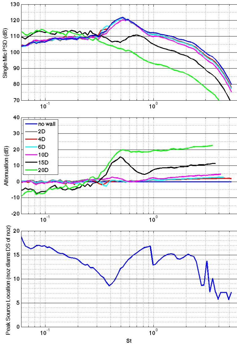
Figure 20. Single mic spectra (upper left), attenuation plots (center left), peak location plot (lower left) and beamform maps (right) for the bare jet and surfaces extending 2, 4, 6, 10, 15, and 20D downstream of nozzle and 3D away from jet centerline for the SMC016 CD nozzle at the under-expanded setpoint (11617, M_j=1.61 , TSR=0.76 ).
