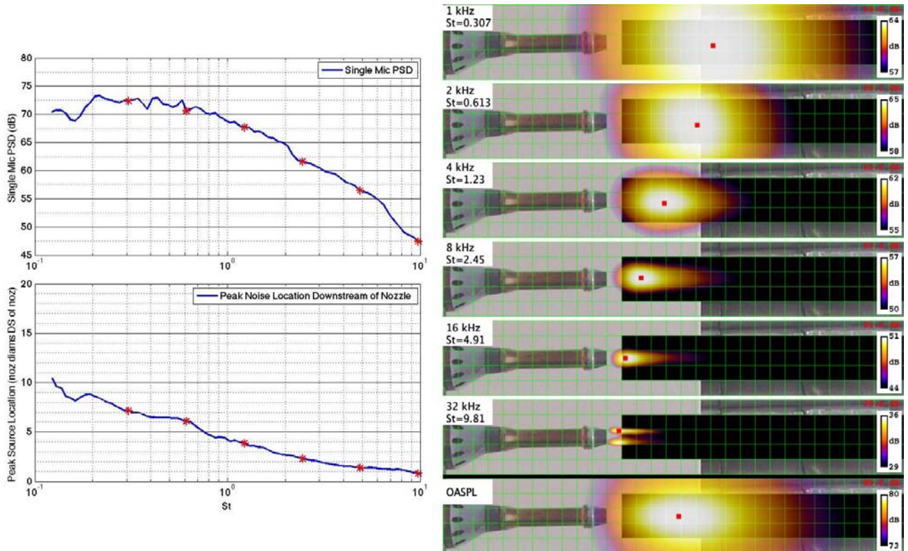
Figure 7. Single microphone spectra (upper left), peak location plot (lower left), 1/12 th OB beamform maps (right), and OASPL beamform map (lower right) for the SMC000 RC nozzle operating at setpoint 3 ( M_a=0.50 , TSR=0.95 )
