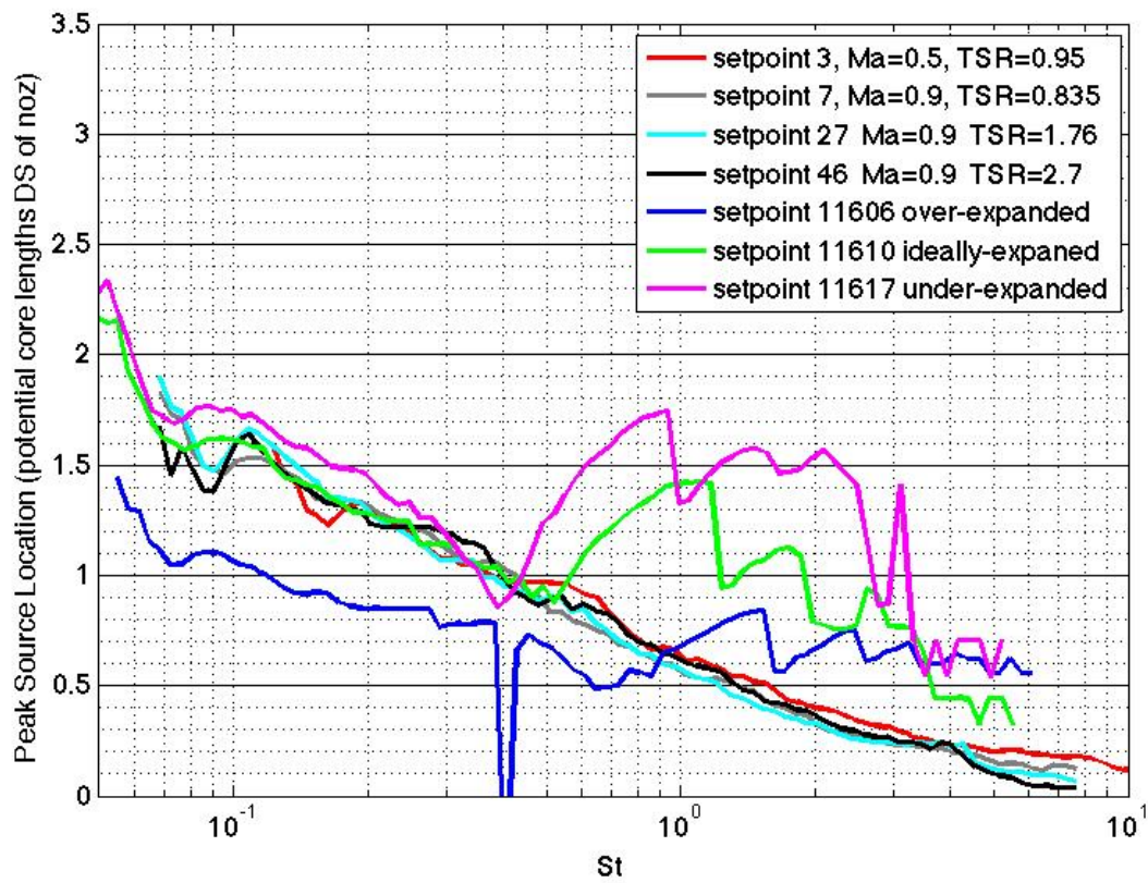
Figure 13. Nondimensional peak noise source location plotted versus nondimensional frequency for each of the seven tested setpoints.
