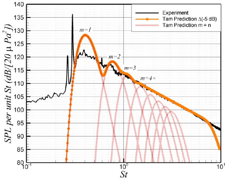
Figure 11. BBSN spectral humps predicted using Tam's model compared with experimental data. (figure taken from Miller, ref 10)
