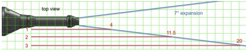
Figure 14. Schematic showing jet/surface intersection points for surfaces 1, 2, and 3 jet diameters from the jet centerline and a jet assumed to expand at a 7° angle.
