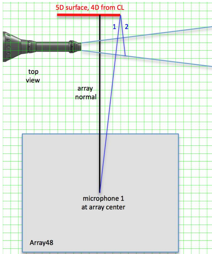
Figure 21. Schematic of a reflecting surface configuration test illustrating the law of reflection.
