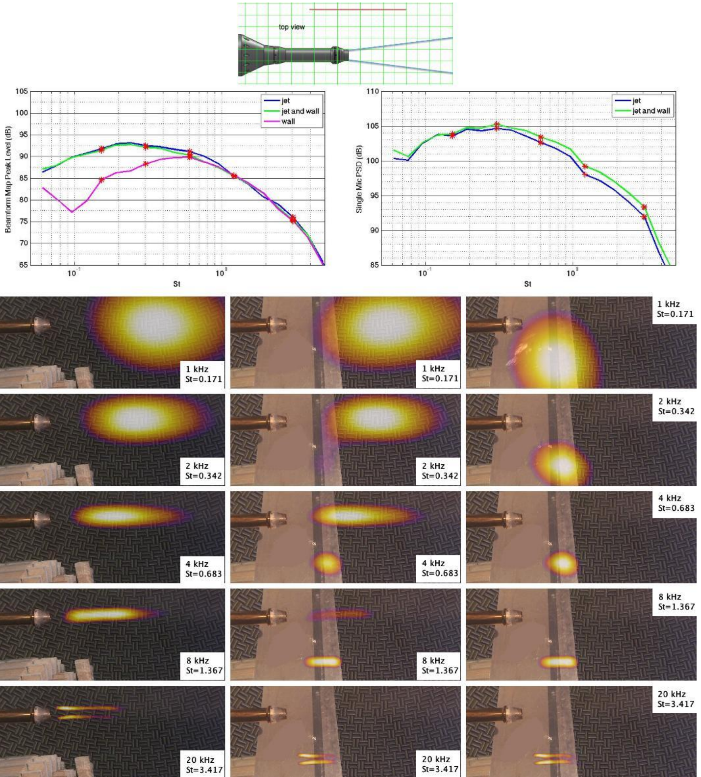
Figure 22. Beamform map peak spectra (upper left), single mic spectra (upper right) and beamform maps (bottom) for the bare jet and the 5D reflecting surface located 4D from the jet centerline for the SMC000 nozzle at setpoint 7.
