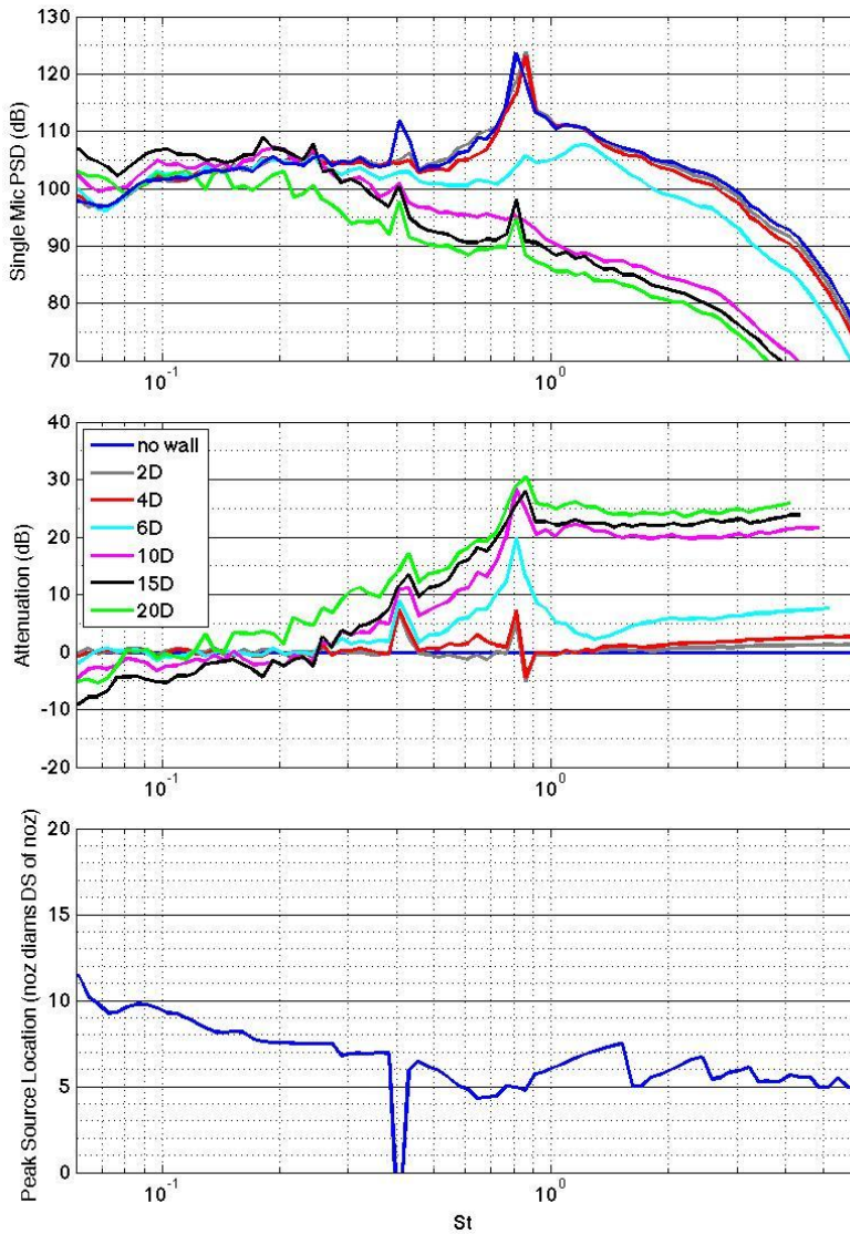
Figure 18. Single mic spectra (upper left), attenuation plots (center left), peak location plot (lower left) and beamform maps (right) for the bare jet and surfaces extending 2, 4, 6, 10, 15, and 20D downstream of nozzle and 3D away from jet centerline for the SMC016 nozzle at the over-expanded setpoint ( 11606 , M_j=1.29 , TSR=0.76 ).
