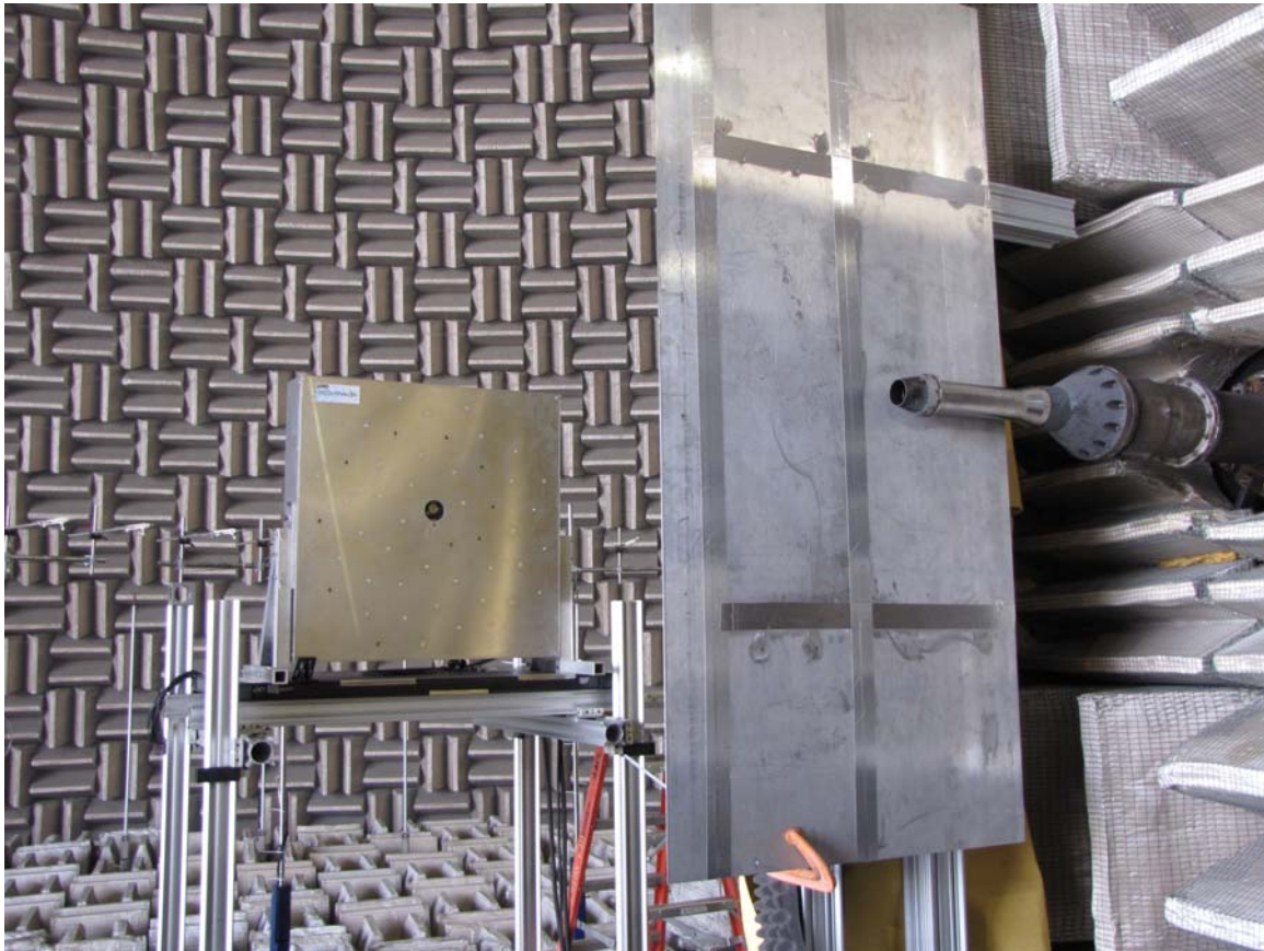
Figure 5. Photo showing the phased array during a shielding configuration test.
