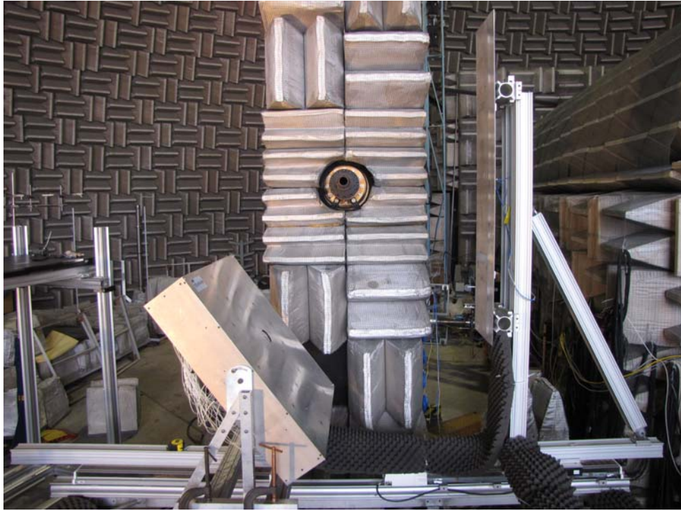
Figure 6. Photo showing the phased array mounted on the moveable cart during a reflecting configuration test.
