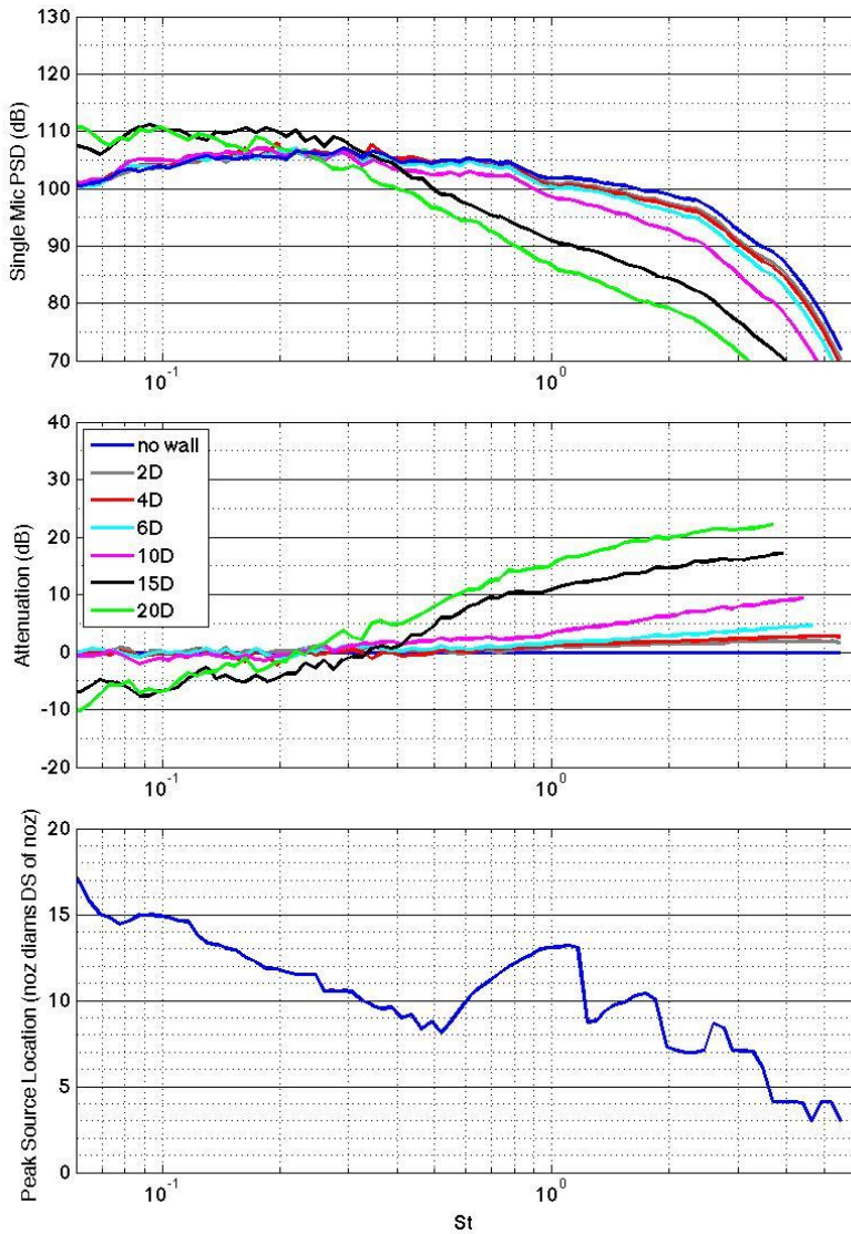
Figure 19. Single mic spectra (upper left), attenuation plots (center left), peak location plot (lower left) and beamform maps (right) for the bare jet and surfaces extending 2, 4, 6, 10, 15, and 20D downstream of nozzle and 3D away from jet centerline for the SMC016 nozzle at the ideally-expanded setpoint (11610, M_j=1.50 , TSR=0.72 ).
