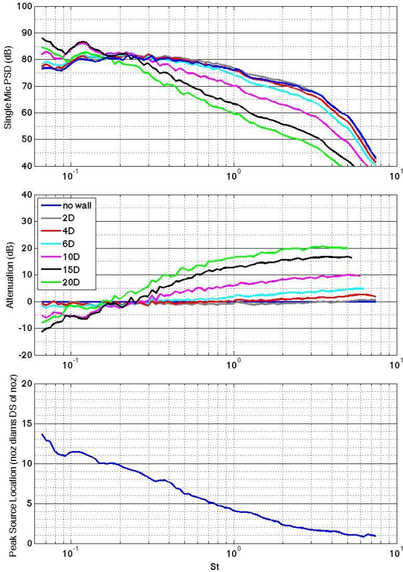
Figure 15. Single mic spectra (upper left), attenuation plots (center left), peak location plot (lower left) and beamform maps (right) for the bare jet and surfaces extending 2, 4, 6, 10, 15, and 20D downstream of nozzle and 3D away from jet centerline for the SMC000 nozzle at setpoint 7 ( M_a=0.90 , TSR=0.835 ).
