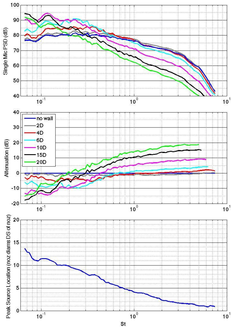
Figure 17. Single microphone spectra (upper left), attenuation plots (center left), peak location plot (lower left) and beamform maps (right) for the bare jet and surfaces extending 2, 4, 6, 10, 15, and 20D downstream of nozzle and 1D away from jet centerline for the SMC000 nozzle at setpoint 7 ( M_a=0.90 , TSR=0.835 ).
