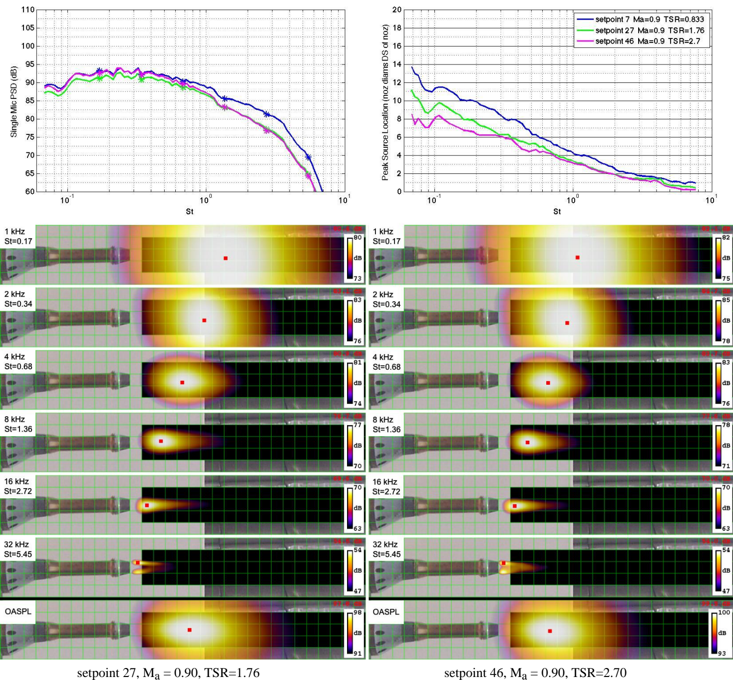
Figure 9. Single mic spectra (upper left), peak location plots (upper right), and beamform maps (bottom) for the SMC000 nozzle at setpoints 27 ( M_a=0.90 , TSR=1.76) and 46 ( M_a=0.90 , TSR=2.70).
