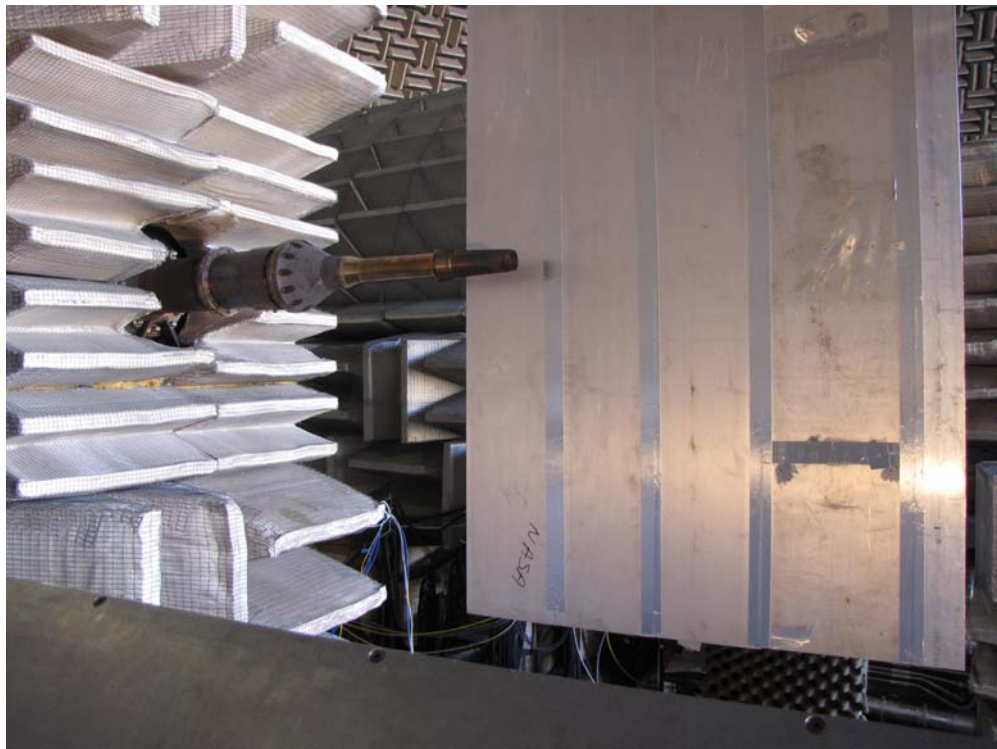
Figure 3. Photos showing example shielding (top) and reflecting (bottom) surface configurations.
