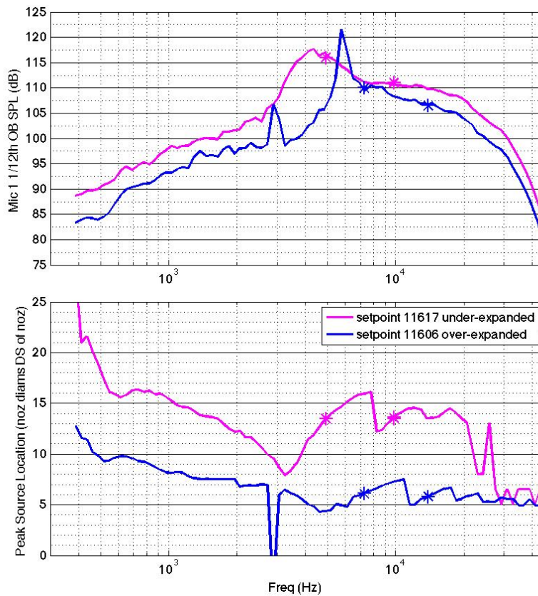
Figure 12. Peak frequencies (asterisks) corresponding to the two lowest-frequency BBSN humps predicted by Tam's model overlaid on top of spectra and peak location plots measured with SMC016 CD nozzle at setpoints 11606 ( M_j=1.29 ) and 11617 ( M_j=1.61 )
