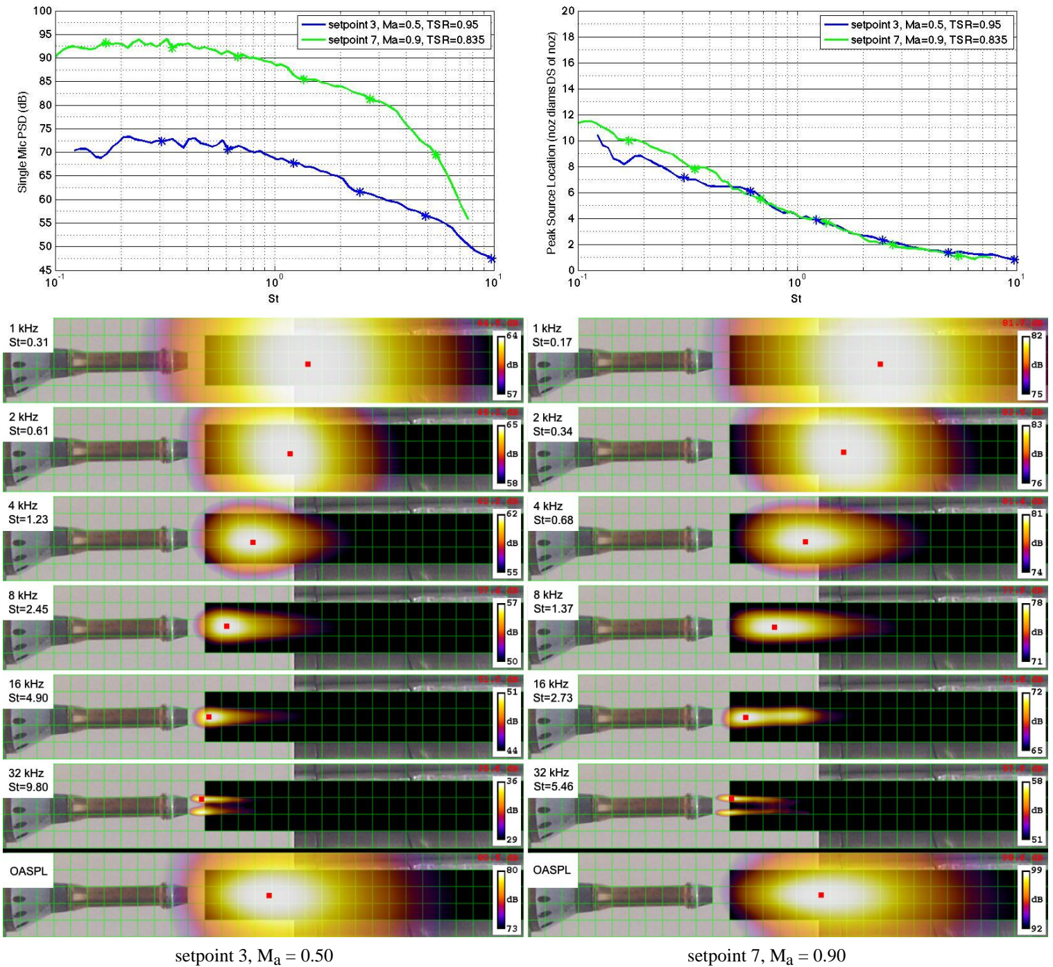
Figure 8. Single mic spectra (upper left), peak location plots (upper right), and beamform maps (bottom) for the SMC000 nozzle at setpoints 3 ( M_a=0.50 , TSR=0.95) and 7 ( M_a=0.90 , TSR=0.835).
