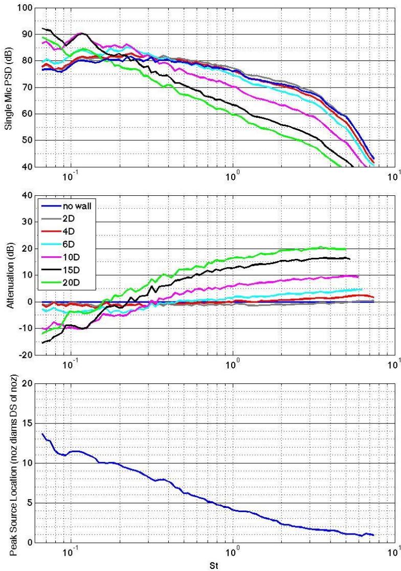
Figure 16. Single microphone spectra (upper left), attenuation plots (center left), peak location plot (lower left) and beamform maps (right) for the bare jet and surfaces extending 2, 4, 6, 10, 15, and 20D downstream of nozzle and 2D away from jet centerline for the SMC000 nozzle at setpoint 7 ( M_a=0.90 , TSR=0.835 ).
