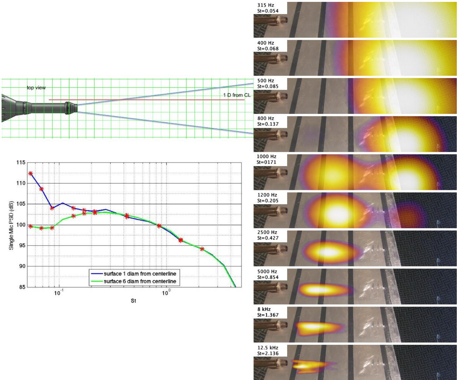
Figure 24. Single mic spectra (left) for the 20D reflecting surface located 1D (in the flow, blue) and 6D (out of the flow, green) from the jet centerline and 1/3 rd OB beamform maps (right) for the same surface located 1D (in the flow) from the jet centerline for the SMC000 nozzle at setpoint 7.
