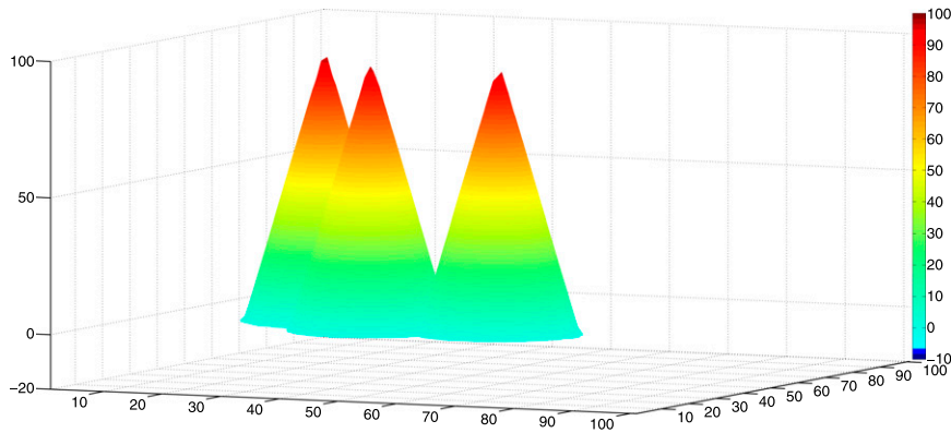
FIG. 7. Three members of the initial 50-member ensemble generated by perturbing the location of the center of the cone.
