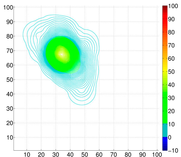
FIG. 8. The forecast ensemble mean at the first measurement time from bird's-eye perspective.
