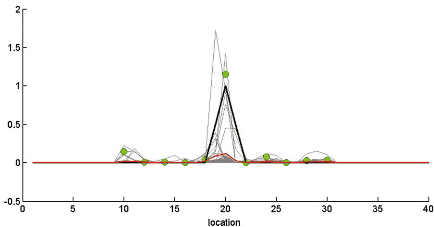
FIG. 5. 1D static analysis results for the log transformed EnKF with measurement gaps and additive log transformed measurement error variance set at the log of the additive untransformed synthetic measurement error. The true state (black), observations (green), analysis ensemble (gray), and ensemble mean (red) are shown. The analysis mean mass is 0.348 < 2 . The mass is not conserved, but the analysis mean and all analysis replicates are nonnegative. The analysis does not capture the triangular feature.
