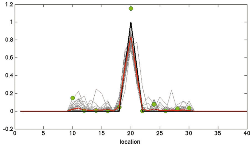
FIG. 10. 1D static analysis results for QP with positivity constraint and nominal assumed measurement error variance 0.01. True state (black), observations (green), analysis ensemble (gray), and analysis ensemble mean (red). The analysis ensemble members and their mean conserve mass and are always nonnegative. The analysis mean underestimates true at the peak in order to conserve total mass since the ensemble members and mean both include some mass in the region where the true state is zero.
