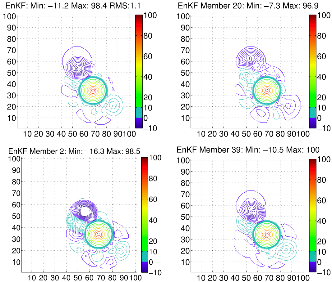
FIG. 9. (top left) The analysis at the end of the solid-body rotation experiment (time step 30241), obtained with the EnKF algorithm and 50 ensemble members. Ensemble members are shown as examples of replicates with the (top right) highest and (bottom left) lowest minimum values. (bottom right) An ensemble member with a minimum value between the two is depicted. Contour lines in the range from -10 to 10 are shown in steps of 1, and above 10 in steps of 10.
