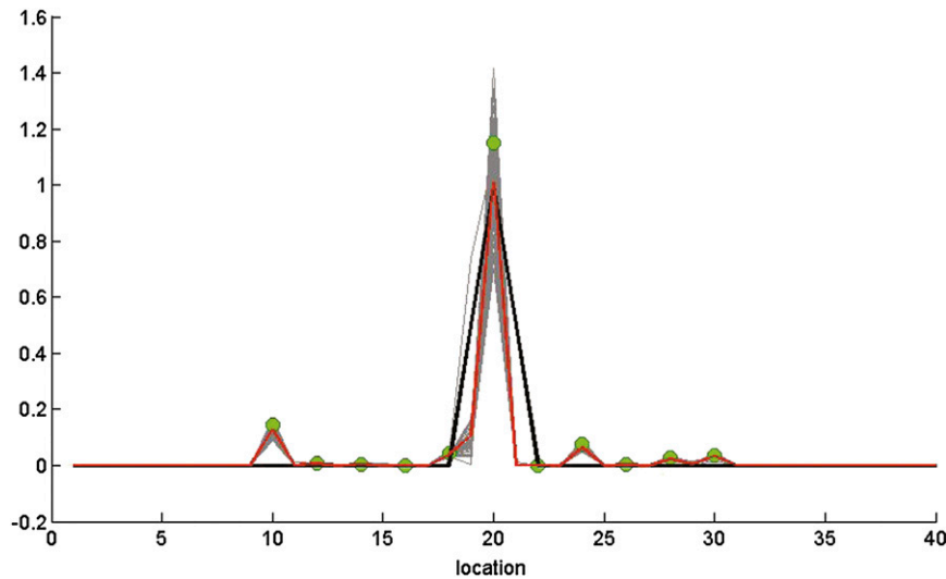
FIG. 6. 1D static analysis results for the log transformed EnKF with measurement gaps and measurement error covariance diagonal set at 0.1 variance of the log measurement error. The true state (black), observations (green), analysis ensemble (gray), and ensemble mean (red) are shown. The analysis mean mass is equal to 1.42 < 2 is not conserved, but the analysis mean and all analysis ensemble members are nonnegative. The ensemble is greatly constrained by the measurements and ensemble variability is small.
