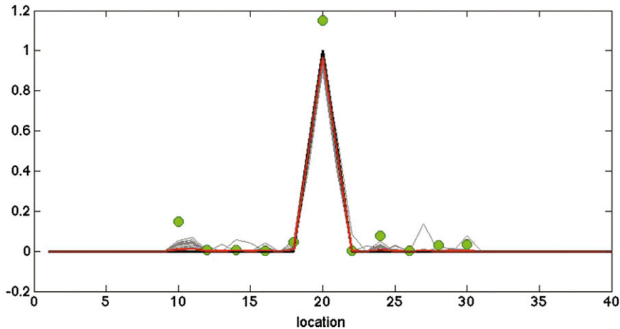
FIG. 11. 1D static analysis results for QPens with positivity constraint and lowered assumed measurement error variance (0.0025). True state (black), observations (green), analysis ensemble (gray), and analysis ensemble mean (red). The analysis ensemble and their mean conserve mass and are always nonnegative. The analysis mean and ensemble members are very close to the true values.
