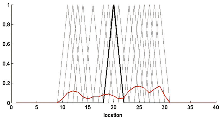
FIG. 1. 1D static forecast/prior. The true state (black), forecast/prior mean (red), and forecast/prior ensemble (gray) are shown. Mass of true, forecast mean, and each forecast ensemble member is equal to 2.
