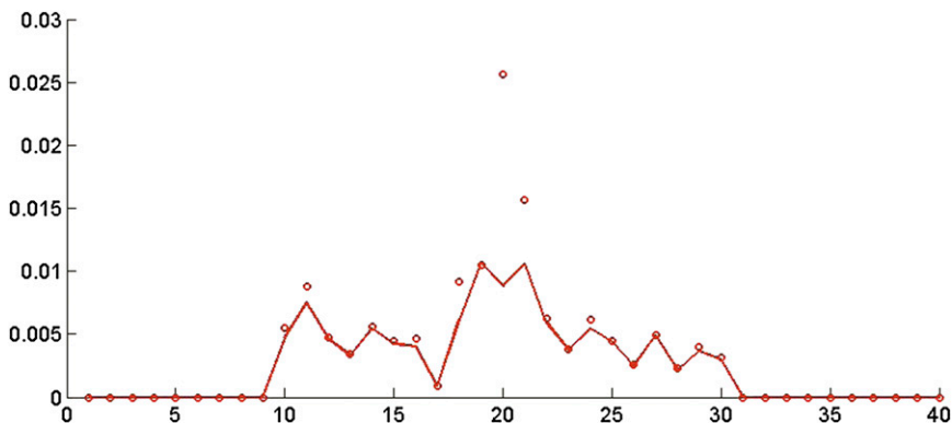
FIG. 12. 1D static analysis results for the QPens with positivity constraint and nominal measurement error variance. Comparison of ensemble standard deviation (solid) and RMSE between analysis ensemble members and true (circles). The QPens variances are generally comparable to the RMSE, with some underestimation at a few locations near the true peak. RMSE values for the QPens are significantly lower than for the EnKF (cf. Fig. 4).
