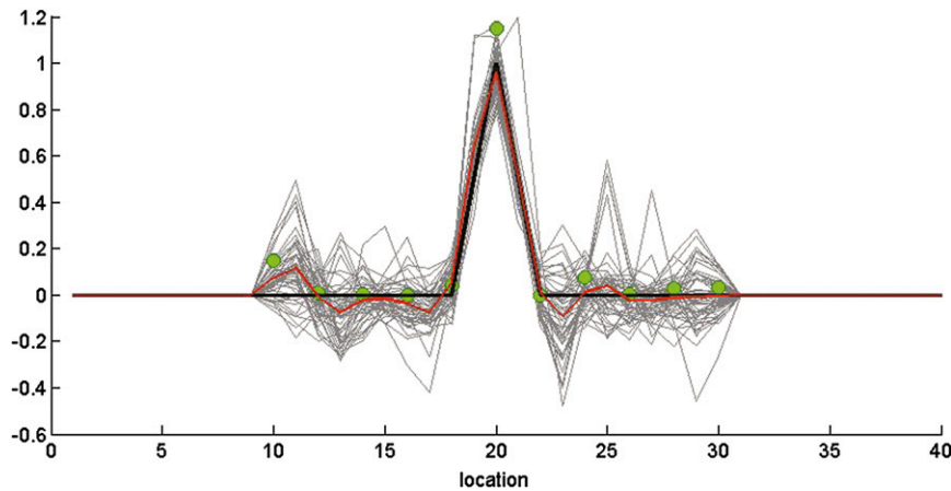
FIG. 2. 1D static analysis results for the EnKF with measurement gaps. The true state (black), observations (green), analysis ensemble (gray), and ensemble mean (red) are shown. Mass is conserved by all analysis ensemble members and analysis mean, but there are significant negative anomalies.
