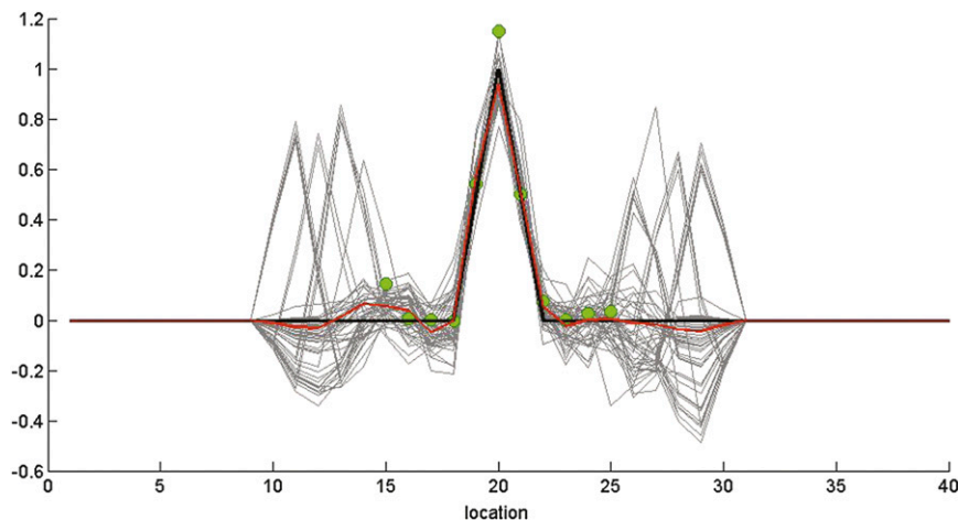
FIG. 3. 1D static analysis results for the EnKF with clustered measurements. The true state (black), observations (green), analysis ensemble (gray), and ensemble mean (red) are shown. Mass is conserved by all analysis ensemble members and the analysis mean, but there are significant negative anomalies.
