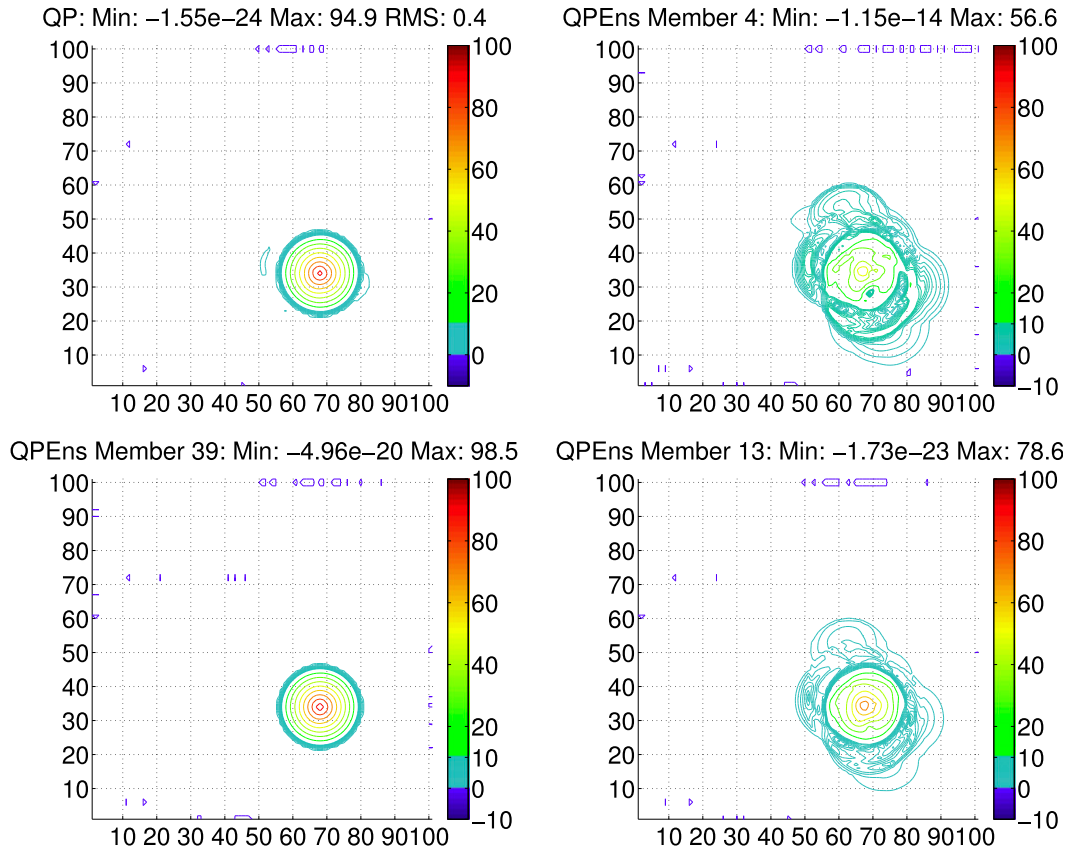
FIG. 13. (top left) The analysis at the end of the solid-body rotation experiment (time step 30241), obtained with the QPEns algorithm. Ensemble members are shown as examples of replicates with the (top right) lowest and (bottom left) highest maximum values. (bottom right) An ensemble member with maximum value between the two is depicted. Contour lines in the range from -10 to 10 are shown in steps of 1 , and above 10 in steps of 10 .
