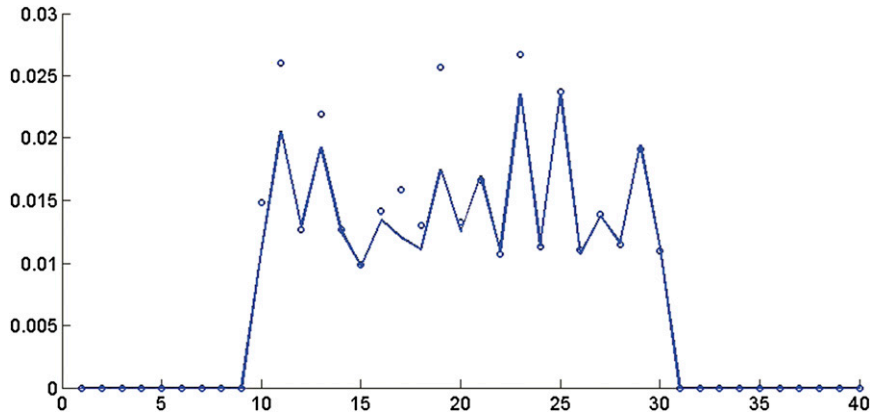
FIG. 4. 1D static analysis results for the EnKF with measurement gaps. Comparison of ensemble standard deviation (solid) and RMSE between analysis ensemble members and true (circles). The EnKF variances are generally comparable to the RMSE, with some underestimation at scattered locations.
