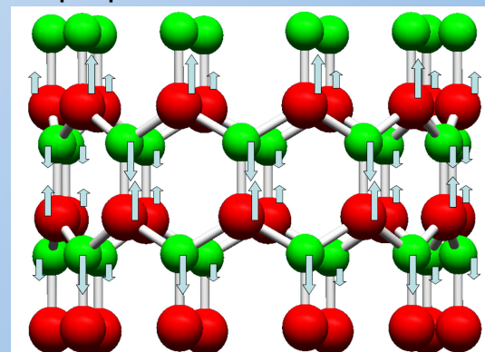
B-N stretching vibration mode perpendicular to the c-axis
