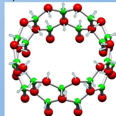
B-N-B bending vibration mode parallel to the c-axis
