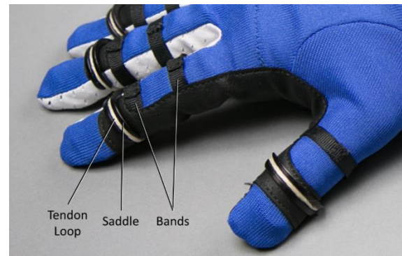
Fig. 3. Finger Detail
