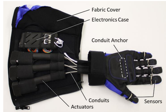
Fig. 2. Forearm Layout, Conduit Anchor, and Sensors
