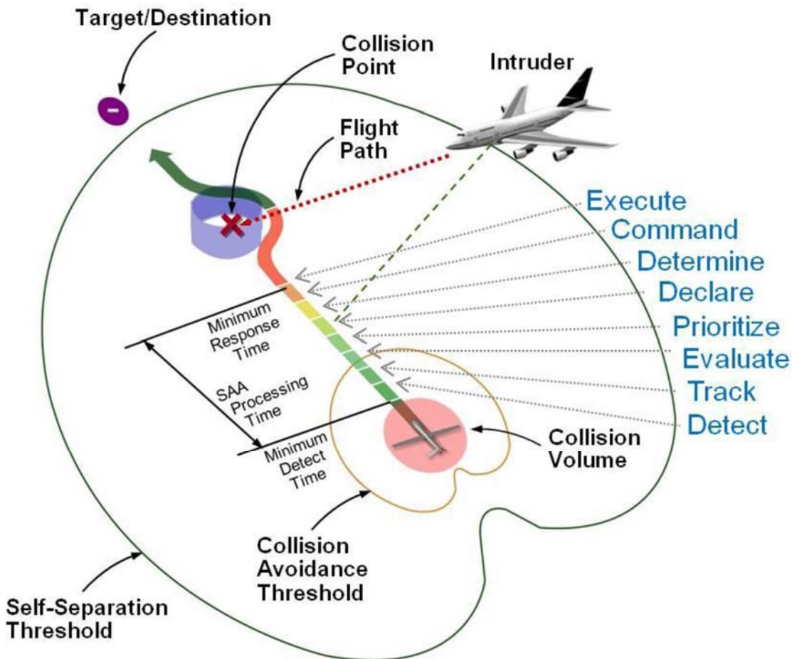
Figure 1. DAA Sub-Functions, Thresholds and Volumes
