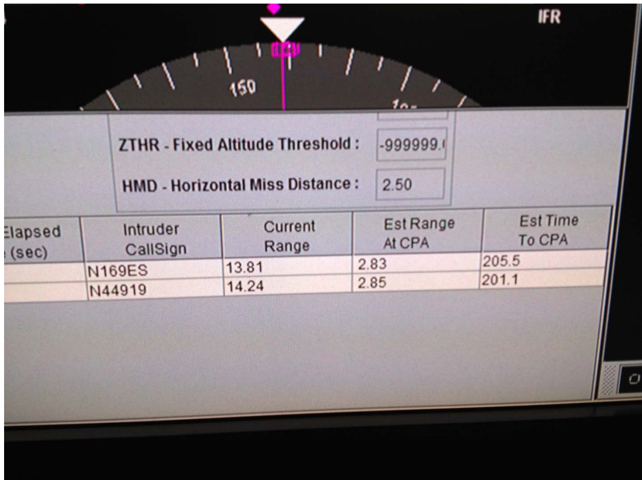
Figure 4. CAS-1 UAS GCS Display of Nearby Converging Intruders
