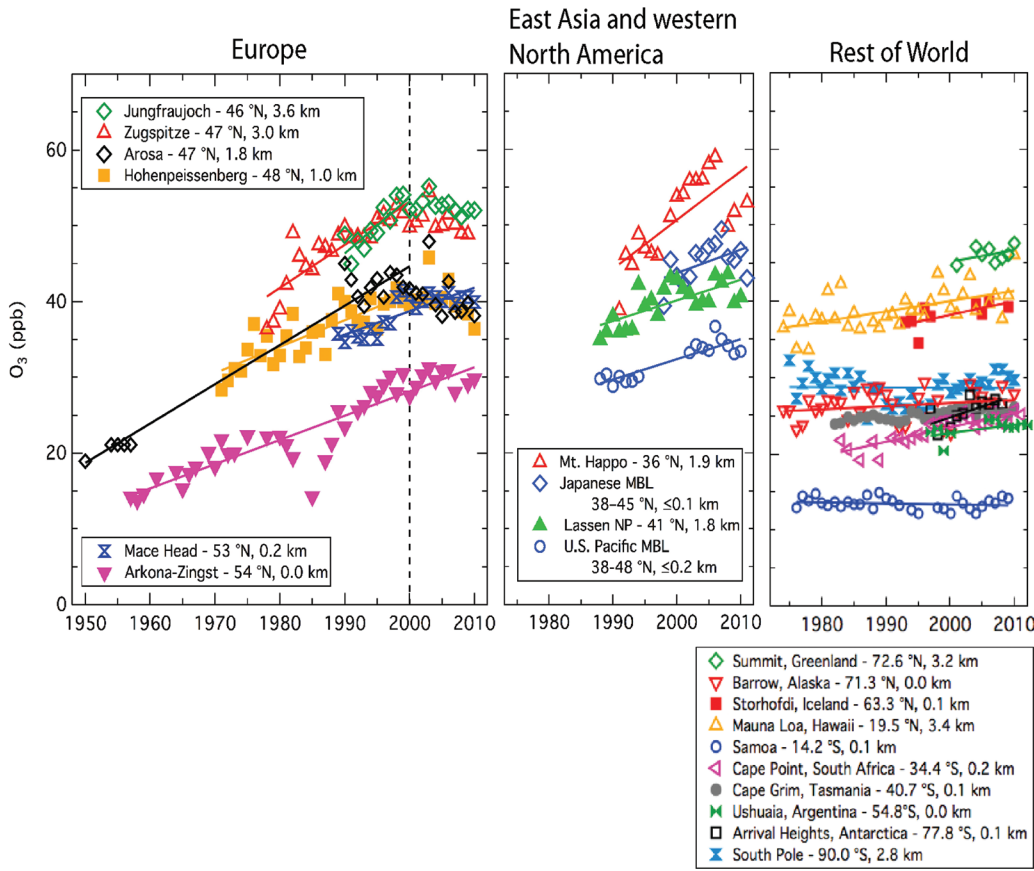
Figure 1 Surface ozone time series at several rural sites around the world.
