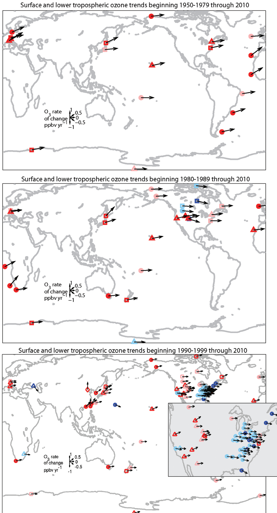
Figure 2 Global surface and lower tropospheric ozone trends.
