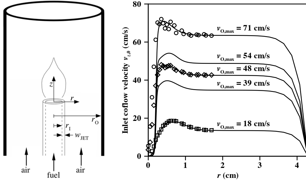
Figure 1: Left: Schematic of the burner used in the simulations. Right: Measured (symbols) and fitted (line) velocity profiles of the coflow air.
