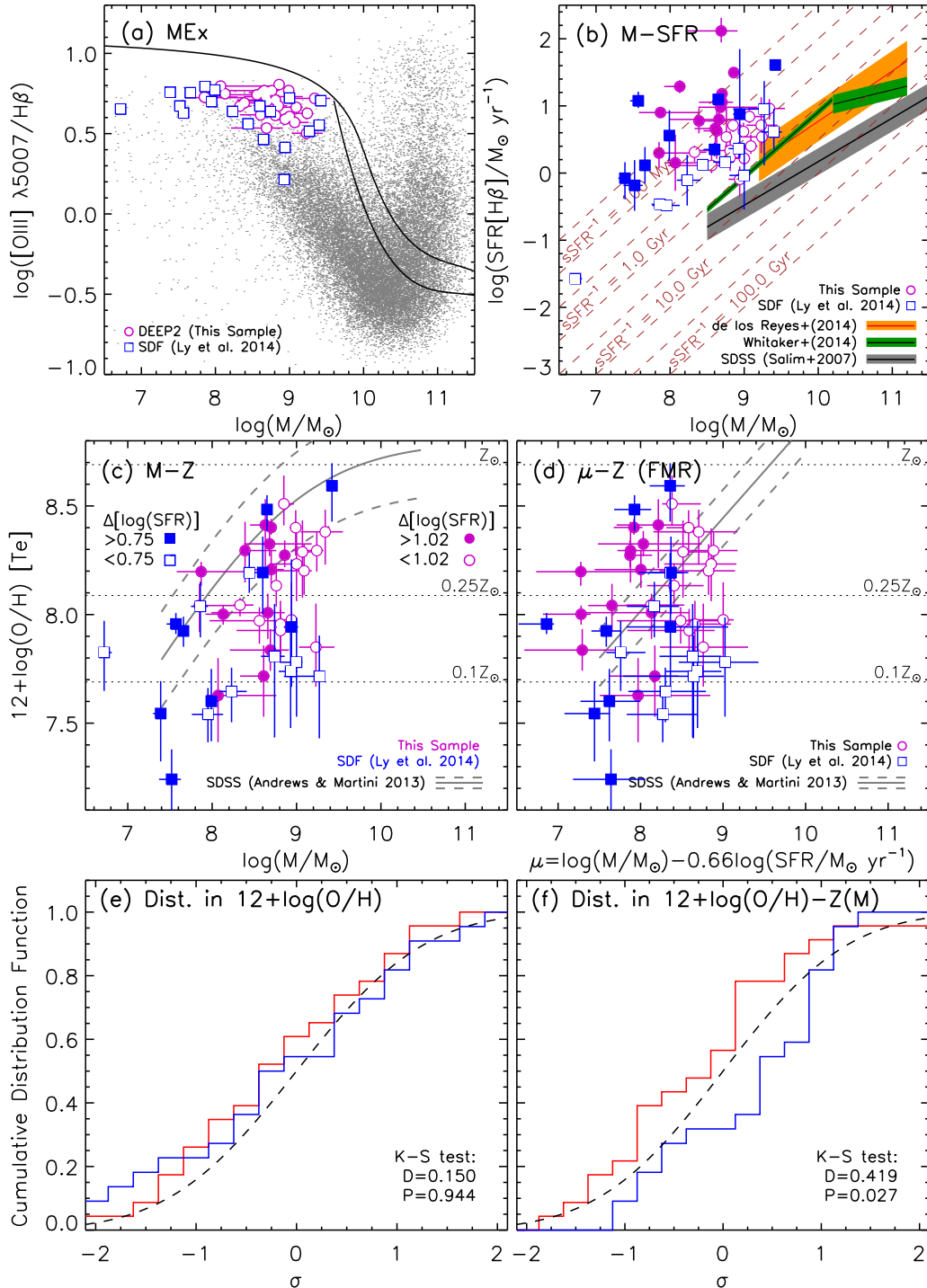
FIG. 4.— Relations between stellar mass and (a) “excitation” ( [\text{O III}]/\text{H}\beta ), (b) dust-corrected \text{H}\beta SFR, (c) metallicity, and (d) metallicity and dust-corrected \text{H}\beta SFR. The DEEP2 [\text{O III}]\lambda 4363 sample is shown by the purple circles. Overlaid as blue squares is the Ly14 [\text{O III}]\lambda 4363 sample. Results from the SDSS sample (Salim et al. 2007; Juneau et al. 2014; AM13) is illustrated in gray. For comparison, we also overlay in panel (b) the stellar mass–SFR relation of \text{H}\alpha -selected galaxies at z = 0.8 (de los Reyes et al. 2014) and mass-selected star-forming galaxies at z = 0.5-1 (Whitaker et al. 2014a) in orange and green, respectively. For direct metallicity comparisons, we illustrate the results of AM13, which stacked spectra to measure average T_e -based metallicities. Panels (e) and (f) show the cumulative distribution functions for two samples with low (open symbols in (b)–(d); blue line) and high SFRs (filled symbols; red line) when the DEEP2 and SDF samples are combined. The K-S statistics (D) and the probability that the two distributions are identical (P) are given in the lower right-hand corner.
