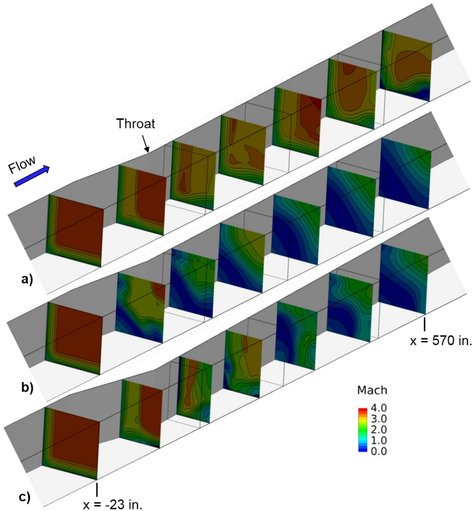
Figure 6. Mach number contours at axial stations of the 10x10 SWT second throat from the CFD simulations at Mach 3.5. a) w_{TH} = 98.57 inches and p_1/p_0 = 13.93 , b) w_{TH} = 98.57 inches and p_1/p_0 = 17.86 , and c) w_{TH} = 72.29 inches and p_1/p_0 = 18.49 .
