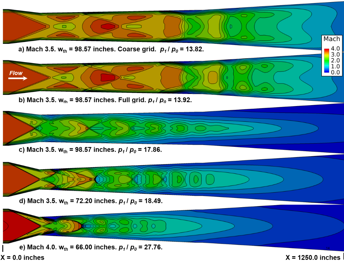
Figure 4. Mach number contours on the horizontal symmetry plane of the 10x10 SWT second throat from the CFD simulations at Mach 3.5 and Mach 4.0.
