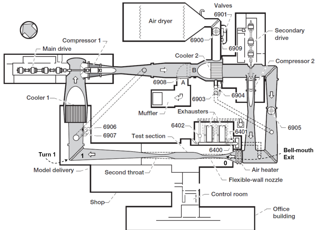
Figure 1. Plan view of the NASA Glenn Abe Silverstein 10x10 foot supersonic wind tunnel.
