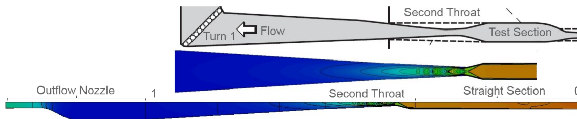
Figure 2. Flow domain for the CFD simulations of the 10x10 SWT second throat.
