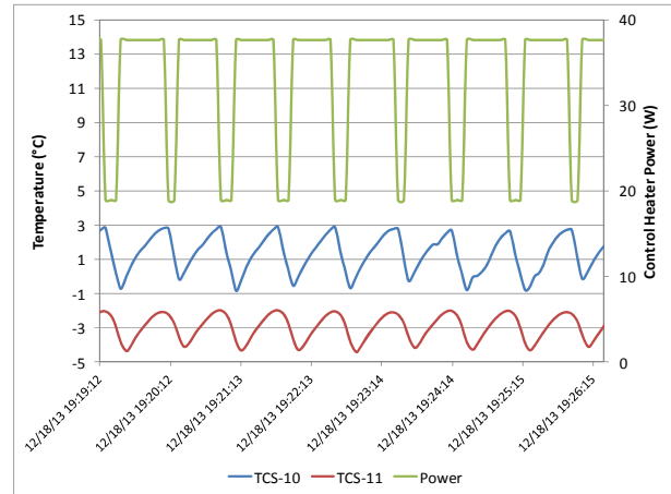
Figure 18. Temperature Oscillations with 38W/19W Reservoir Control Heater Power
