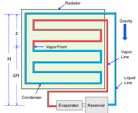
Figure 3. Gravitational Pressure Head in LHP with Vertical Condenser
