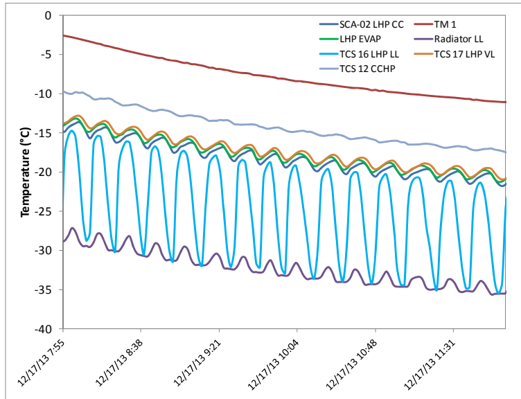
Figure 11. Oscillating Reservoir Temperature during Cold Transition Test
