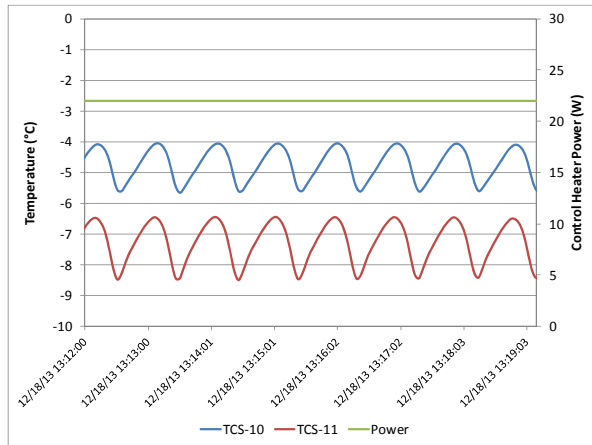
Figure 17. Temperature Oscillations with 22W Reservoir Control Heater Power
