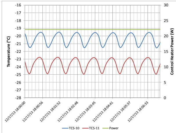
Figure 13. Reservoir Temperature during Quasi-Steady State
