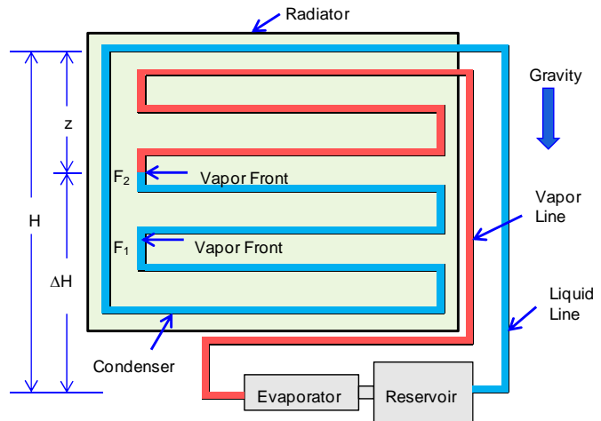
Figure 7. Vapor Front Moves Back and Forth between F 1 and F 2
