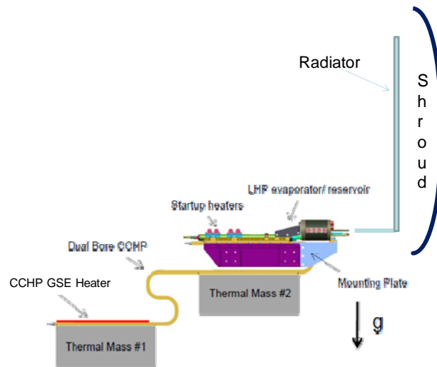
Figure 8. Schematic of Test Setup of ATLAS LTCS TV Testing
