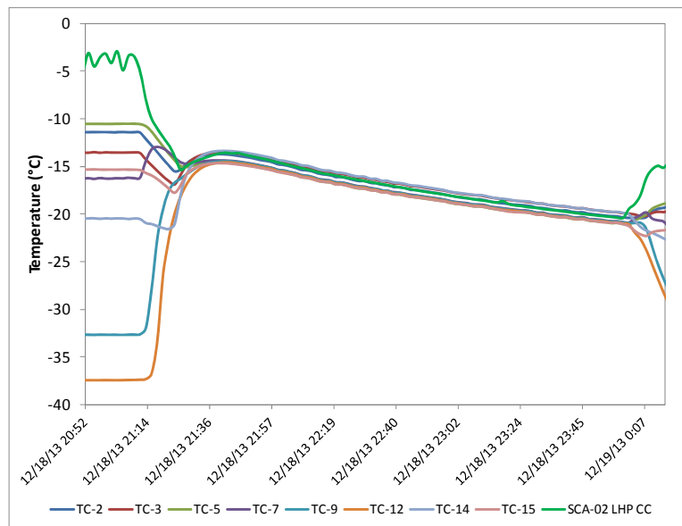
Figure 21. Radiator Temperature with and without Control Heater Power
