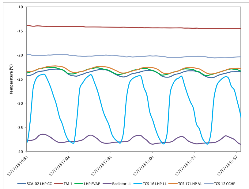
Figure 12. Oscillating Reservoir Temperature during Quasi-Steady State
