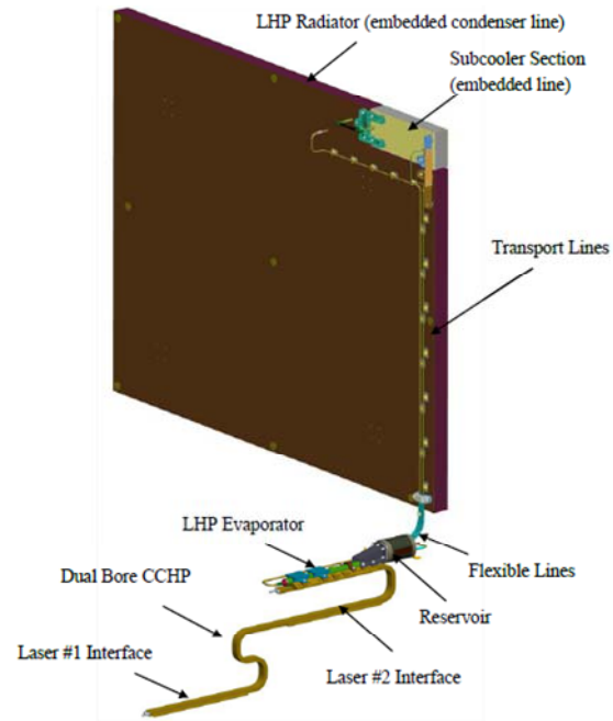
Figure 1. Schematic ATLAS TCS
