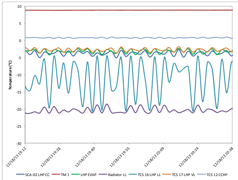
Figure 16. Oscillating Temperatures during Quasi-Steady State with 196W and -78^{\circ}\text{C} Sink Temperature
