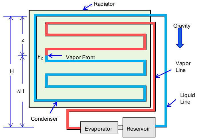
Figure 6. Vapor Length at Its Minimum Value
