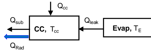
Figure 4. Reservoir Energy Balance
