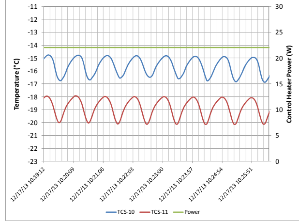
Figure 14. Oscillating Reservoir Temperature during Cold Transition
