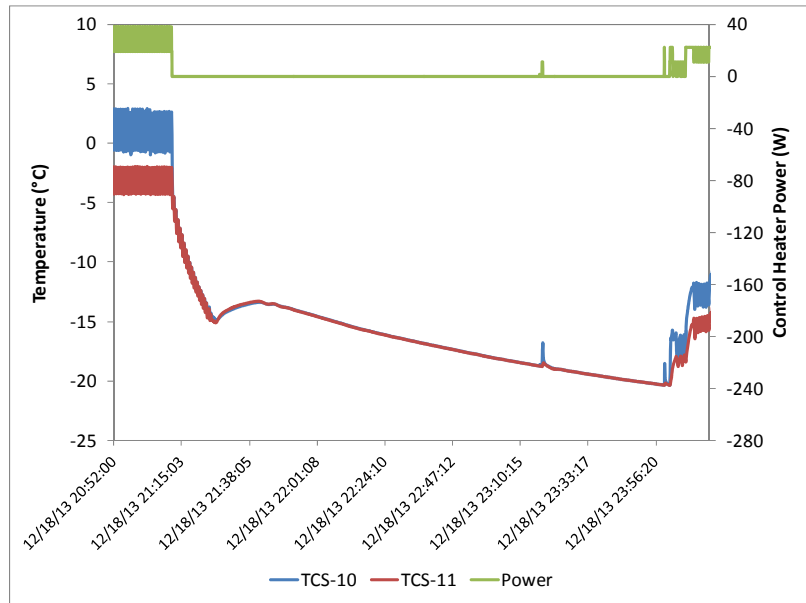
Figure 20. Reservoir Temperatures with and without Control Heater Power
