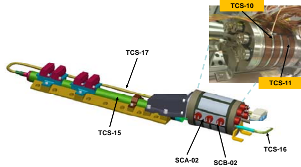
Figure 9. Some Temperature Sensors on the LHP
