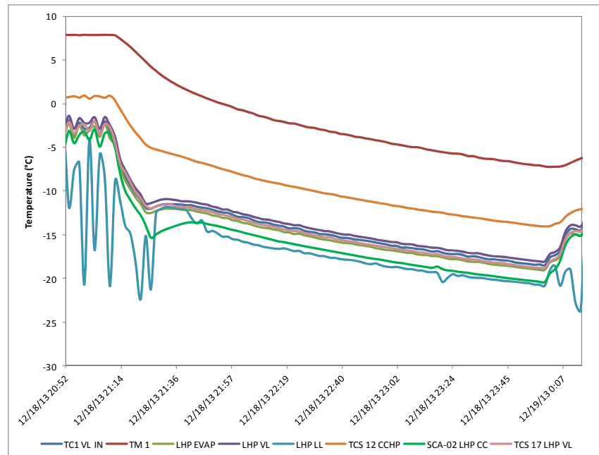
Figure 19. Loop Temperatures with and without Control Heater Power
