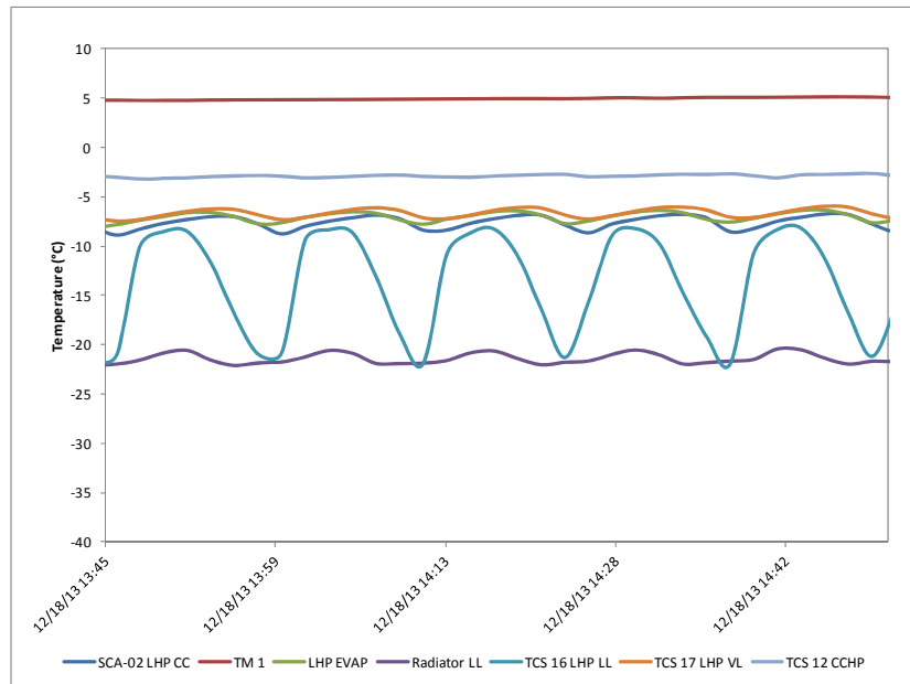
Figure 15. Oscillating Temperatures during Quasi-Steady State with 196W and -78^{\circ}\text{C} Sink Temperature
