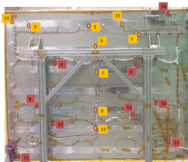
Figure 10. Thermocouples on the Radiator
