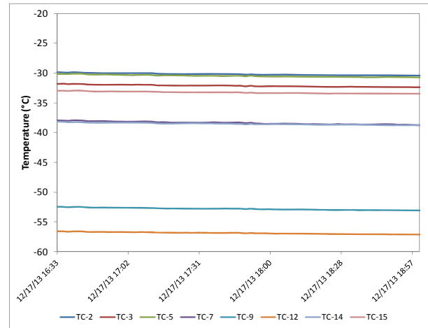
Figure 22. Radiator Temperatures during Oscillations with 38W/19W Reservoir Power
