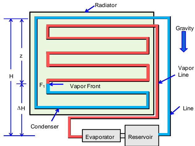
Figure 5. Vapor Length at Its Maximum Value
