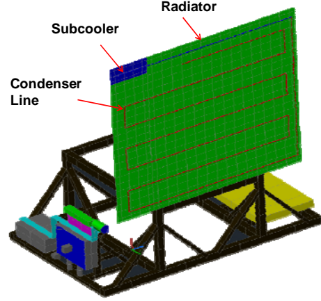
Figure 2. The Vertical Radiator
