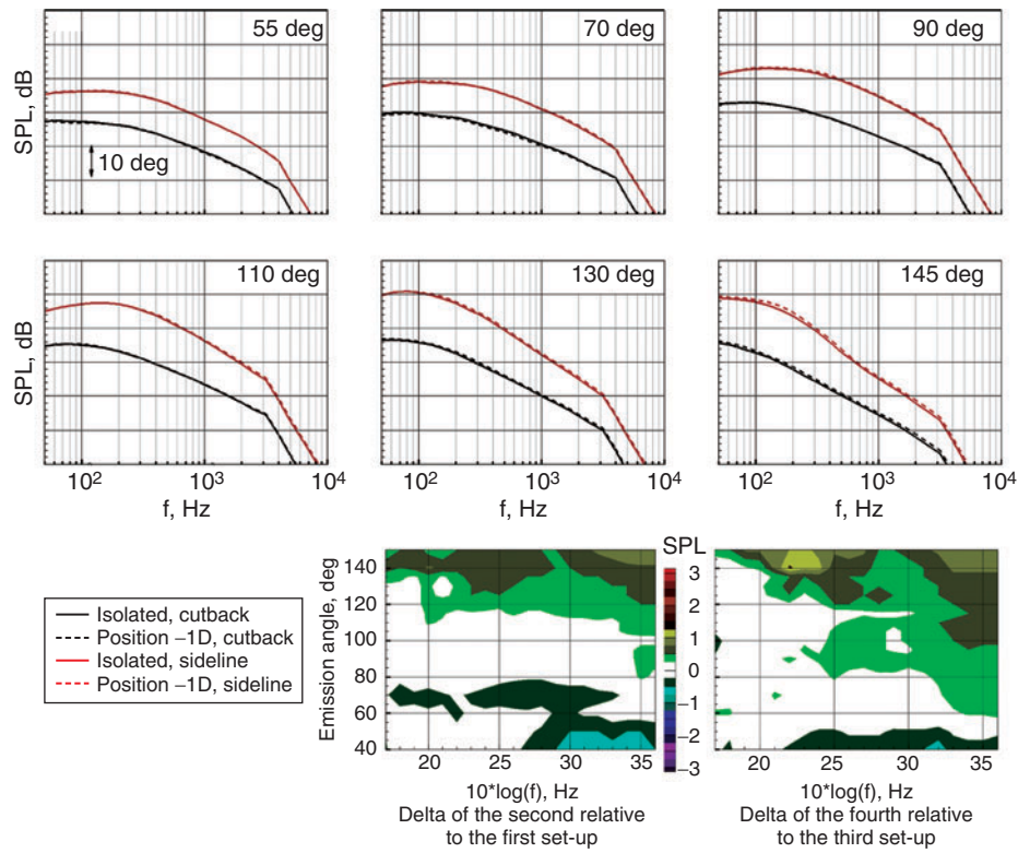
Figure 6: Far-field spectra at cutback and sideline power of isolated jet noise compared to installed at the x/D = -1 position, M_T = 0.2 .
