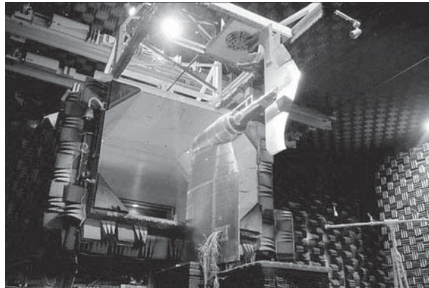
Figure 3: Boeing Low Speed Aeroacoustic Facility configuration for the BWB PAA experiment with the simulated BWB airframe model.
