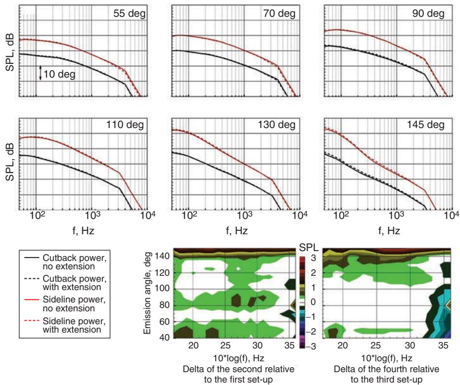
Figure 5: The effect of the nozzle extension on the full scale spectra of the high bypass ratio axisymmetric nozzle at cutback and sideline conditions, M_T = 0.24 . Each color contour level is 0.25 dB.
