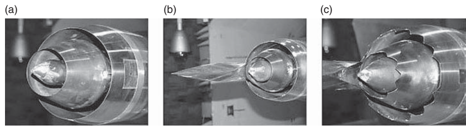
Figure 7: Nozzle configurations, a. LBPR axisymmetric, b. HBPR with pylon, c. Chev2 chevron nozzle.
