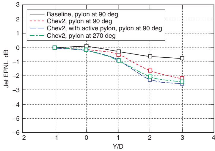
Figure 27: Normalized jet noise EPNLdB vs. X/D at sideline power.
