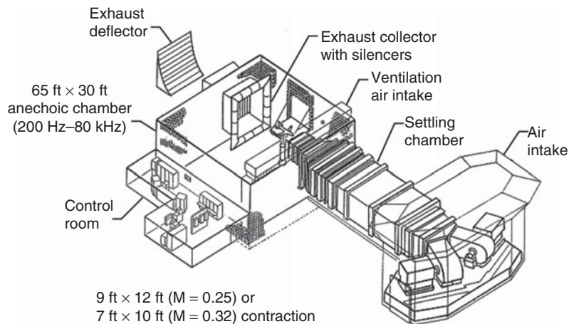
Figure 2: Boeing's Low Speed Aeroacoustic Facility (LSAF).
