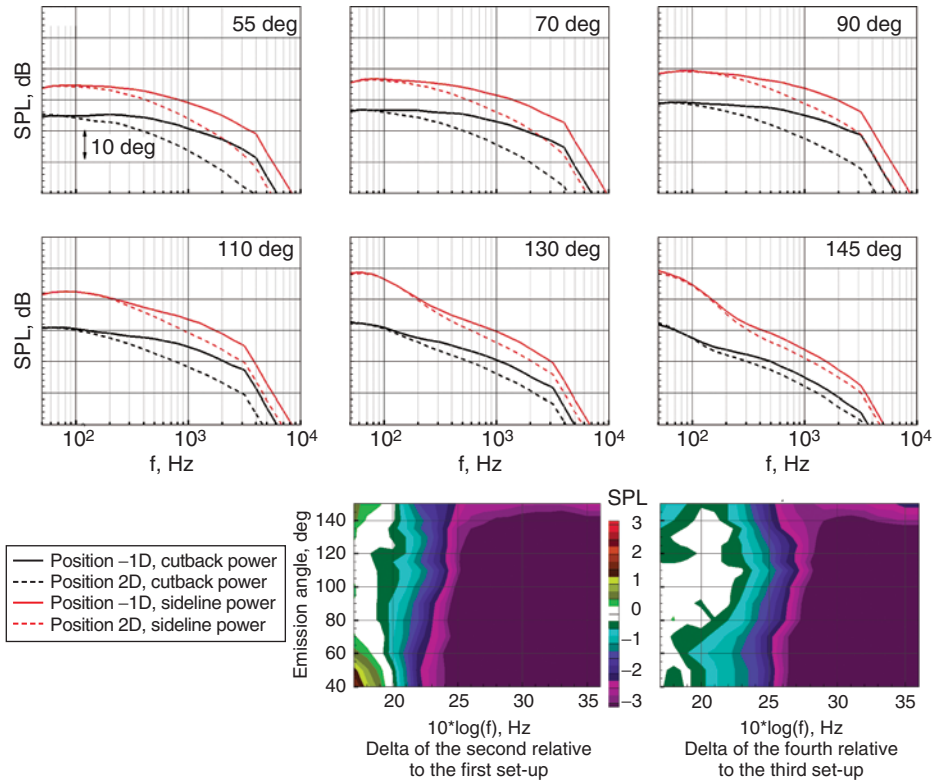
Figure 22: Shielding effect for the HBPR nozzle with pylon at 270 degrees and Chev2 at cutback and sideline power as a function of fan diameter referenced to the wing trailing edge, M_T = 0.2 .
