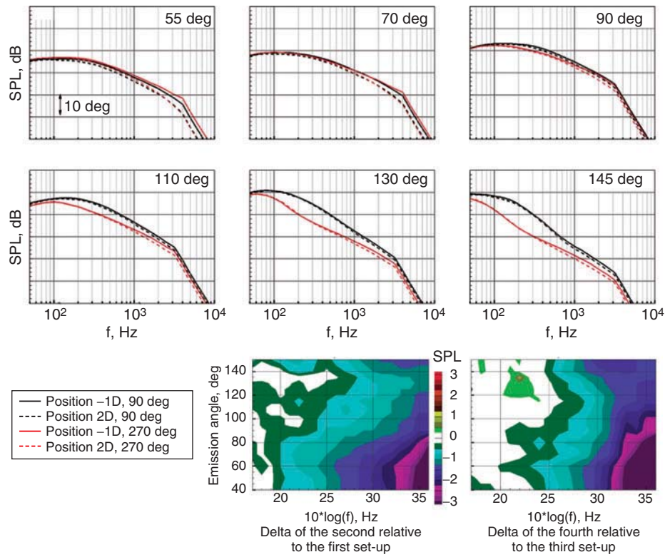
Figure 18: Shielding effect for the HBPR nozzle with pylon oriented at 90 and 270 degrees at sideline power as a function of fan diameter referenced to the wing trailing edge, M_T = 0.2 .
