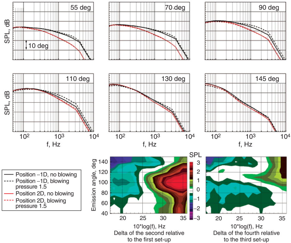
Figure 24: Shielding effect for the active pylon nozzle with and without blowing as a function of fan diameter referenced to the wing trailing edge, M_T = 0.2 . Blowing pressure ratio = 1.5.
