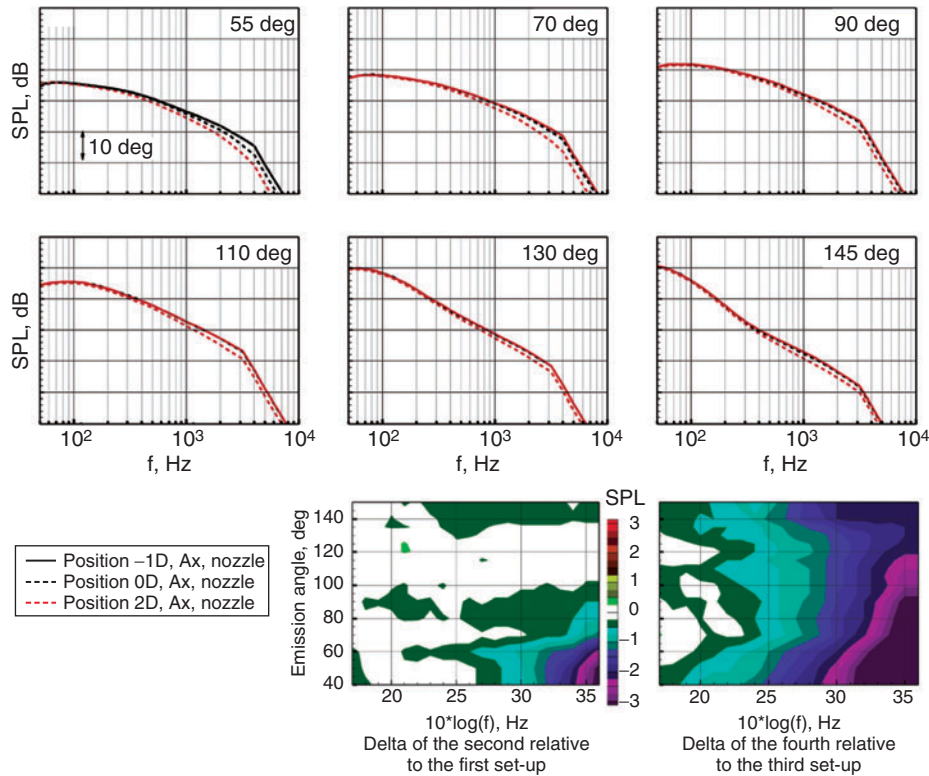
Figure 17: Shielding effect for the HBPR axisymmetric nozzle at sideline power as a function of fan diameter referenced to the wing trailing edge, M_T = 0.2 .
