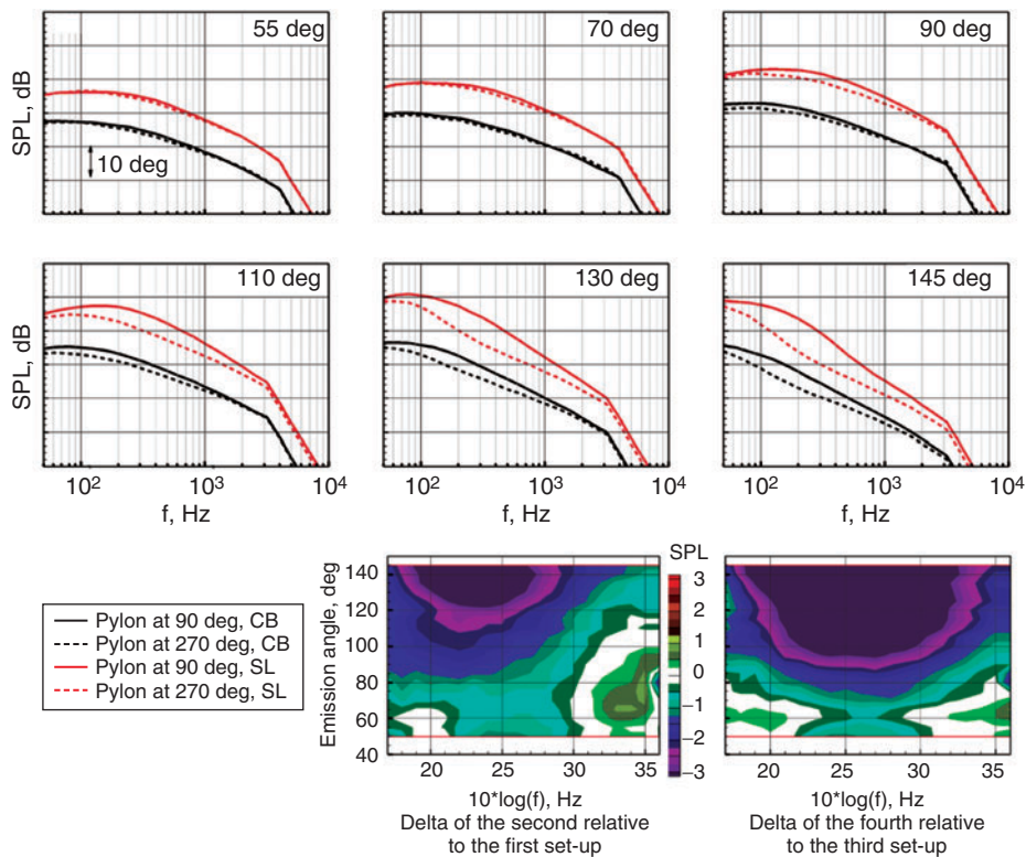
Figure 14: Effect of pylon orientation at cutback and sideline power for the HBPR nozzle. Pylon at 90 deg oriented towards the microphones of the polar angle array at 90 degrees. M_T = 0.2 .
