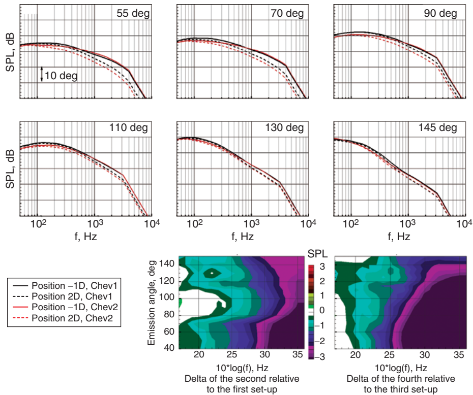
Figure 21: Shielding effect for the HBPR nozzle with pylon at 90 degrees and different chevron configurations at sideline power as a function of fan diameter referenced to the wing trailing edge, M_T = 0.2 .
