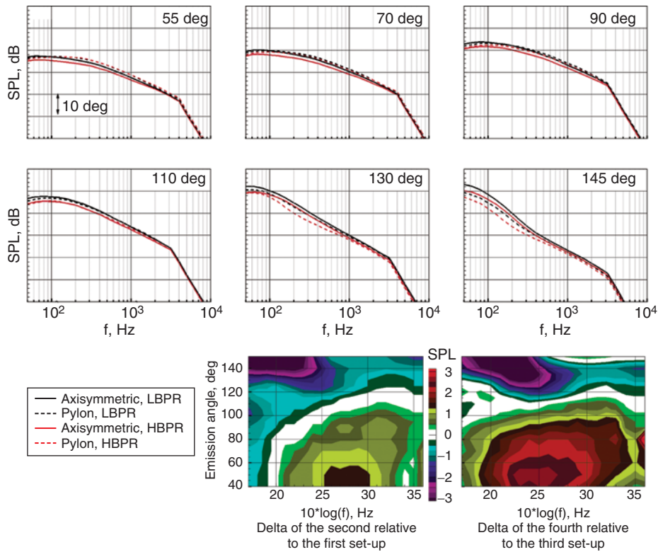
Figure 12: Pylon effect for low and high bypass ratio nozzles at sideline power, M_T = 0.2 .
