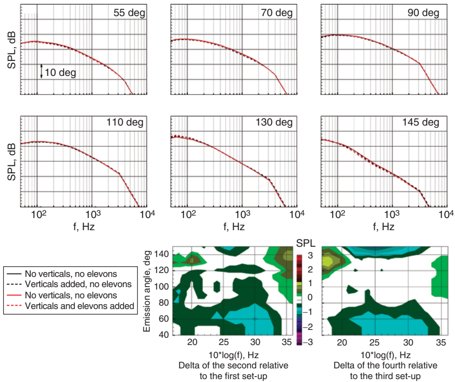
Figure 26: Effect of the elevons and verticals on shielding with the nozzle location at two diameters upstream of the wing trailing edge. Sideline power, M_T = 0.2 .
