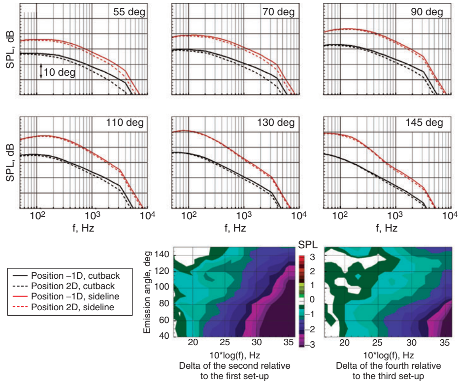
Figure 19: Shielding effect for the HBPR nozzle with pylon at cutback and sideline power as a function of fan diameter referenced to the wing trailing edge, M_T = 0.2 .
