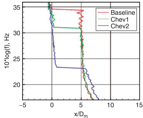
Figure 16: Variations of jet noise source location with nozzle configuration as seen by the phased array at sideline power. HBPR nozzle, M_T = 0.2 .
