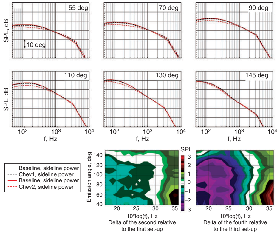
Figure 15: Chevron effect for the mildly (Chev1) and aggressively immersed chevron (Chev2) design at sideline power, M_T = 0.2 .
