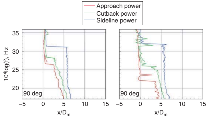
Figure 20: Source location changes with power setting for the baseline nozzle with pylon at static (left plot) and wind on (right plot) conditions as seen by the phased array.
