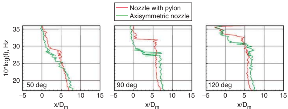
Figure 13: Phased array source locations for an axisymmetric nozzle and a nozzle with pylon at sideline power, M_T = 0.24 .
