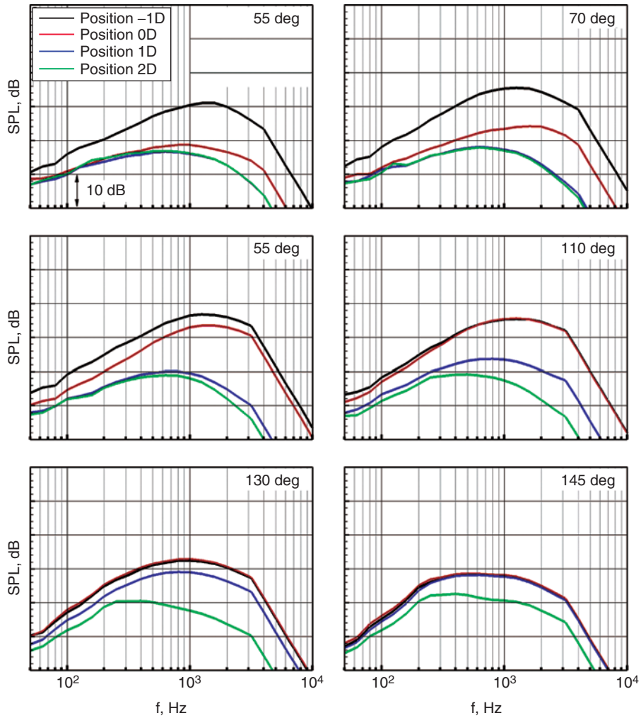
Figure 29: Spectral plot of broadband point source shielding as a function of X/D , M_T = 0.2 .
