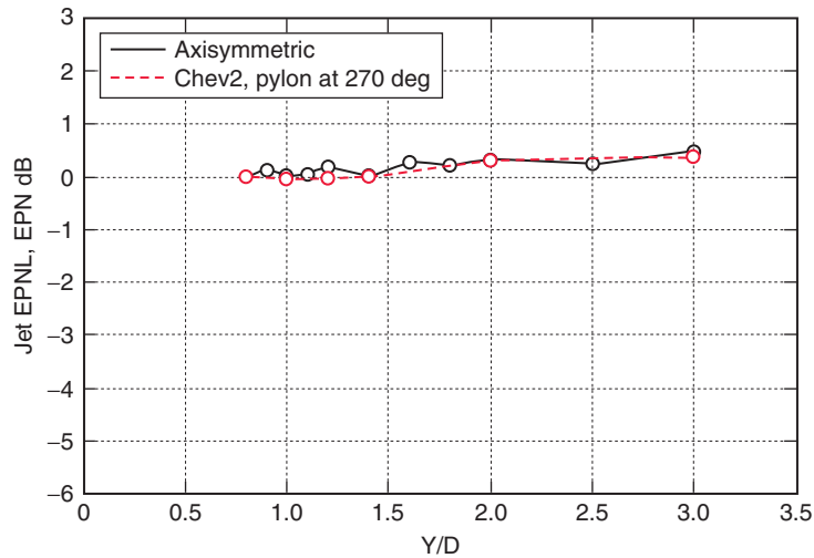
Figure 25: The effect on jet noise of spacing of the jet centerline above the airframe surface, Y/D , with the jet nozzle fixed, axially, at X/D = 2 upstream of the trailing edge, sideline gas condition, EPNL calculated from the polar array of microphones at azimuth 90 deg. For each nozzle, the EPNL level at a given Y/D is referenced to its EPNL at Y/D = 0.8 .
