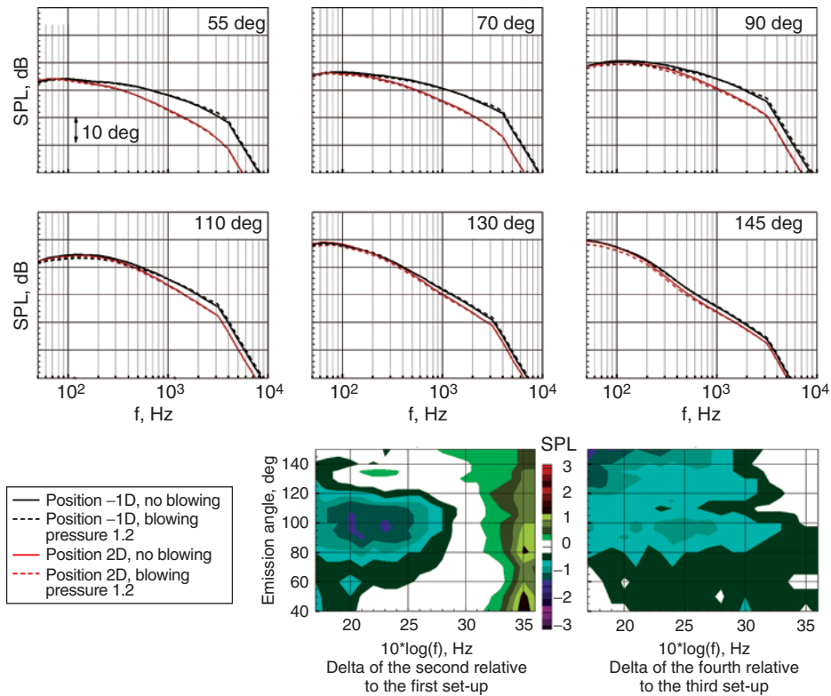
Figure 23: Shielding effect for the active pylon nozzle with and without blowing as a function of fan diameter referenced to the wing trailing edge, M_T = 0.2 . Blowing pressure ratio = 1.2.
