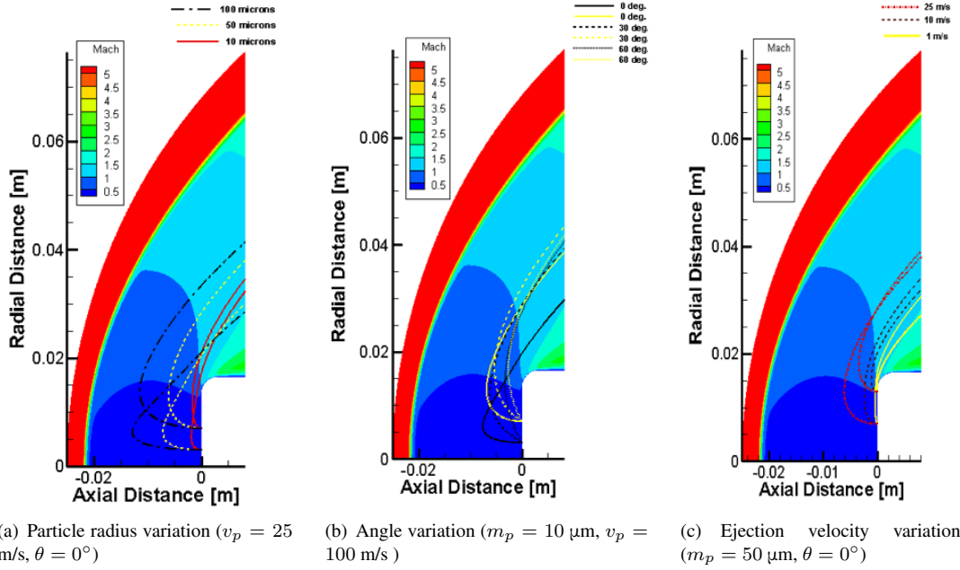
Figure 1. Particle trajectories as a result of the study for the ejection parameters of spalled particle in a Mach 5 argon flow
