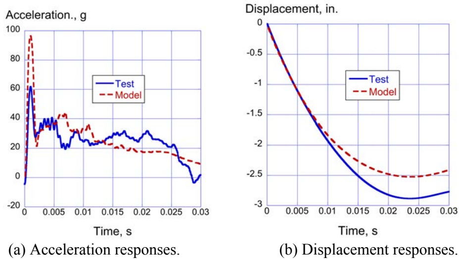
Figure 7. Acceleration and displacement comparisons for the conusoid component vertical drop test.
