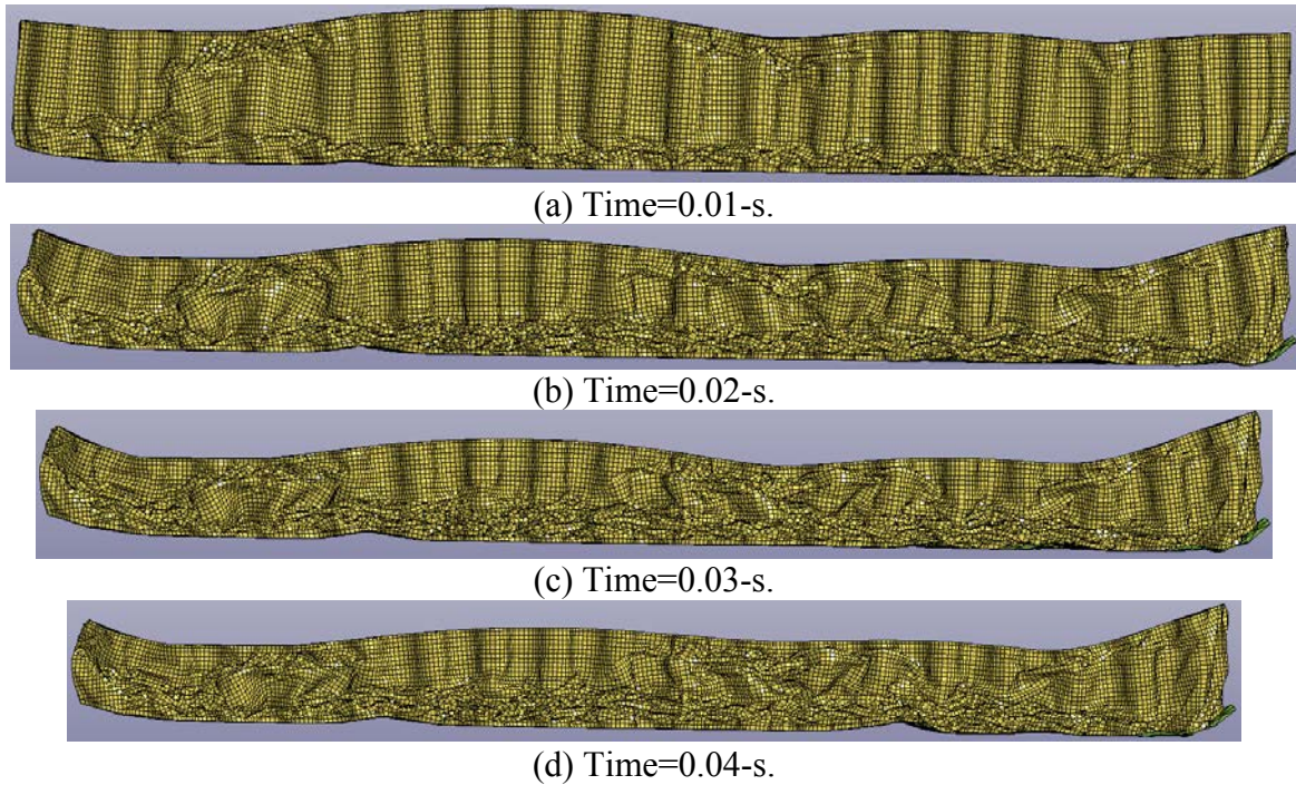
Figure 22. Predicted deformation pattern of the conusoid subfloor.
