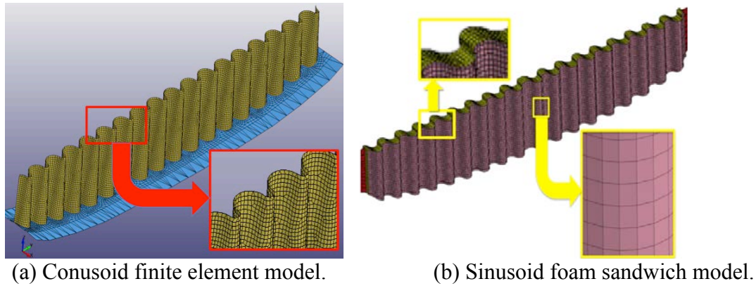
Figure 20. Depictions of the finite element models of the two energy absorbing subfloors.
