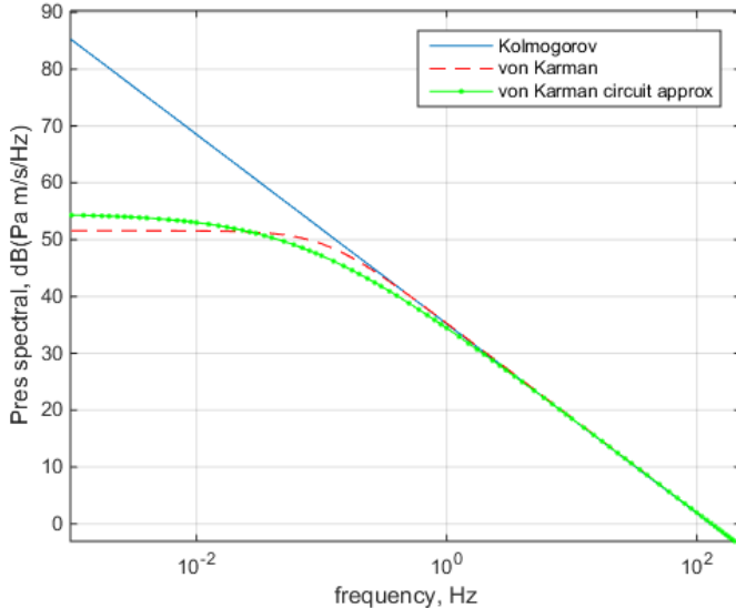
Figure B.10.—Kolmogorov and von Karman spectral for pressure and its von Karman circuit approximation, ( \epsilon = 8.6e-5 m 2 /sec 3 , L = 762 m).
