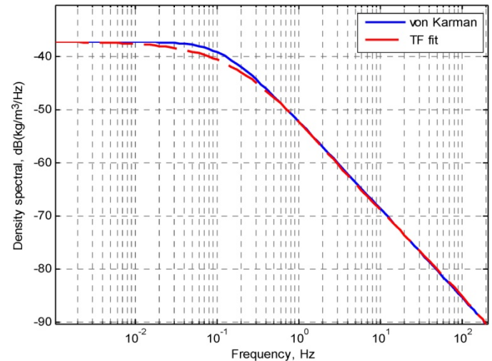
Figure 11.—Density von Karman spectral and its TF fit ( \varepsilon = 8.6e-5 \text{ m}^2/\text{sec}^3 , L = 762 \text{ m} ).
