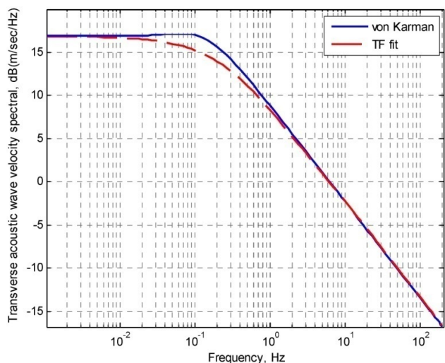
Figure 6.—Transverse von Karman spectral, final adjusted TF fit ( \epsilon = 8.6e-5 m^2/sec^3 , L = 762 m).
