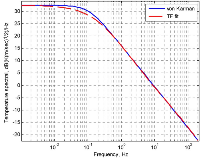
Figure C.7.—Temperature von Karman spectral and its TF fit ( \epsilon=8.6e-5 m 2 /sec 3 , L=762 m).
