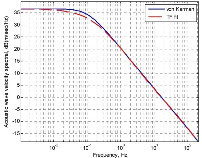
Figure C.8.—Von Karman acoustic wave velocity spectral due to temperature gust and its TF fit ( \epsilon = 8.6e-5 m 2 /sec 3 , L = 762 m).
