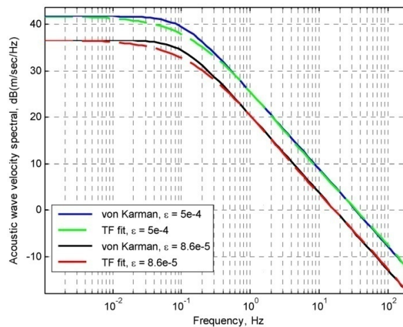
Figure 8.—Von Karman acoustic wave velocity spectral due to temperature gust and its TF fits for different eddy dissipation rates ( L = 762 m).
