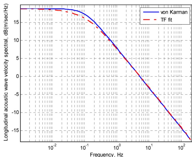
Figure 5.—Longitudinal von Karman spectral, final adjusted TF fit ( \epsilon = 8.6e-5 m^2/sec^3 , L = 762 m).
