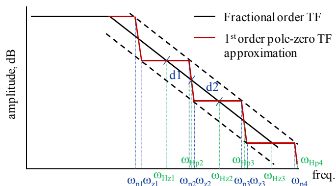
Figure C.1.—Pictorial diagram of fractional order TF fit.
