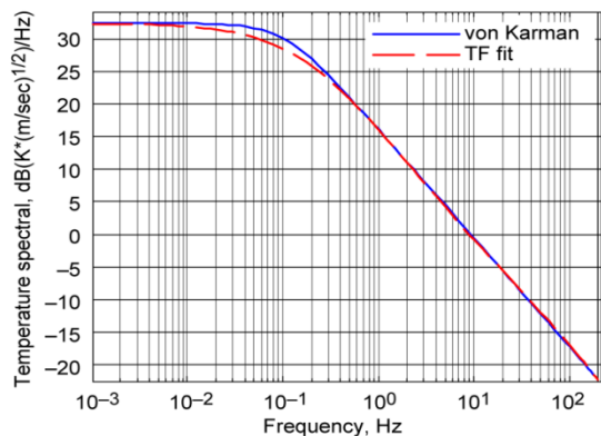
Figure 7.—Temperature von Karman spectral and its TF fit ( \varepsilon = 8.6e-5 \text{ m}^2/\text{sec}^3 , L = 762 m).
