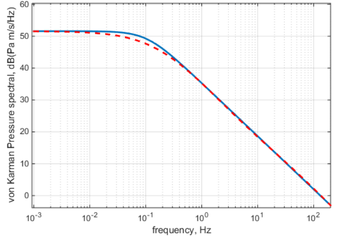
Figure 10.—Pressure von Karman spectral and its TF fit ( \varepsilon = 8.6e-5 \text{ m}^2/\text{sec}^3 , L = 762 \text{ m} ).
