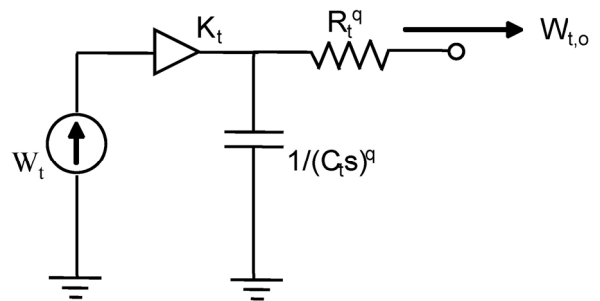
Figure B.1.—Equivalent circuit TF of atmospheric disturbance.
