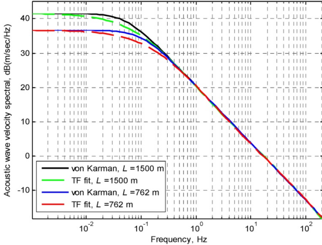
Figure 9.—Von Karman acoustic wave velocity spectral due to temperature gust and its TF fits for different integral scale lengths ( \varepsilon = 8.6e-5 \text{ m}^2/\text{sec}^3 ).
