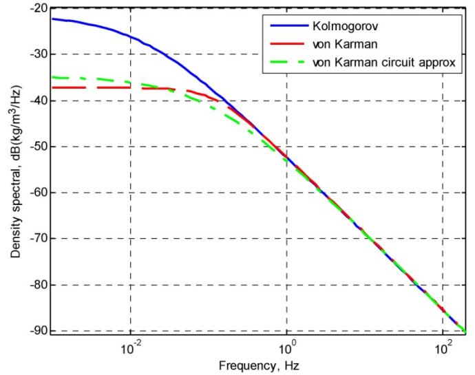
Figure B.11.—Kolmogorov and von Karman spectral for density and its von Karman circuit approximation ( \epsilon = 8.6e-5 m 2 /sec 3 , L = 762 m).
