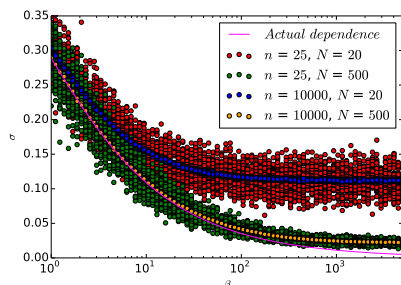
Figure 1. Statistical modeling of the multiplier distribution width \sigma depending on the number of bins, n , and the number of particles per bin, N . The magenta line denotes the actual width (standard deviation) of the \beta distributions.
