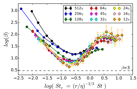
Figure 2. \beta of multiplier pdfs for particle concentration, plotted as a function of St_r (stopping time t_s normalized by the turnover time of an eddy with scale r ), for a variety of binning scales r ranging from 12\eta to 512\eta \approx L/2 . With this scaling, the multiplier pdf \beta values collapse to a universal curve except at the largest scales r > L/10 . A universal curve allows our cascade models to be extended to scales smaller than resolvable by current numerical models.
