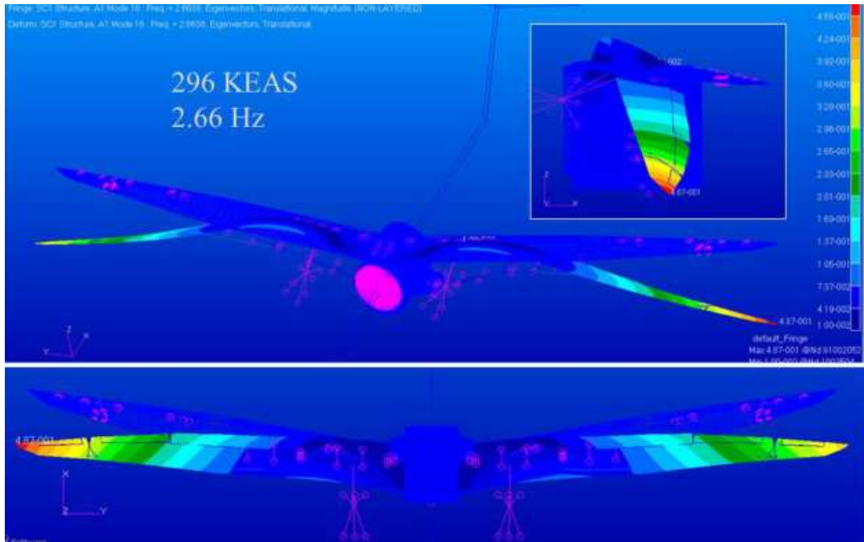
Figure 127. Critical flutter mode for 0-degree NCE reserve fuel case. 296 KEAS and 2.66 Hz.
