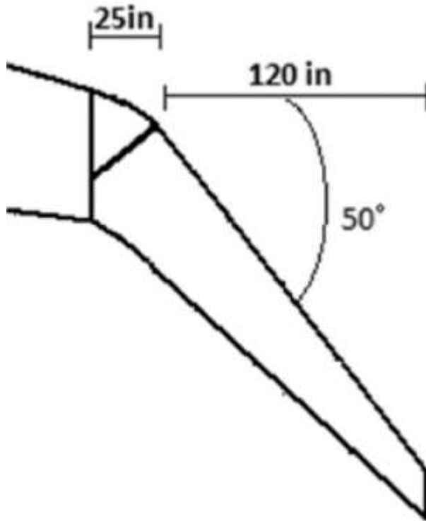
Figure 60. Geometry Sketch of Fully-Swept VGRWT/NCE Tip
