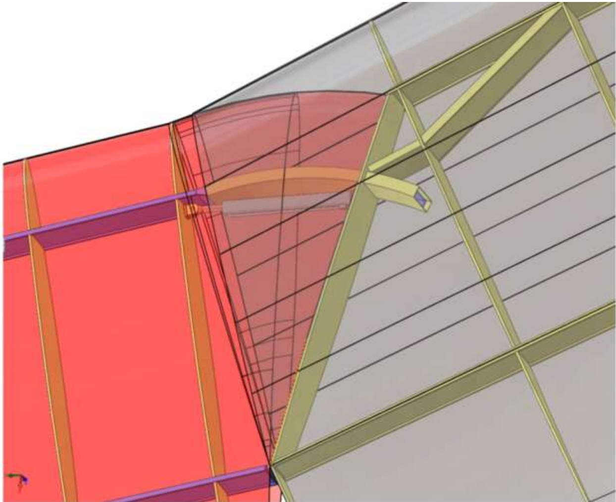
Figure 54. View of NCE-Wing Joint Showing Actuator Connection to NCE Rib and End of NCE Spar Visible in Slider Joint with Wing. NCE Swept Forward 15°.
