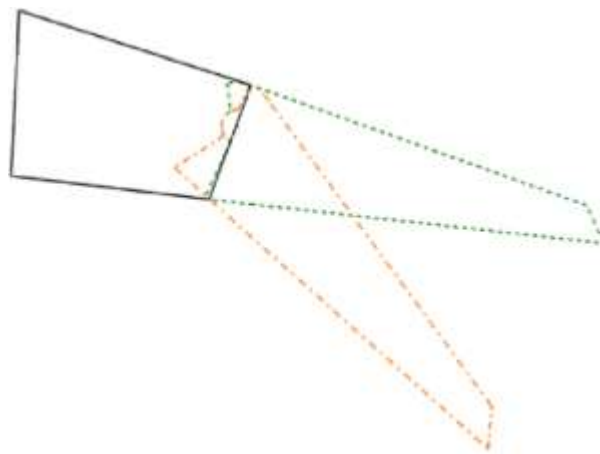
Figure 17. Sketch of Boeing NCE Wingtip Concept
