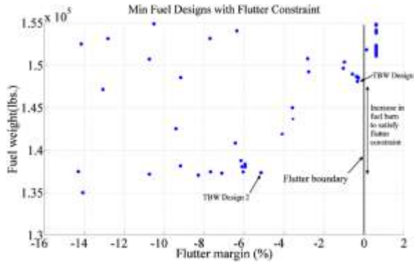
Figure 26. Minimum Fuel Optimized TBW Designs with Flutter as a Constraint
