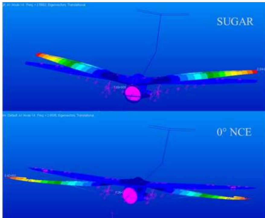
Figure C-8. Full-fuel: Structural mode 14 for baseline SUGAR (2.66 Hz) and 0-deg NCE (2.65) Hz.
