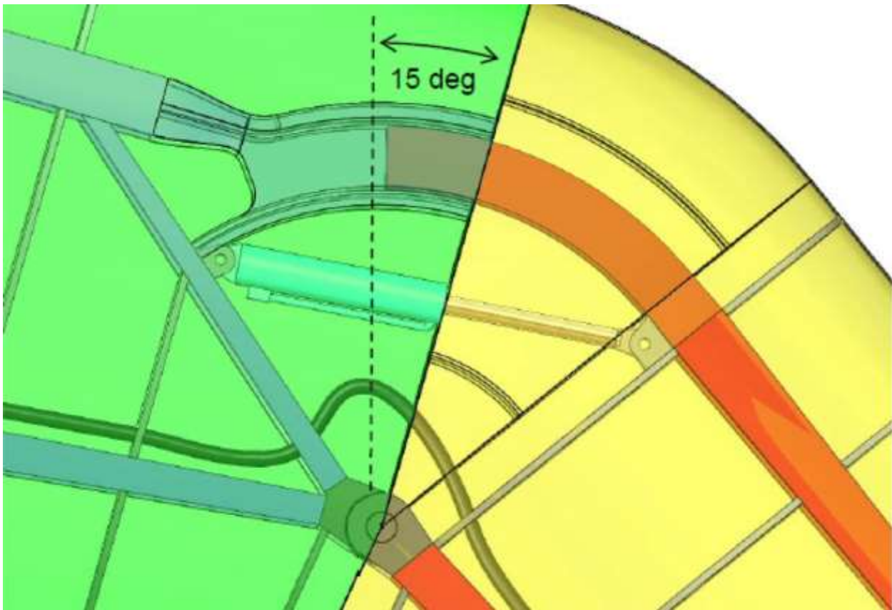
Figure 34. Overhead view of track and beam mechanism with track structure set to transparent showing overlap between track and beam at full sweep.
