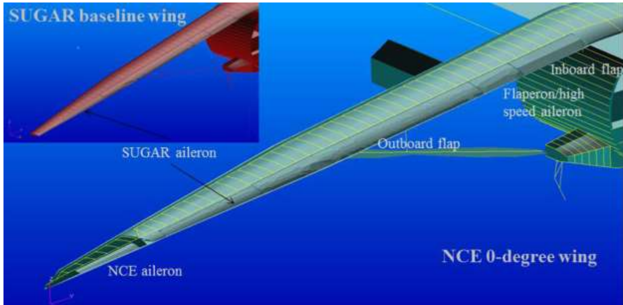
Figure 135. Locations and names of the various control surfaces on the NCE equipped aircraft. For comparison the original SUGAR wing is shown in the inset picture upper left.
