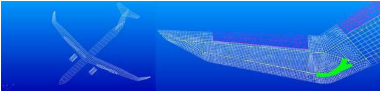
Figure 117. A new aero-mesh (left) was developed for the 26-degree NCE FEM (right).
