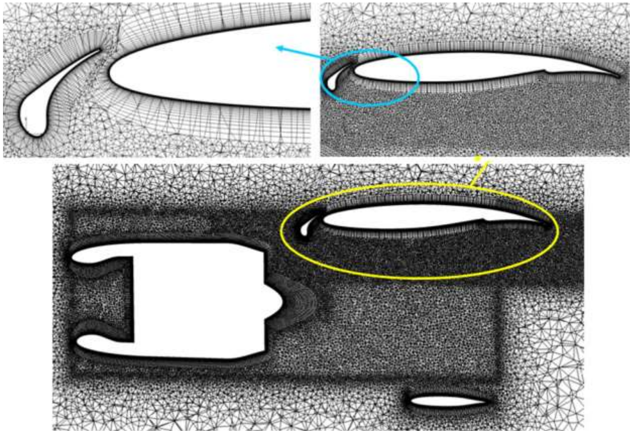
Figure 89. SUGAR Unstructured Geometry at Takeoff
