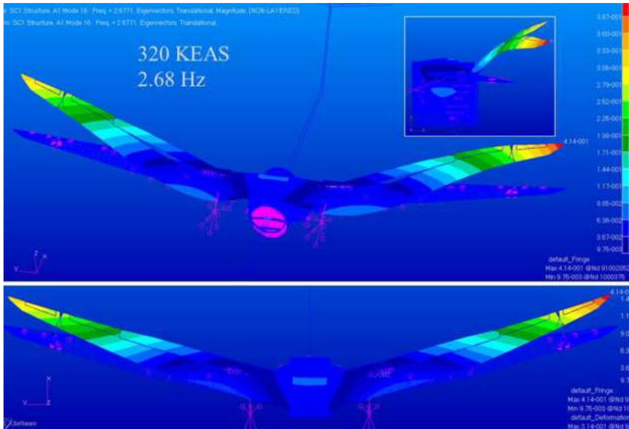
Figure 120. Critical flutter mode for 0-degree NCE full fuel case. 320 KEAS and 2.68 Hz.
