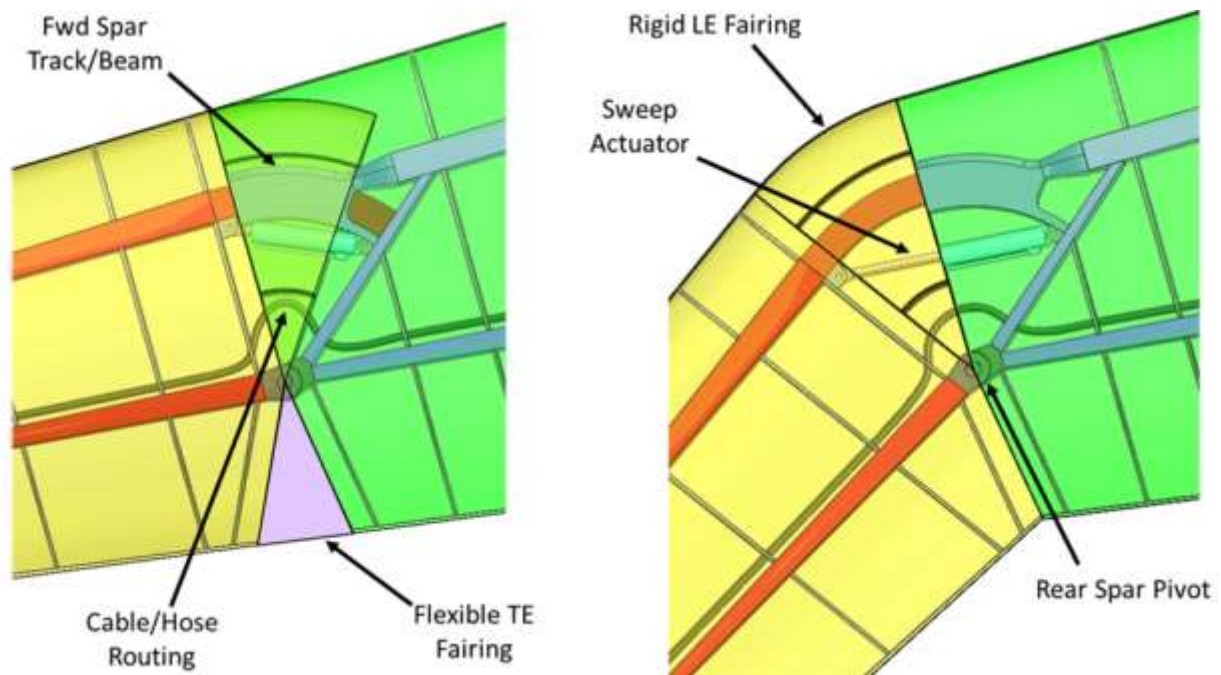
Figure 56. VGRWT Minimum (0 deg) and Maximum Sweep (35 deg)
