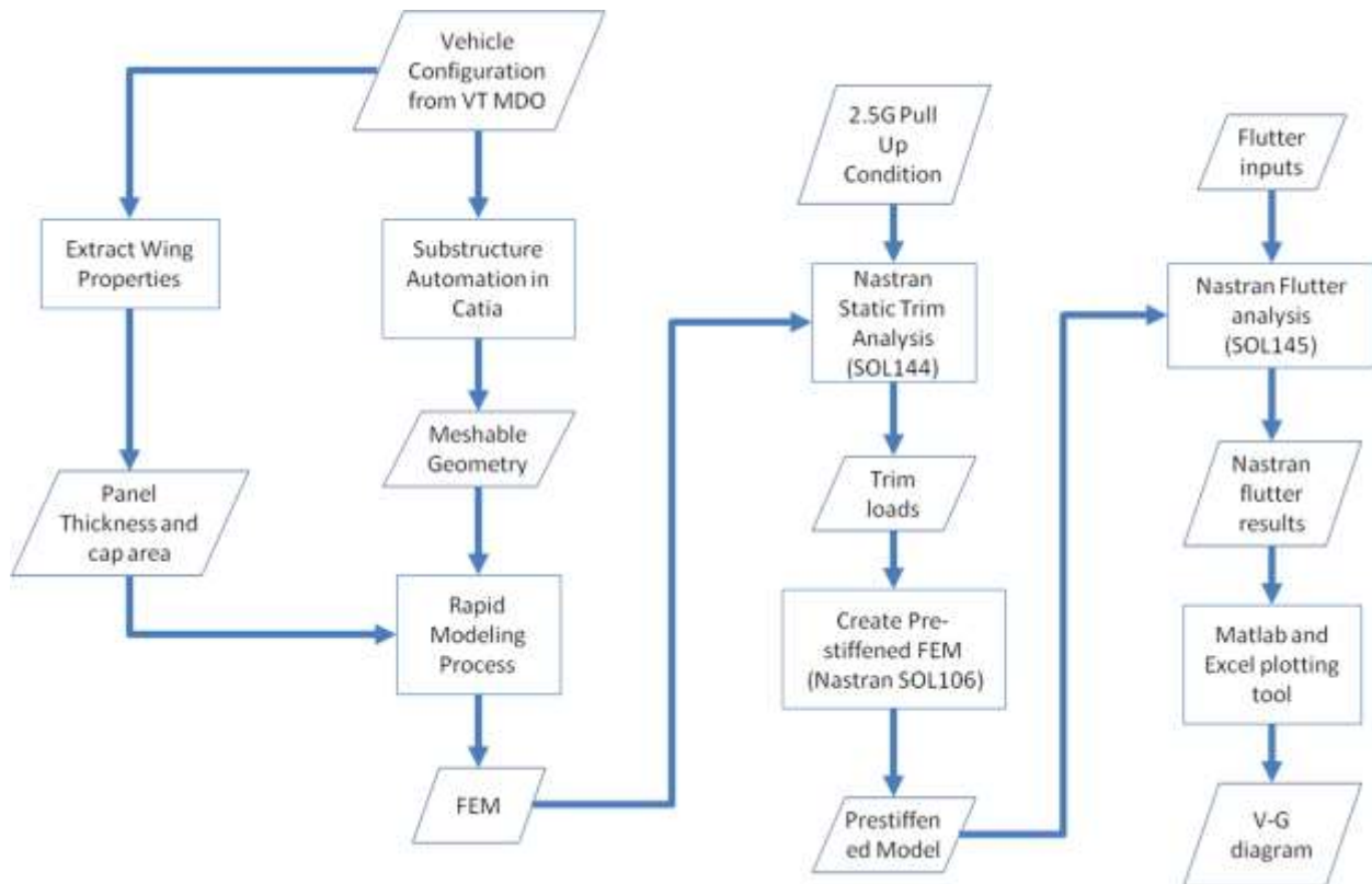
Figure 139. Boeing Process for Modeling and Analyzing Virginia Tech MDO Vehicle
