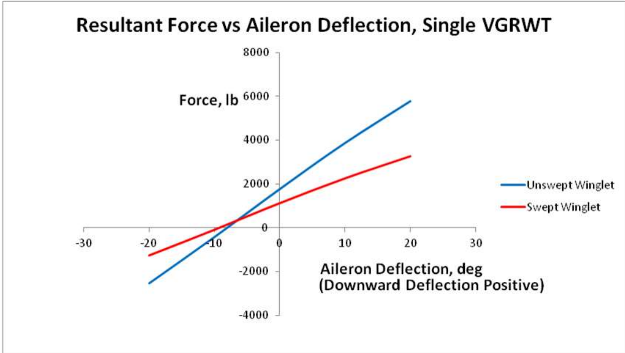
Figure 11. Force vs. Aileron Deflection, Single Wingtip
