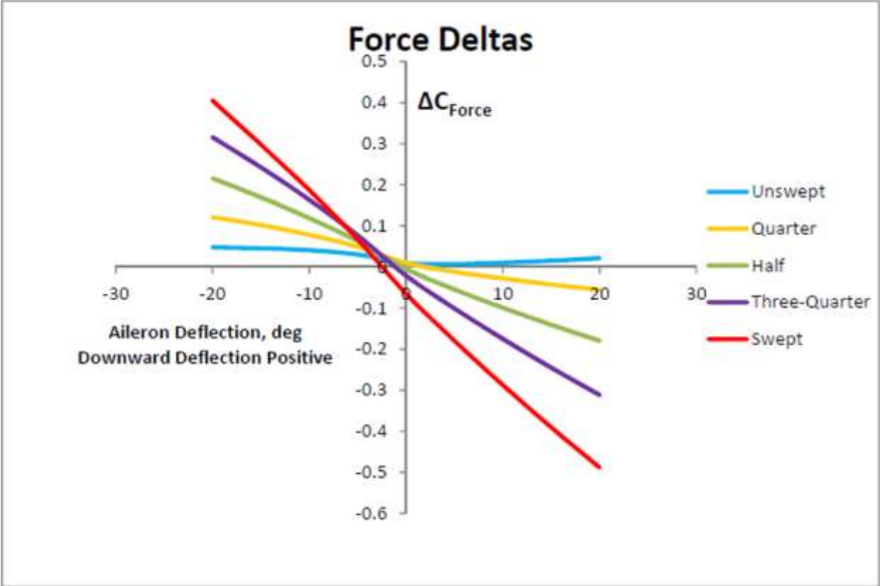
Figure 82. Wingtip Force Coefficient Deltas for VGRWT/NCE Tip as a Function of Sweep and Aileron Deflection
