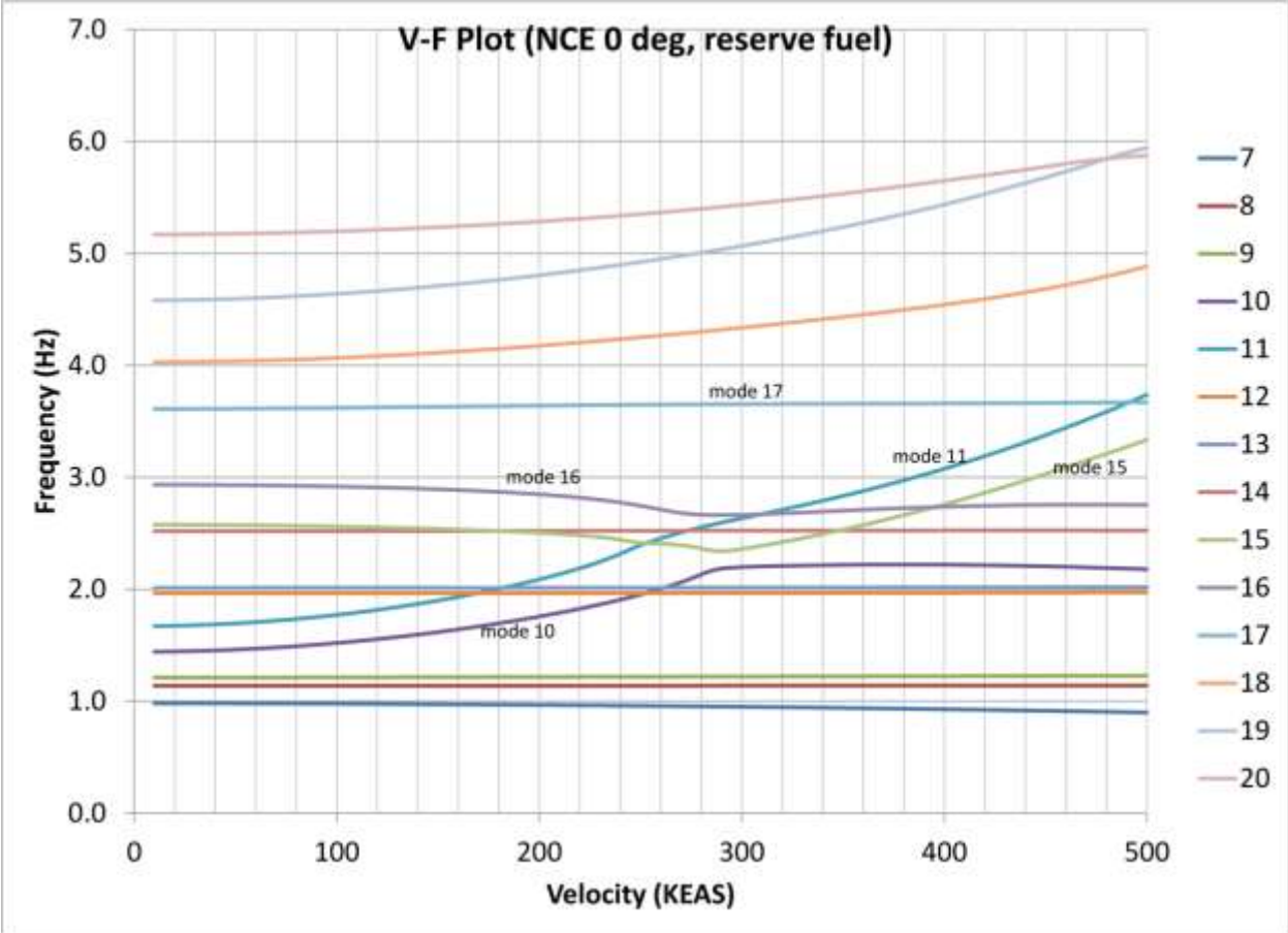
Figure 128. V-F plot for NCE 0-degree reserve fuel case.
