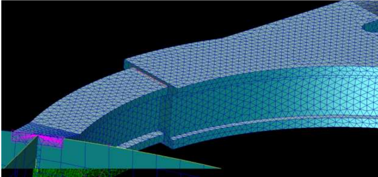
Figure 112. Track and beam interface for 26 degree sweep case. MPC elements (pink) are located at the upper and lower ends of the track and the upper and lower ends of the beam which nests inside the track. Solid elements show on top for clarity. Skeleton view on bottom shows the internal connection between the end of the beam and inside of the track. Note that the MPC on far left is used to rigidly attach the upper beam cap to the wingtip upper spar cap.
