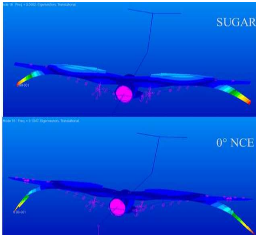
Figure C-10. Full-fuel: Structural mode 16 for baseline SUGAR (3.06 Hz) and 0-deg NCE (3.13) Hz.
