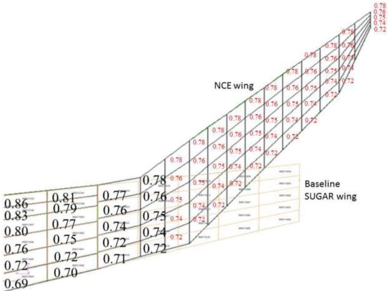
Figure 118. Box-by-box aerodynamic weight factors (NASTRAN WFACT) were applied to the NCE. These values were approximated from the baseline SUGAR aircraft (Boeing Overflow #'s @ Mach 0.82).
