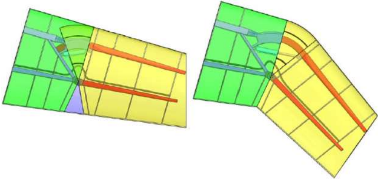
Figure 33. Overview of kinematic model in the unswept (left) and swept (right) positions.
