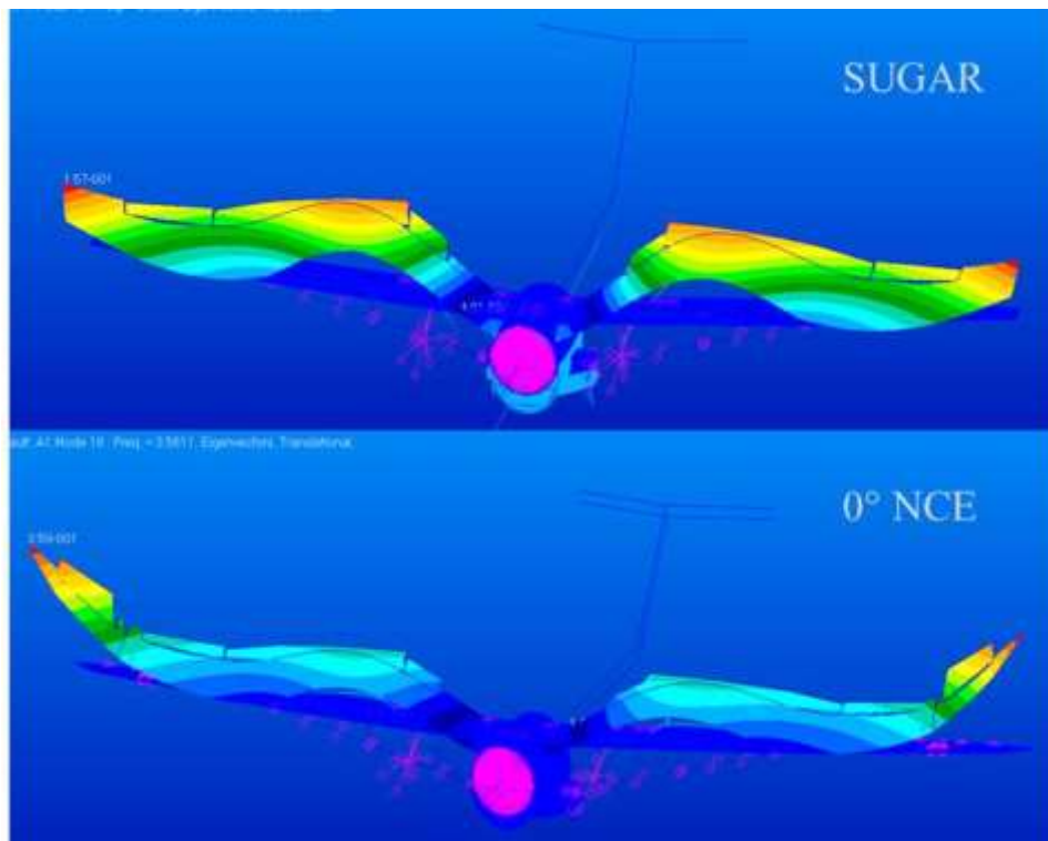
Figure C-12. Full-fuel: Structural mode 18 for baseline SUGAR (3.54 Hz) and 0-deg NCE (3.56) Hz.
