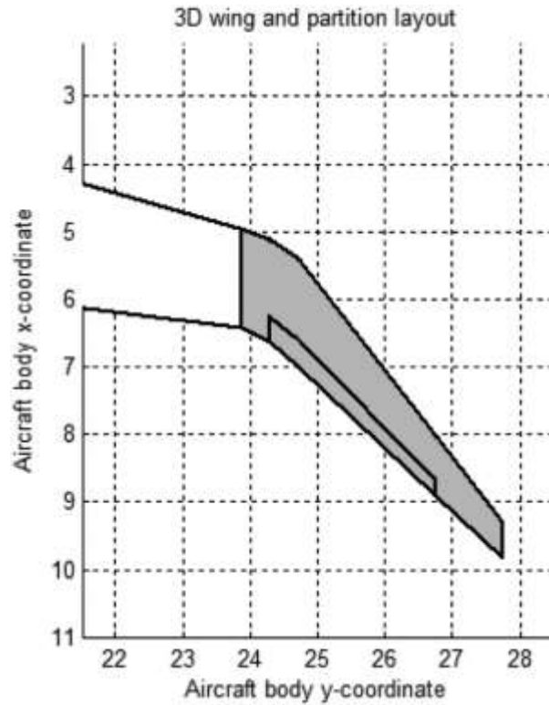
Figure 9. VGRWT Tornado Model, Wingtip Swept at 35^\circ , Pivot at Trailing Edge (Dimensions in meters)
