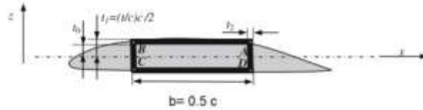
Figure 18(a). Previous VT MDO Structural Model Suitable for Weight Estimation
