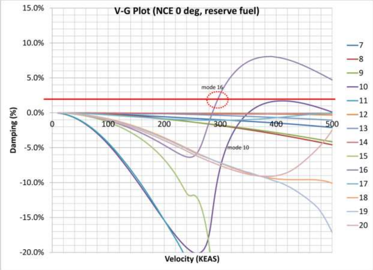
Figure 129. V-G plot for NCE 0-degree reserve fuel case.
