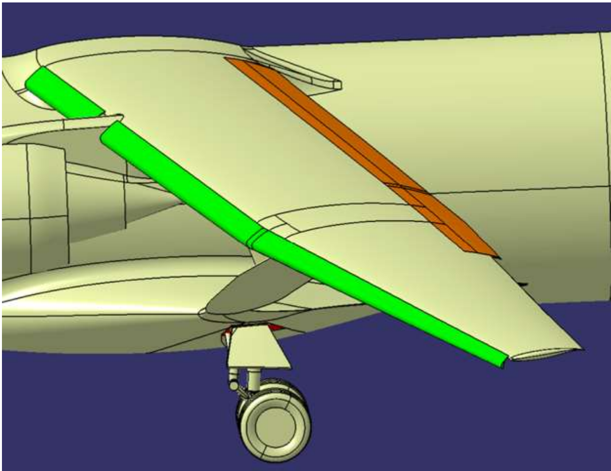
Figure 94. SUGAR Slat System Deployment for Approach/Cutback/Sideline
