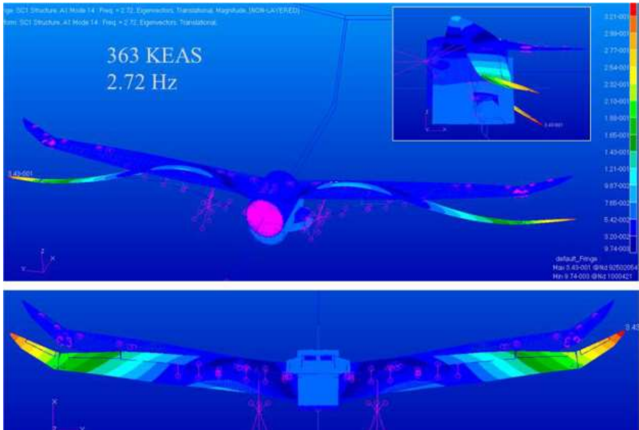
Figure 123. Critical flutter mode for 26-degree NCE full fuel case. 363 KEAS and 2.72 Hz.
