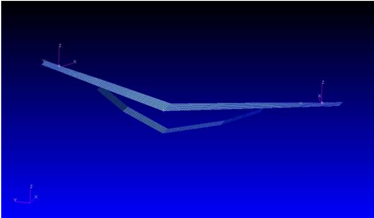
Figure 144. Full Span Doublet Lattice Aero Model
