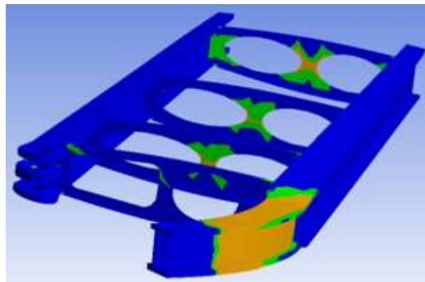
Figure 40. Finite element analysis of full wingtip structure with skin and fairings hidden showing structural margin greater than unity.
