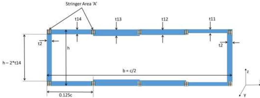
Figure 47. Sketch of the MDO Cross Section Used to Calculate Cross-Sectional Properties of Components
