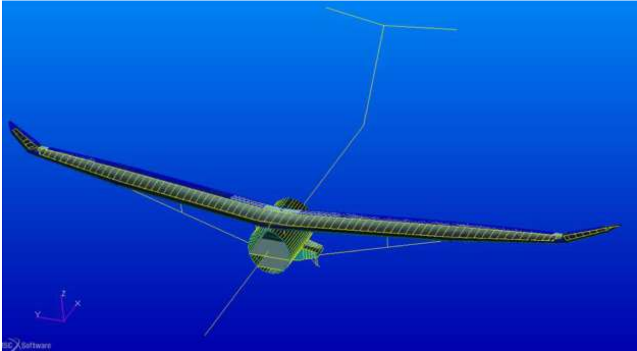
Figure 114. The structural FEM of the NCE equipped aircraft was developed by NextGen and provided to VT. The 26-degree, or \frac{3}{4} sweep configuration is shown here.
