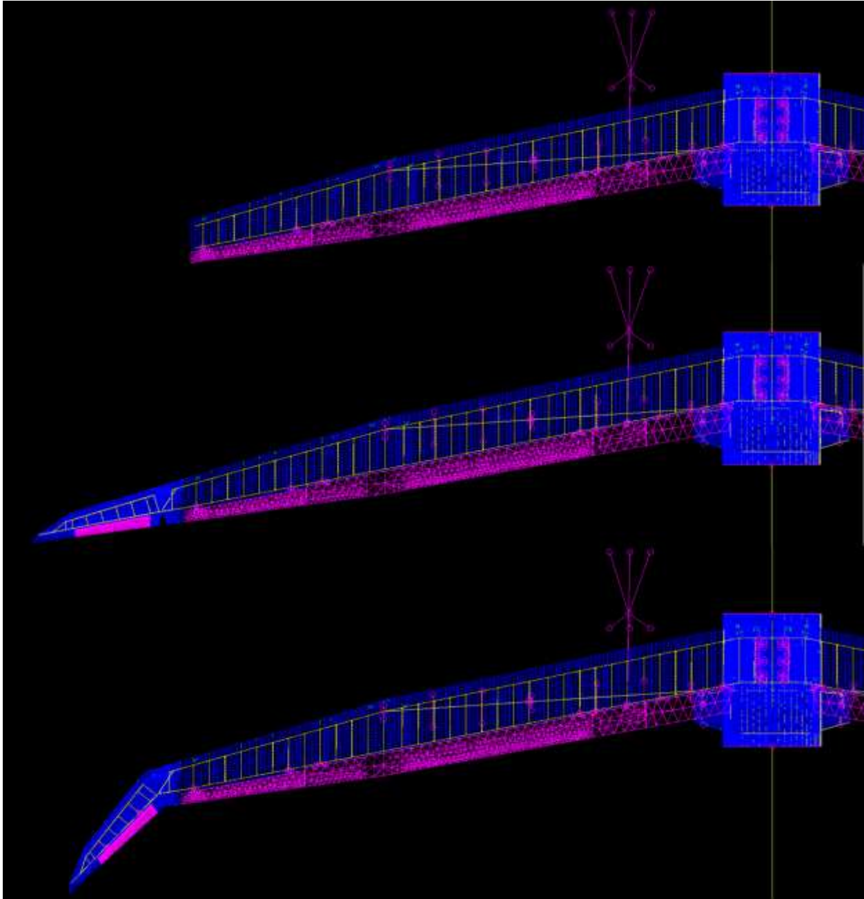
Figure 108. Top-level view of the baseline SUGAR PATRAN model (top) and integrated VGRWT/SUGAR model in the unswept 0 degree (middle) and fully swept 35 degree (bottom) positions.
