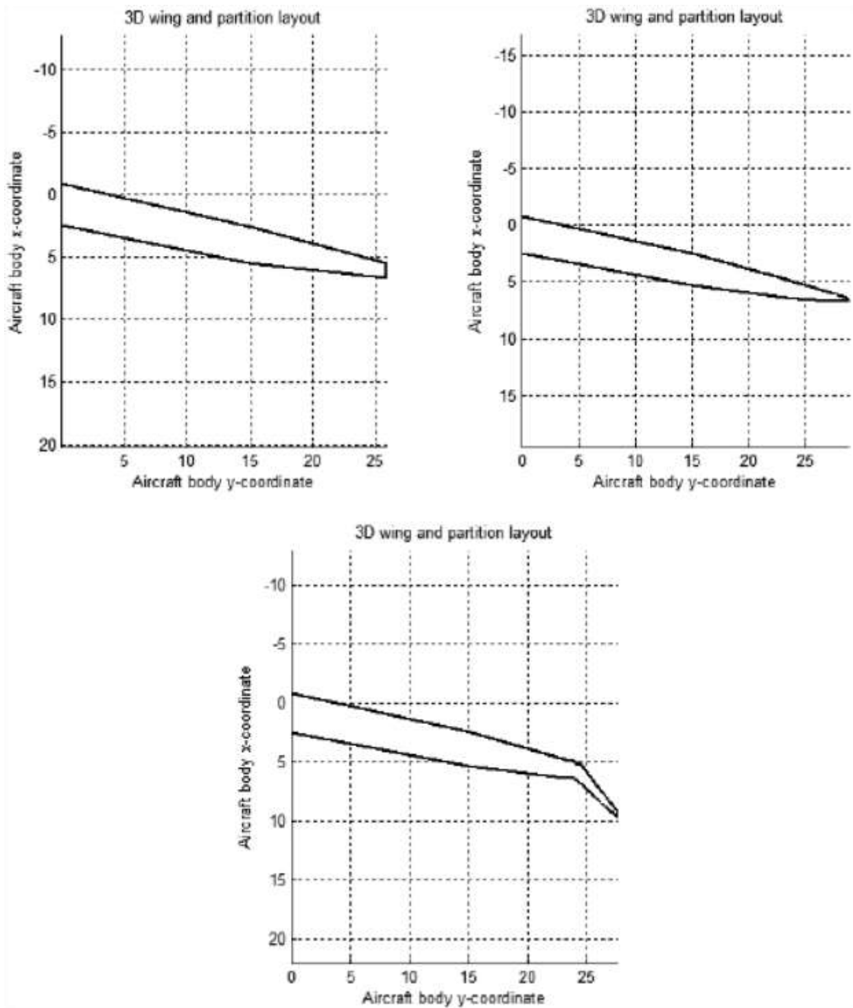
Figure 63. Tornado Clean Wing Models (Half Span Only, Dimensions in Meters)
