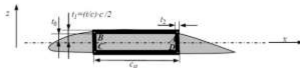
Figure 46. Graphic from MDO Paper Explaining Wing Box Geometry
