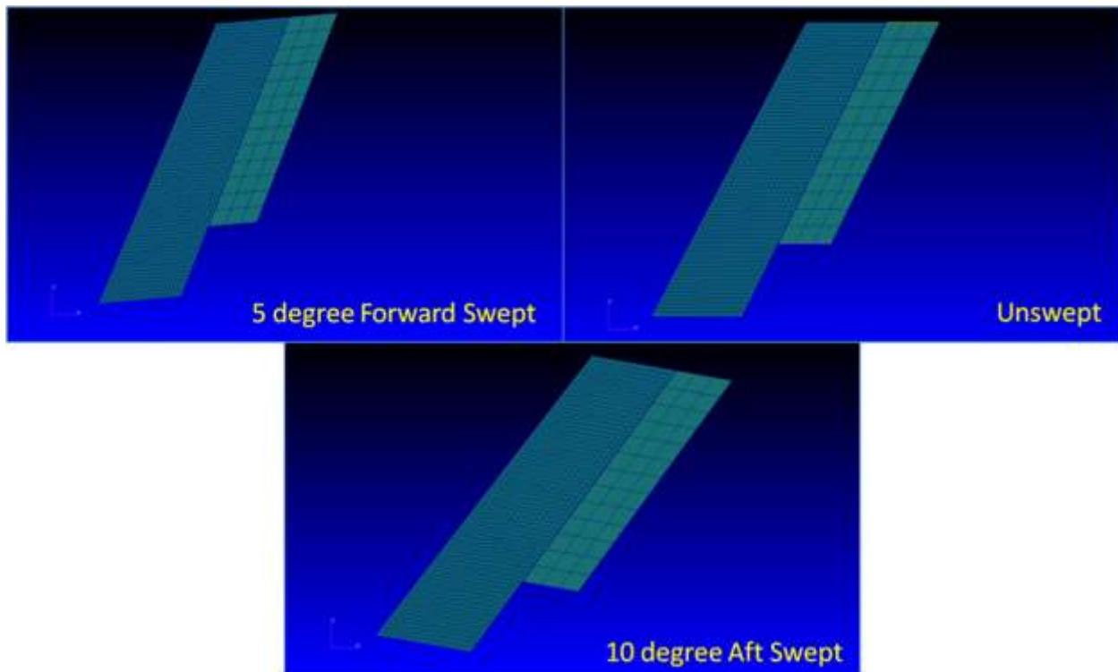
Figure 146. Model of NCE in 3 Different Configurations
