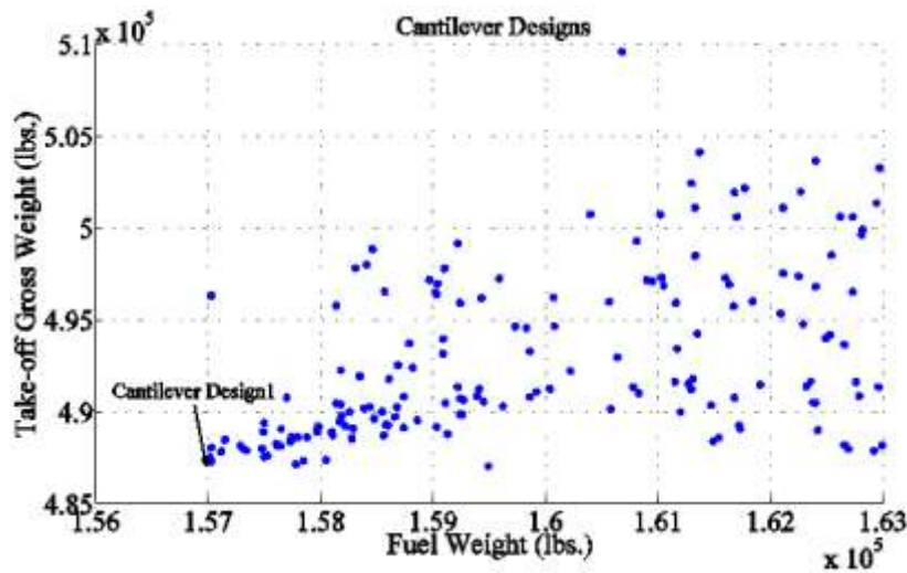
Figure 22. Cantilever Designs Obtained without NCE Tip
