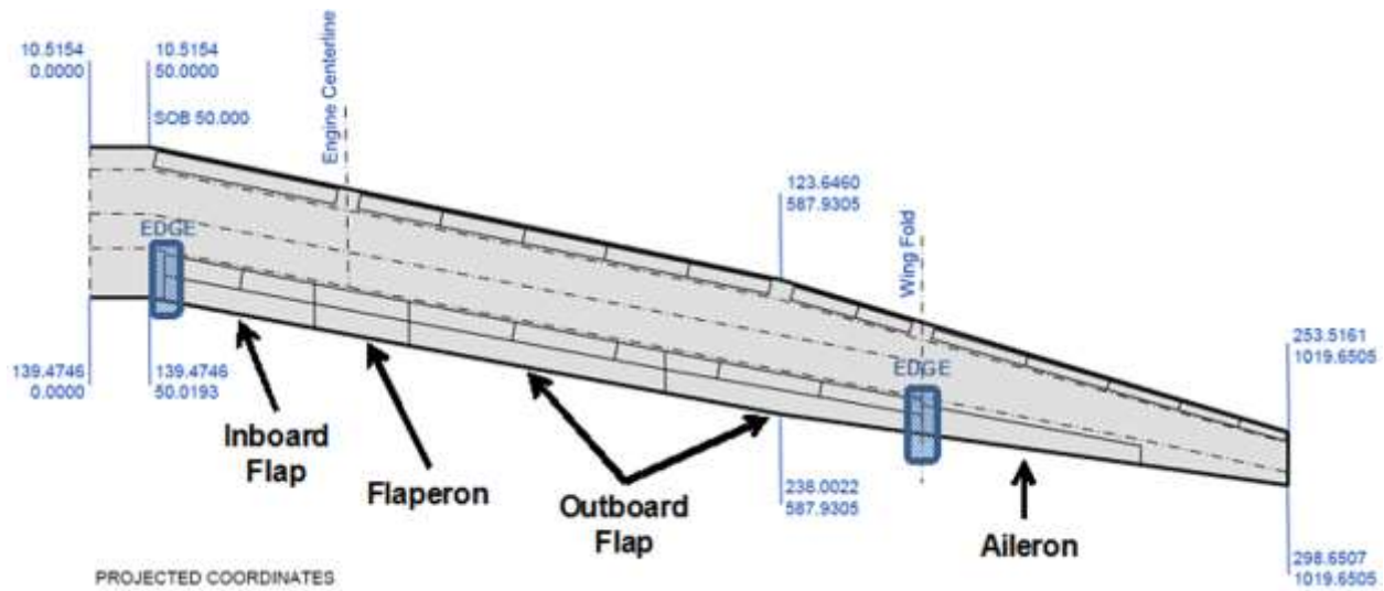
Figure 99. SUGAR Flap System Definition for Noise Analysis
