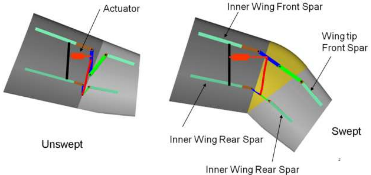
Figure 13. Multi-Pivot Geometry for Effective Pivot at Trailing Edge
