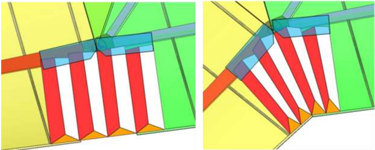
Figure 16. Flexible trailing edge fairing concept for VGRWT in unswept (left) and swept (right) conditions.
