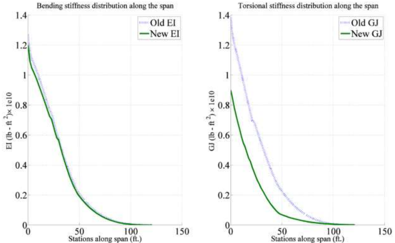
Figure 25. Bending and Torsional Stiffness Distribution for a Cantilever Design with Old and New Structural Models
