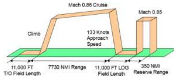
Figure 20. "777-like" Vehicle Flight Mission
