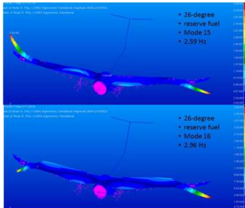
Figure C-18. Reserve-fuel: Structural mode 15 and 16 for 26-deg NCE.
