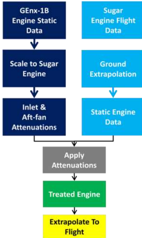
Figure 103. Process for Derivation of SUGAR Treated Engine Noise
