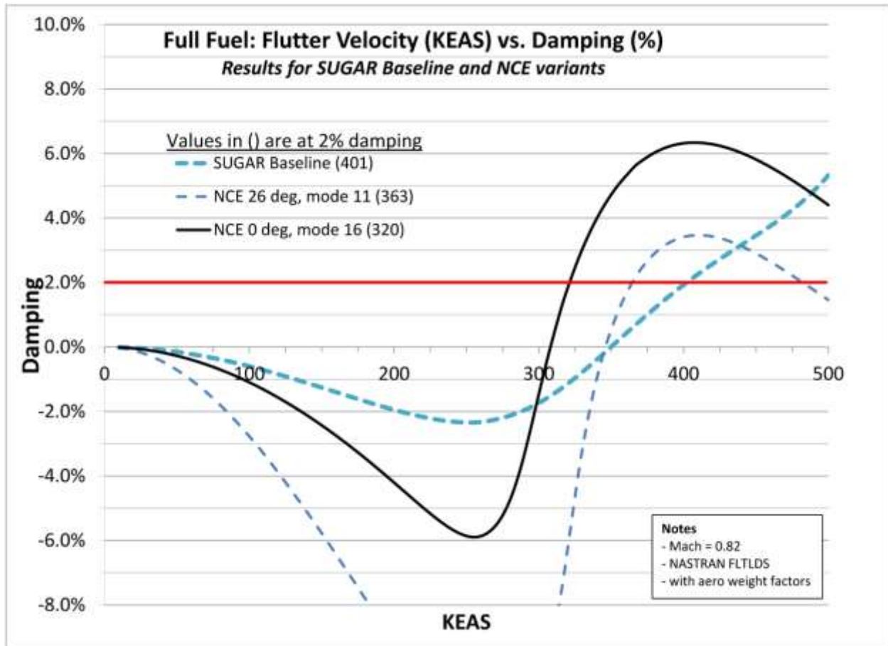
Figure 119. The V-G plot of the critical flutter mode for the full fuel case. Results are shown for the 0-degree and 26-degree NCE configurations as well as the baseline SUGAR aircraft.
