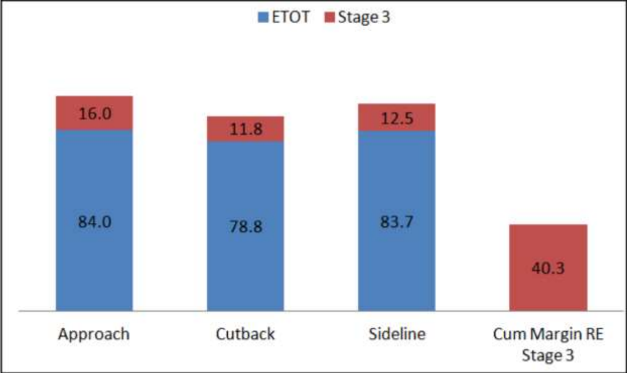
Figure 102. GE Hardwall Engine System Noise Assessment (without Airframe and Acoustic Liners)
