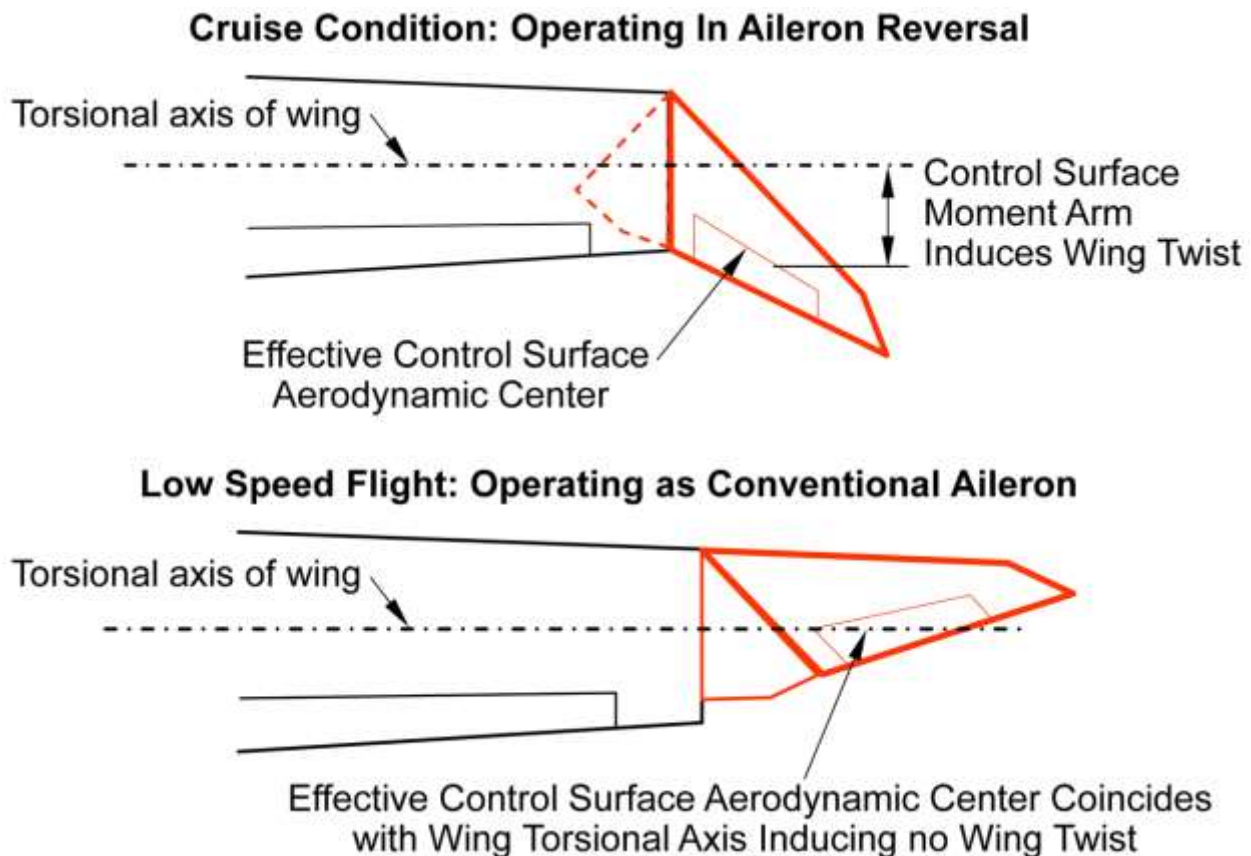
Figure 2. Variable Geometry Raked Wing Tip (VGRWT) Concept
