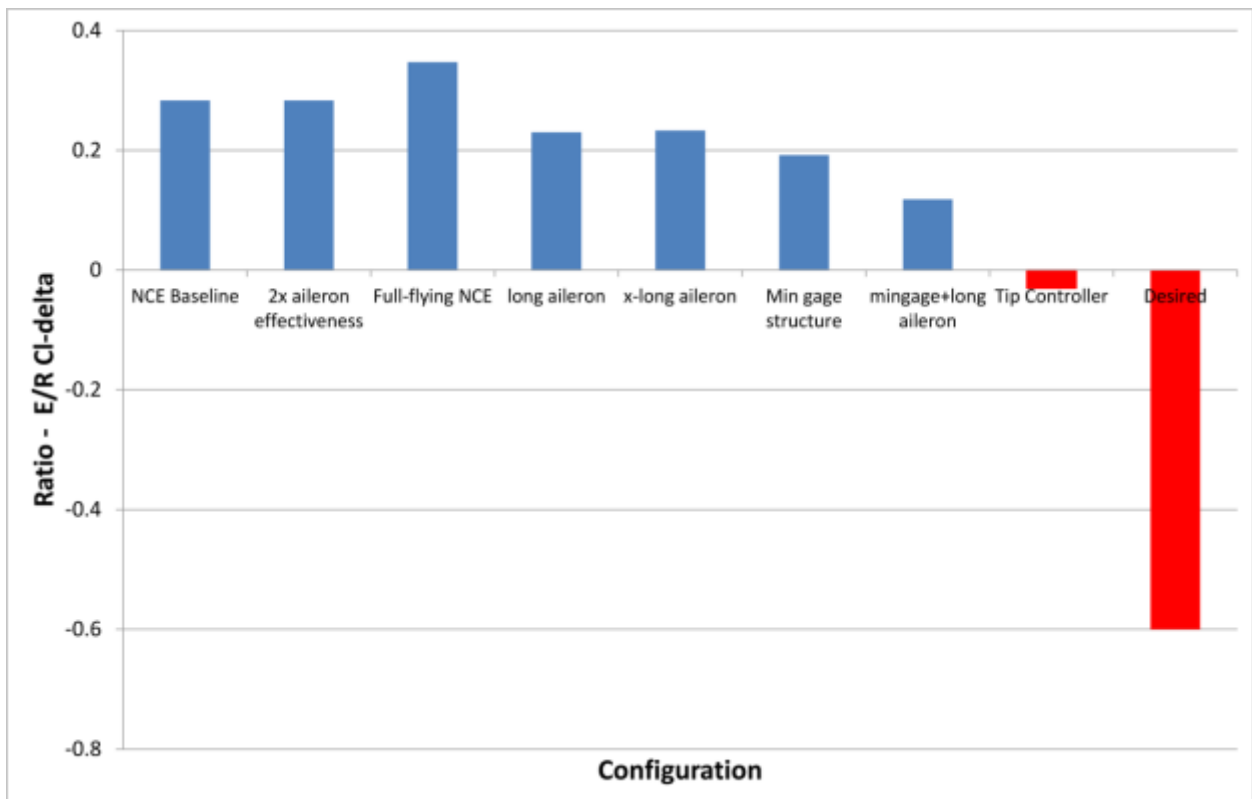
Figure 138. Several variations on the original NCE FEM were evaluated with the goal to achieve the desired role-rate acting in roll reversal.
