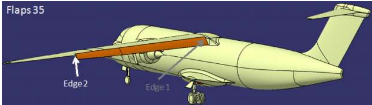
Figure 97. SUGAR Flap System Deployment at Approach
