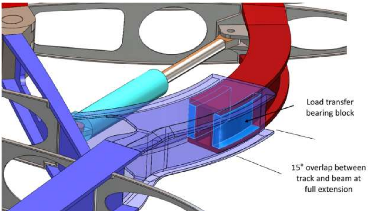
Figure 58. Forward Spar Track and Beam Mechanism (notional actuator shown)
