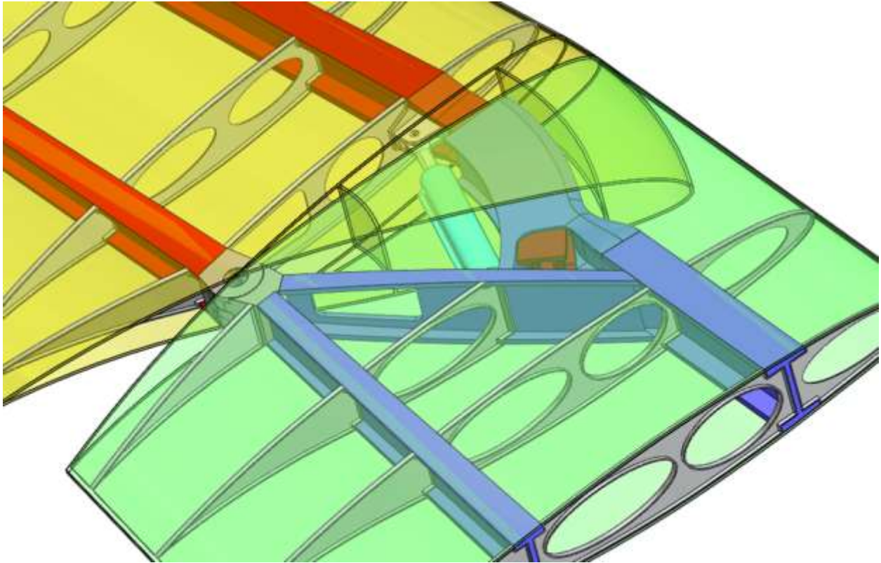
Figure 57. Mechanization Concept Details (aft fairing not shown)
