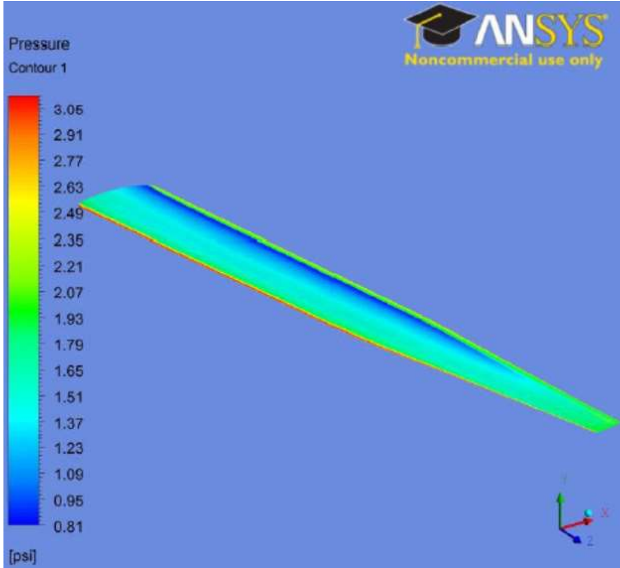
Figure 72. Fluent Prediction of Top Surface Pressure Contours of Baseline SUGAR Main Wing
