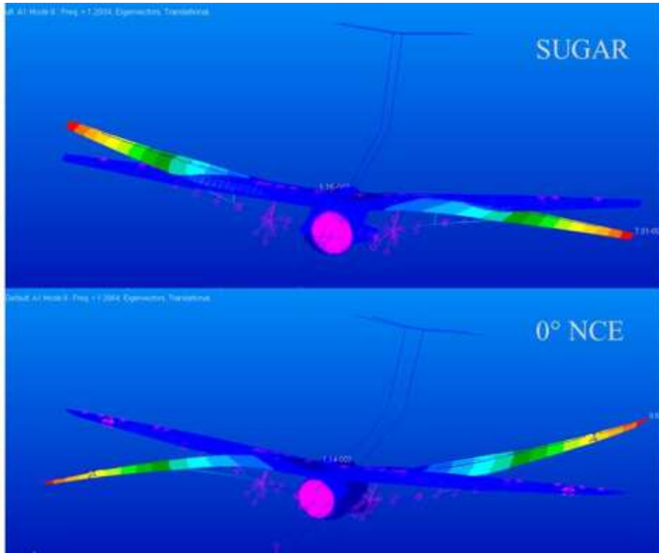
Figure C-3. Full-fuel: Structural mode 9 for baseline SUGAR (1.20 Hz) and 0-deg NCE (1.21) Hz.
