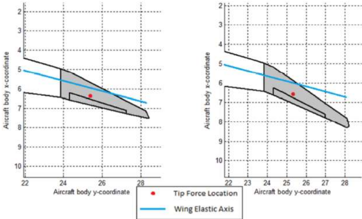
Figure 77. Baseline SUGAR Tip (Left) and Unswept VGRWT/NCE Tip (Right) Force Location (Dimensions in Meters)
