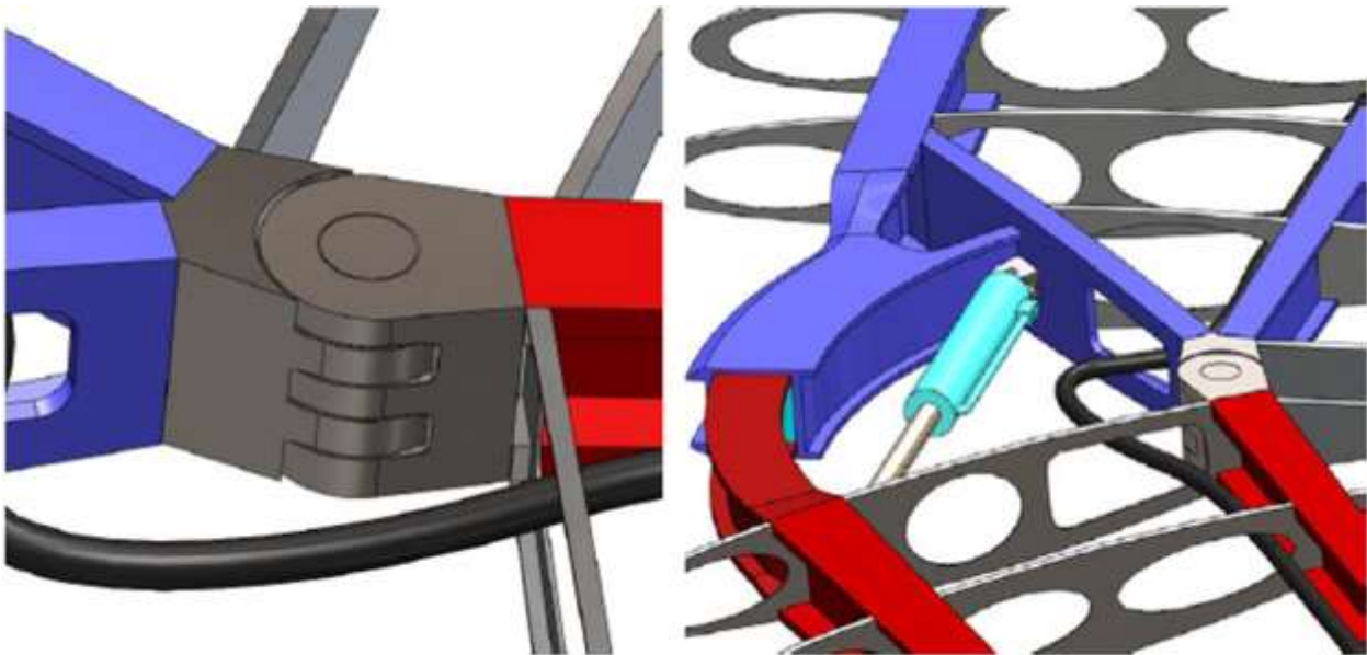
Figure 37. Rear spar pivot block (left) and cross spar (right).
