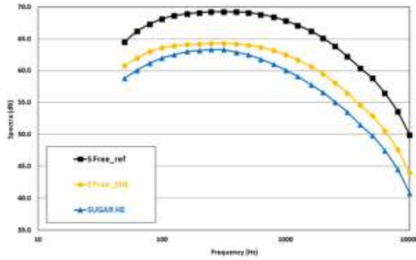
Figure 93. SUGAR Free vs. SUGAR Total Gear Noise Comparison at Approach
