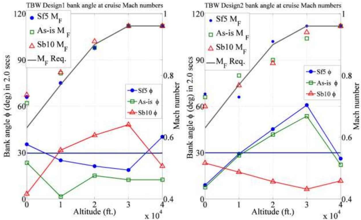
Figure 31. Bank angle achieved by TBW Design 1 and Design 2 in 2.0 seconds with the NCE tip at various altitudes but only at cruise Mach numbers and flutter Mach numbers at these altitudes.
