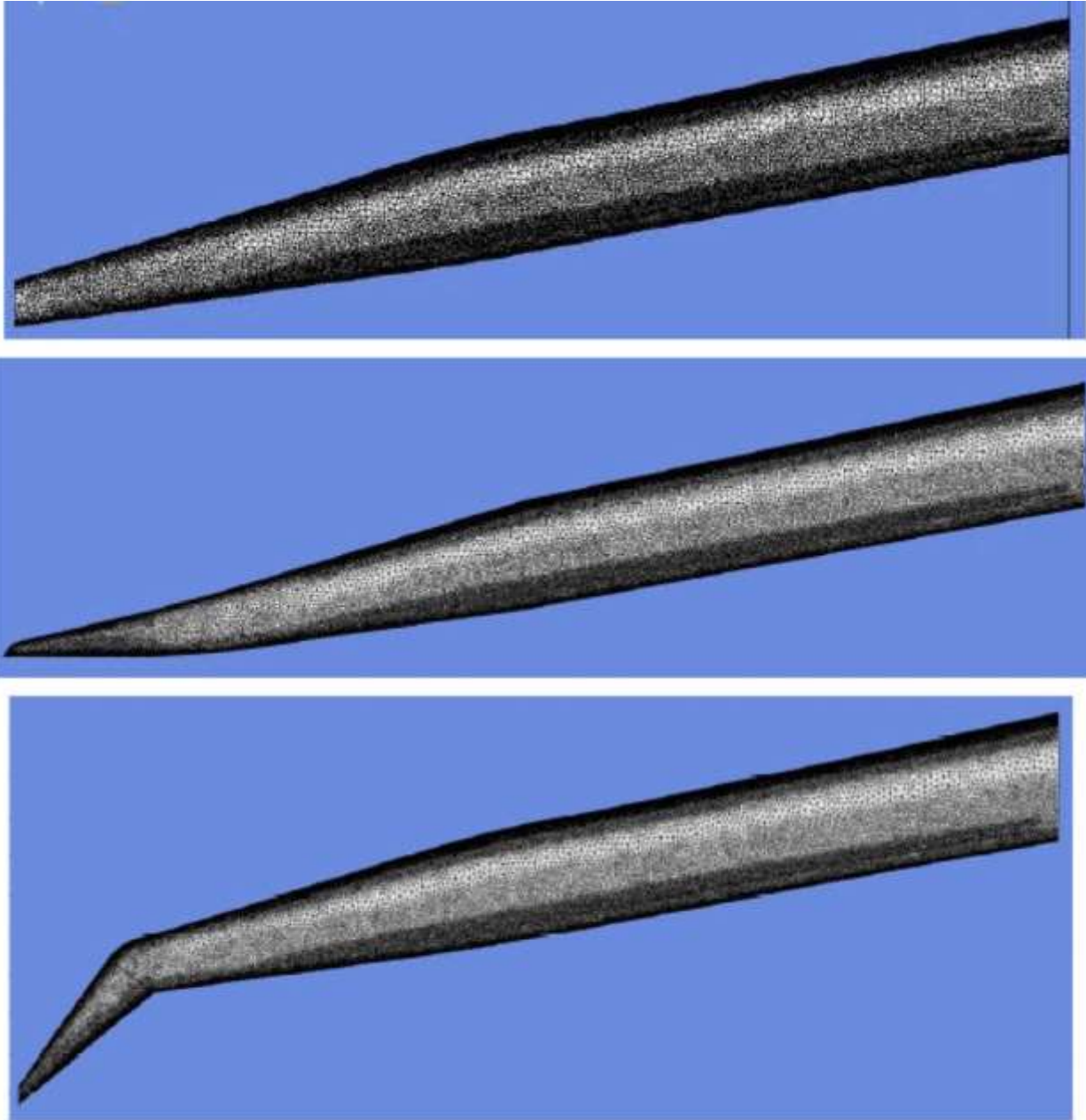
Figure 64. Fluent Clean Wing Models before Adaptation Top: Baseline SUGAR Main Wing Middle: SUGAR Wing with Unswept VGRWT/NCE Tip Bottom: SUGAR Wing with Fully-Swept VGRWT/NCE Tip
