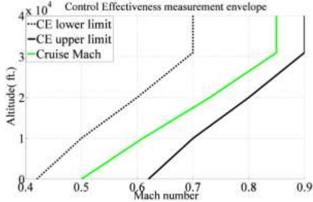
Figure 19. Control Effectiveness measurement envelope for "777-like" aircraft
