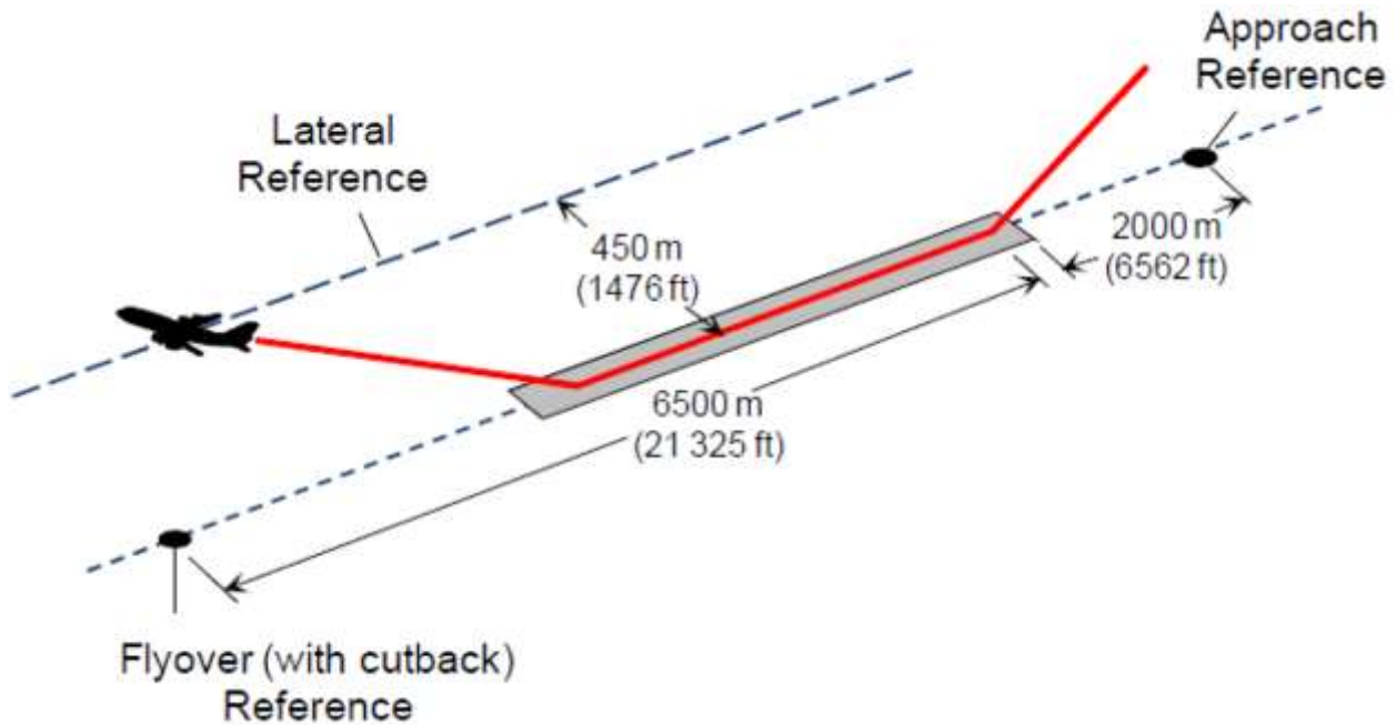
Figure 86. FAR 36 Noise Profile
