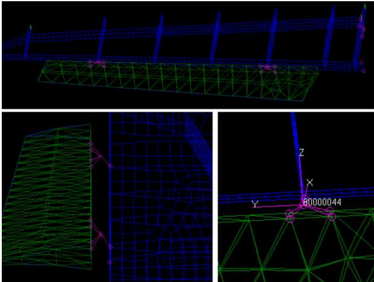
Figure 113. RBE2 Elements (pink) Modeling the Aileron Hinges (top, bottom left) and the Local Coordinate System Defining the Hinge Axis and MPC Constraints
