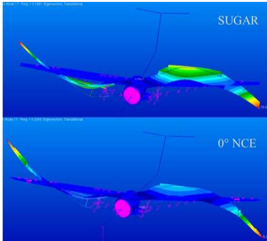
Figure C-11. Full-fuel: Structural mode 17 for baseline SUGAR (3.20 Hz) and 0-deg NCE (3.23) Hz
