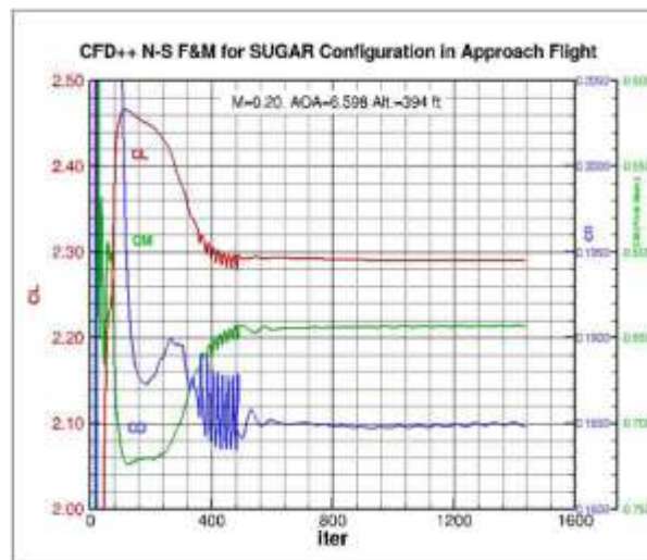
Figure 90. CFD++ Solution Convergence
