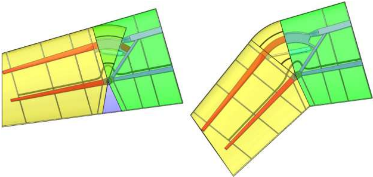
Figure 107. Simplified kinematic model of the variable geometry raked wingtip kinematic developed in Task 3.0 in fully unswept 0° (left) and fully swept 35° (right) sweep positions.
