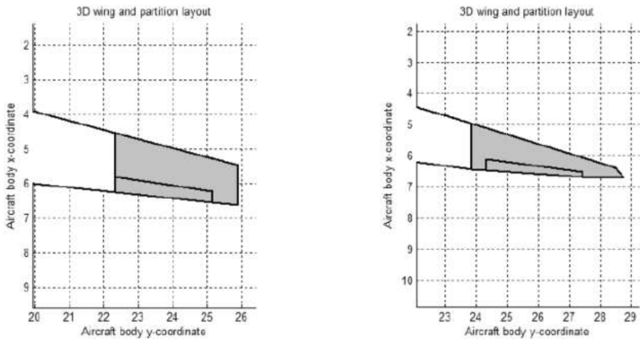
Figure 67. Baseline SUGAR (Left) and Unswept (Right) VGRWT/NCE Tip Details, Dimensions in Meters, Tip Areas for Comparison are Shaded
