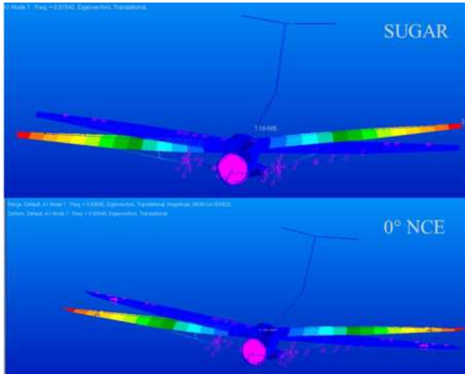
Figure C-1. Full-fuel: Structural mode 7 for baseline SUGAR (0.92 Hz) and 0-deg NCE (0.94) Hz.
