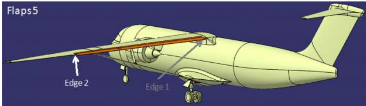
Figure 98. SUGAR Flap System Deployment at Cutback/Sideline
