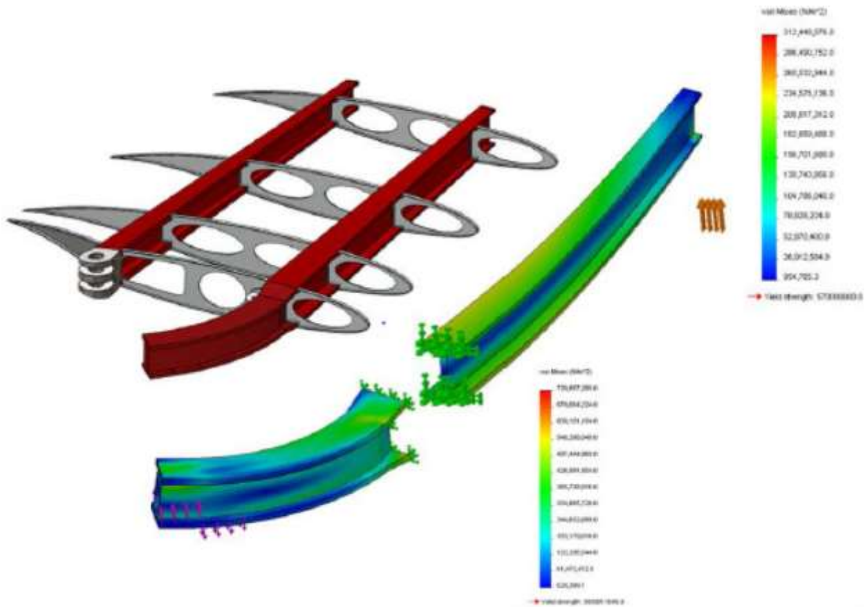
Figure 39. Component Level Sizing of Wingtip Forward Spar and Track
