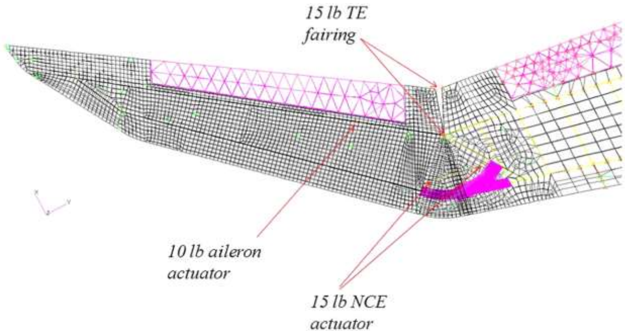
Figure 115. The important nonstructural masses were added to the FEM. The total planform weight of the NCE wingtip (structural + non-structural) was similar to the baseline sugar (10 psf).
