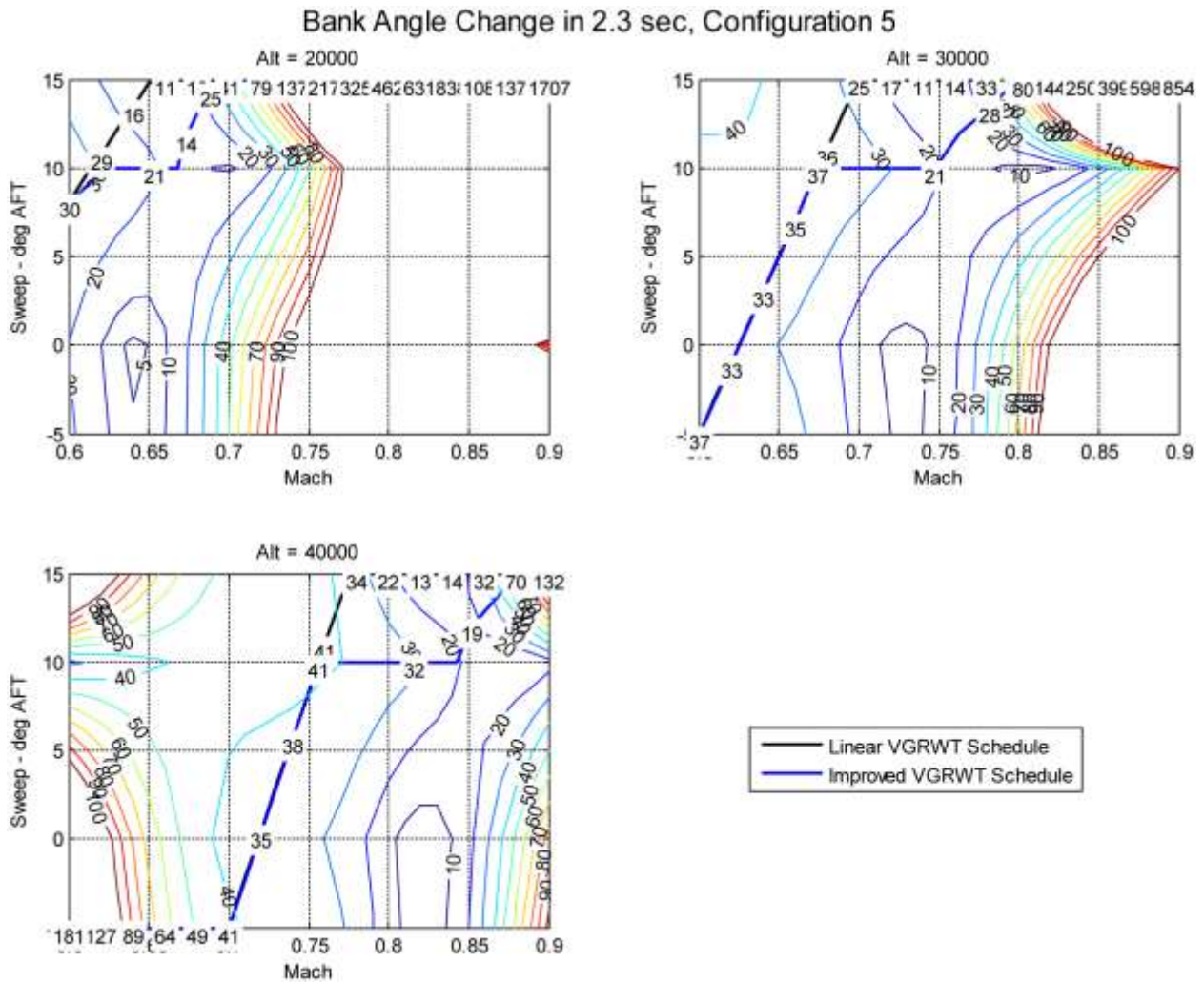
Figure 151. TBW Design 2 Bank Angle Change in 2.3 sec.
