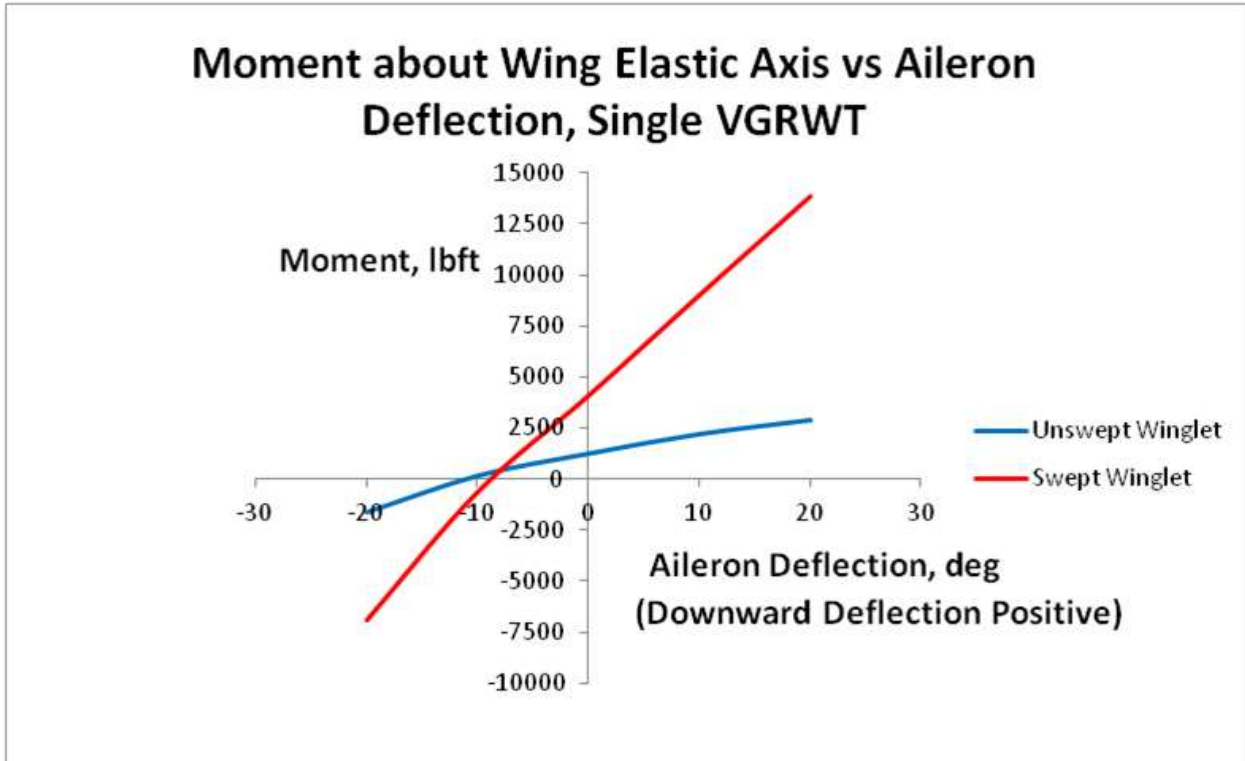
Figure 12. Moment about Wing Elastic Axis vs. Aileron Deflection, Single Wingtip
