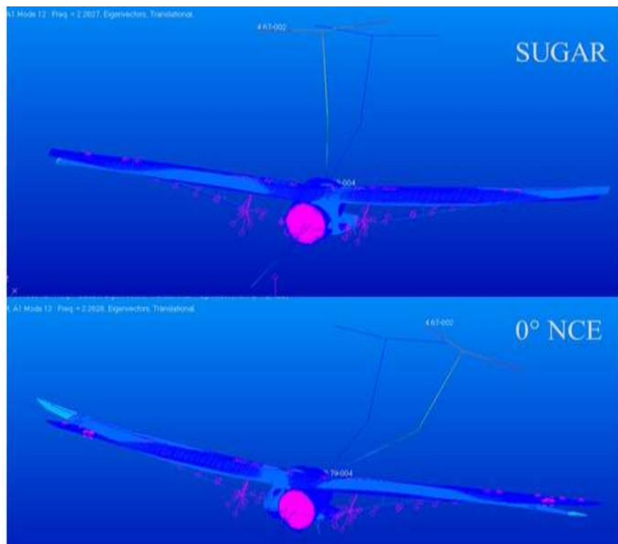
Figure C-6. Full-fuel: Structural mode 12 for baseline SUGAR (2.26 Hz) and 0-deg NCE (2.26) Hz.
