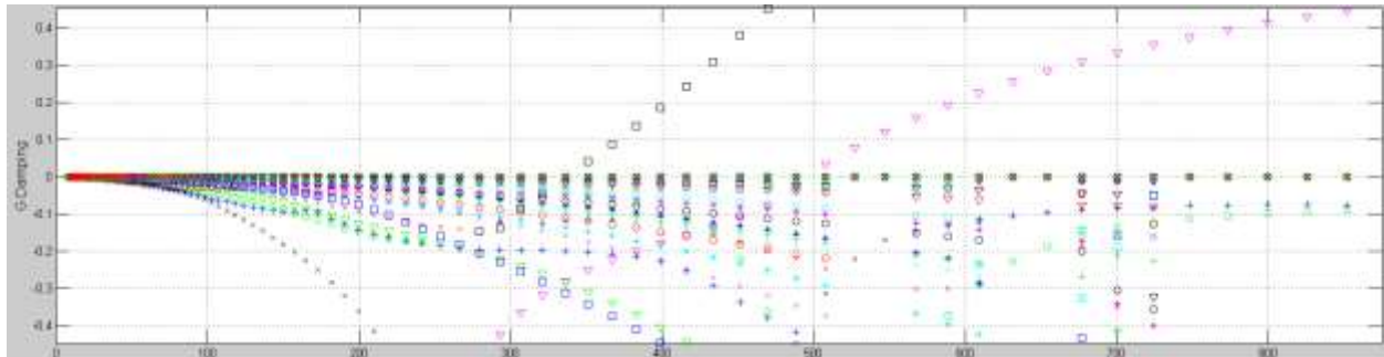
Figure 142. V-G Diagram of Half Span Model
