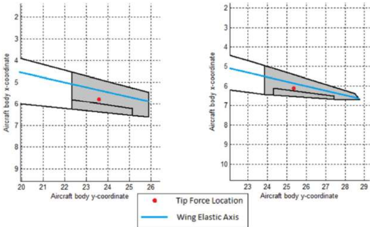
Figure 78. Quarter-Sweep VGRWT/NCE Tip (Left) and Half-Sweep VGRWT/NCE Tip (Right) Force Location (Dimensions in Meters)
