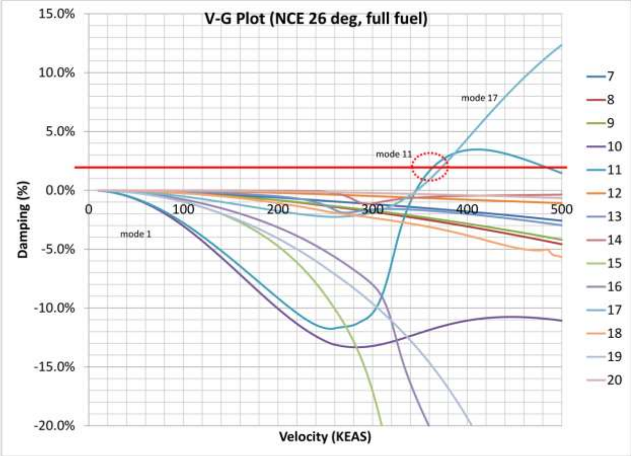
Figure 125. V-G plot for NCE 26-degree full fuel case.
