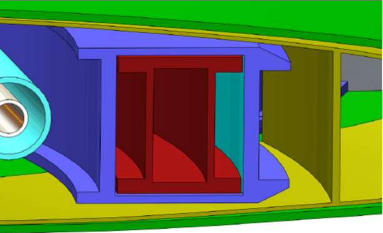
Figure 36. Cross section of nested track and beam structure showing the fixed structures (wing root track, blue; root wing skin, green) and moving structures (wingtip beam, red; wingtip forward fairing, yellow).
