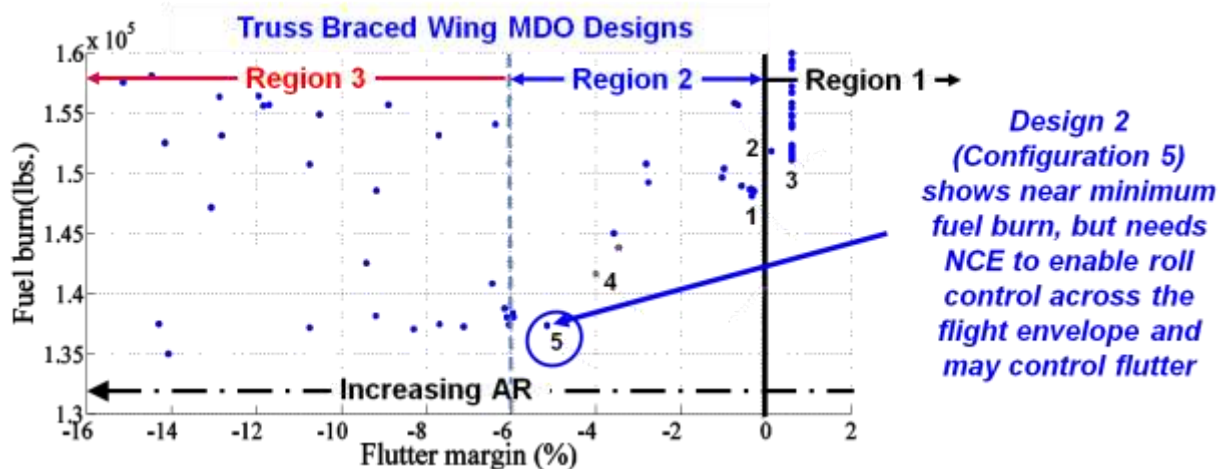
Figure 155. Key VT MDO Summarized Results for Dual-Aisle TBW Configuration
