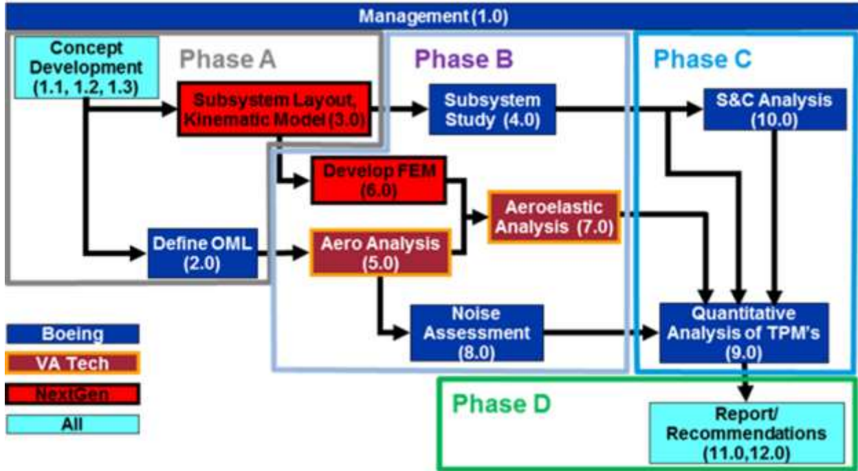
Figure 1. Novel Control Effector Program Plan
