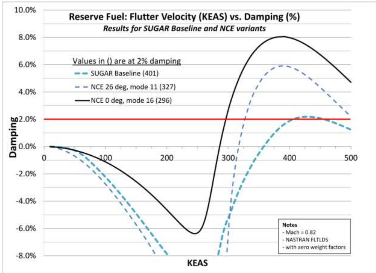
Figure 126. The V-G plot of the critical flutter mode for the reserve fuel case. Results are shown for the 0-degree and 26-degree NCE configurations as well as the baseline SUGAR aircraft.
