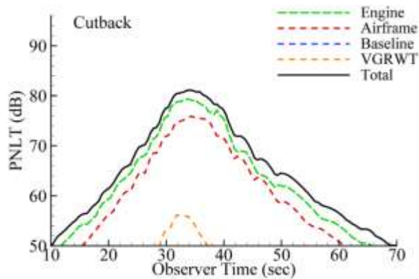
Figure 105. SUGAR/RGWRT Cutback Aircraft Noise
