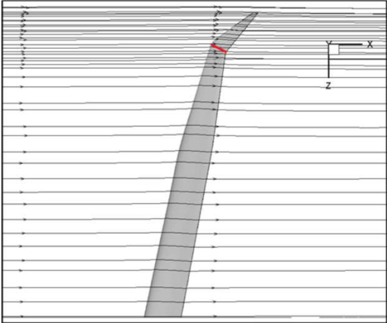
Figure 84. Fluent Prediction of Streamlines over Step for Fully-Swept VGRWT/NCE Tip (Step Drawn in Red)
