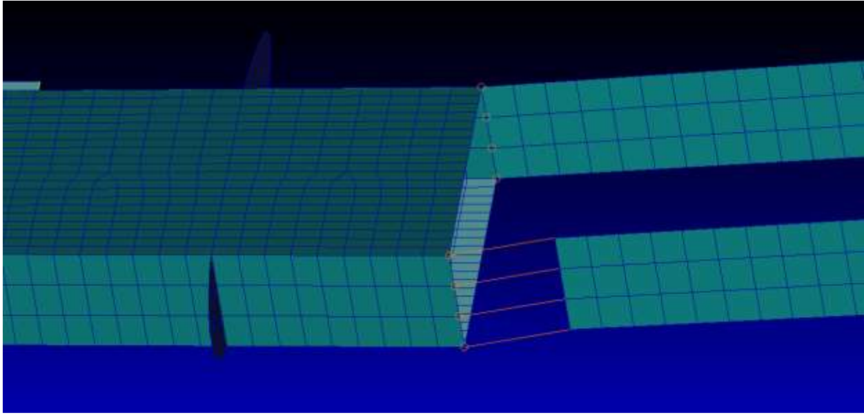
Figure 147. NCE to Wing Connectivity
