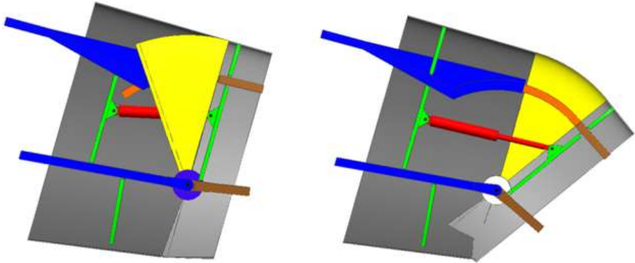
Figure 14. Aft Spar Pivot/Forward Spar Track/Rail Geometry
