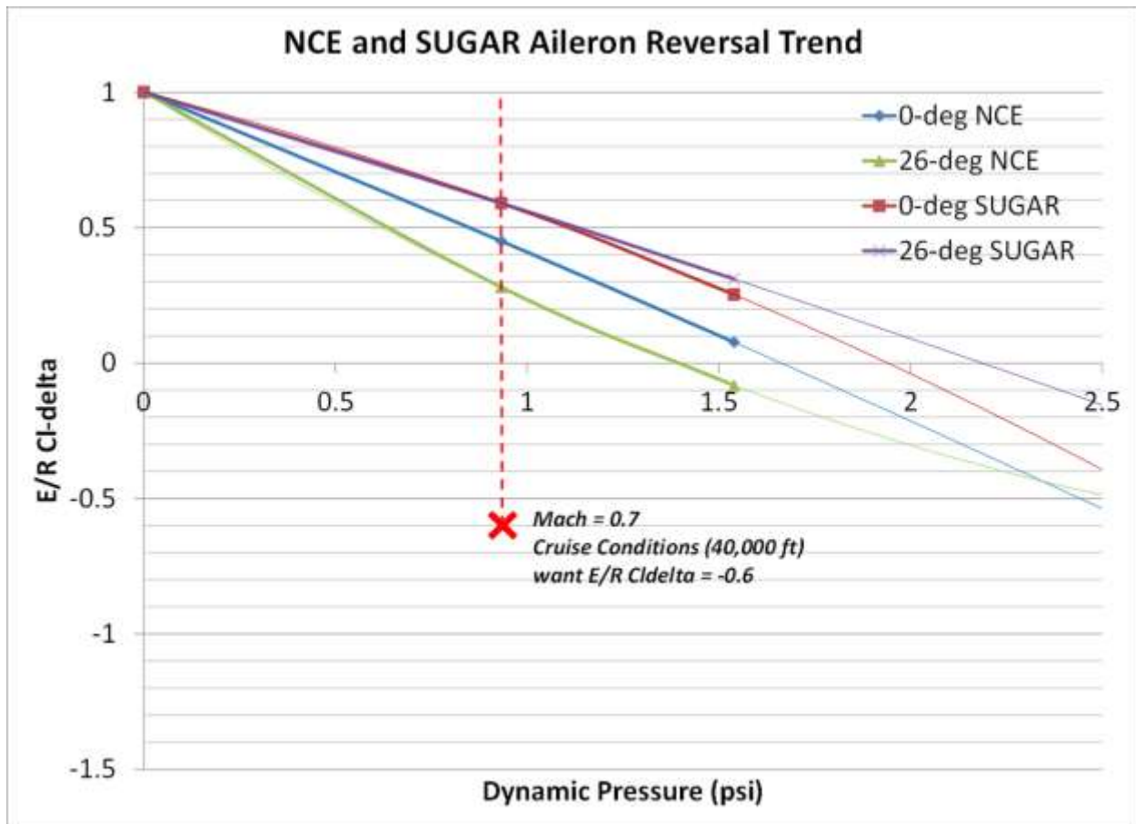
Figure 136. E/R C_{L\delta} vs. dynamic pressure for 0-degree and 26-degree NCE aircraft. Results are provided for control configurations using NCE aileron only, or SUGAR aileron only. Zero crossings indicate the dynamic pressure at which aileron reversal occurs. The desired value to achieve sufficient roll control at cruise condition, acting in aileron reversal, is -0.6.
