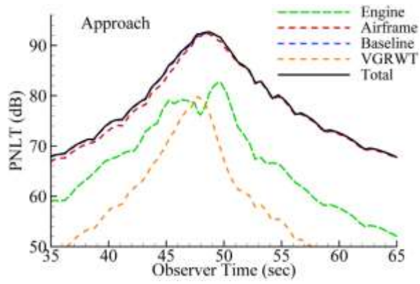
Figure 106. SUGAR/RGWT Approach Aircraft Noise
