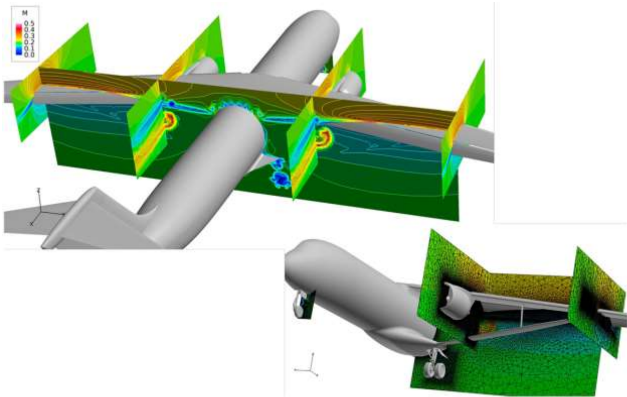
Figure 91. CFD++ Computed Mach Cuts
