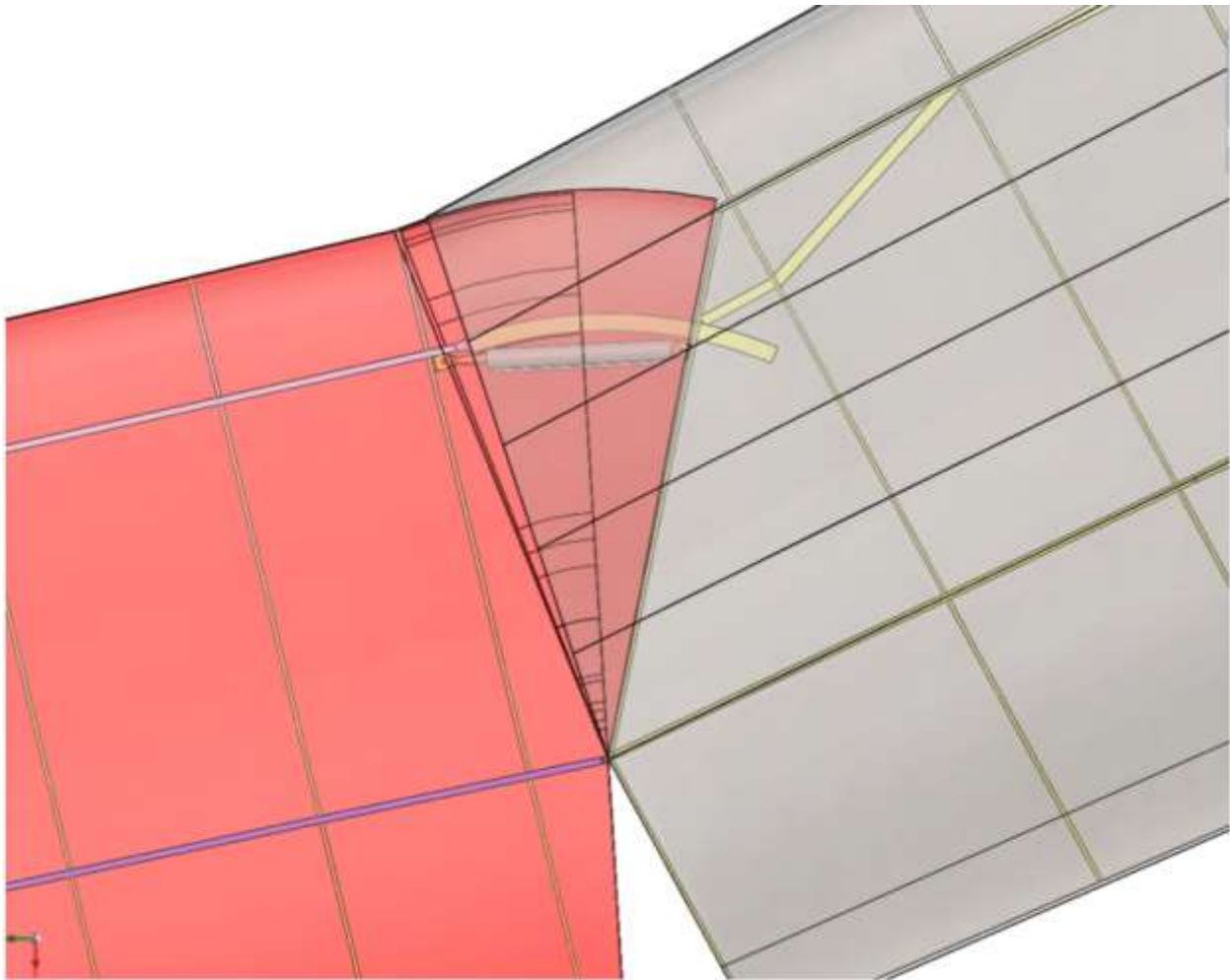
Figure 53. View of the NCE-Wing Joint Area with NCE Swept Forward 15°
