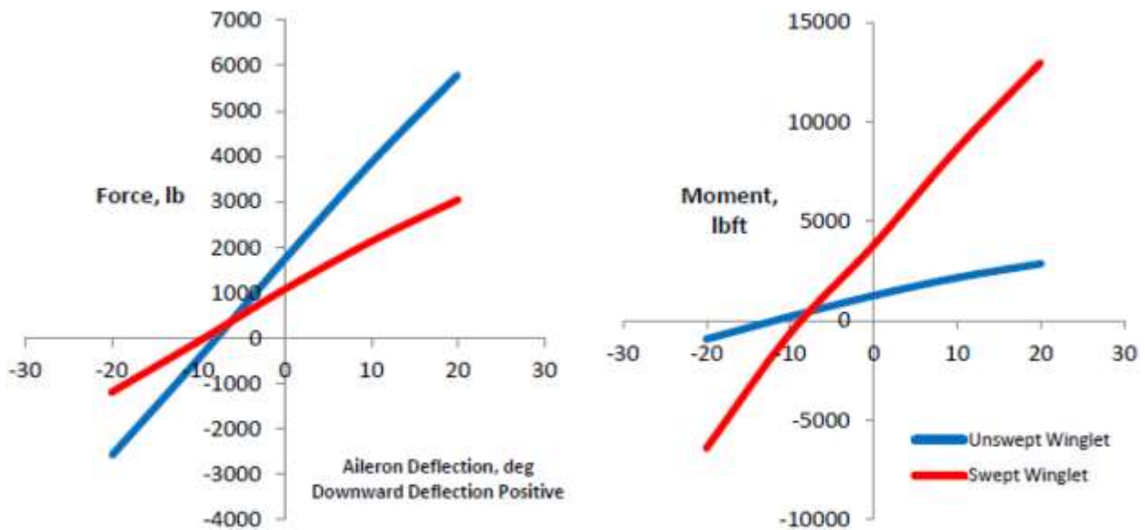
Figure 38. Tornado generated wingtip force and moment values with respect to aileron deflection.
