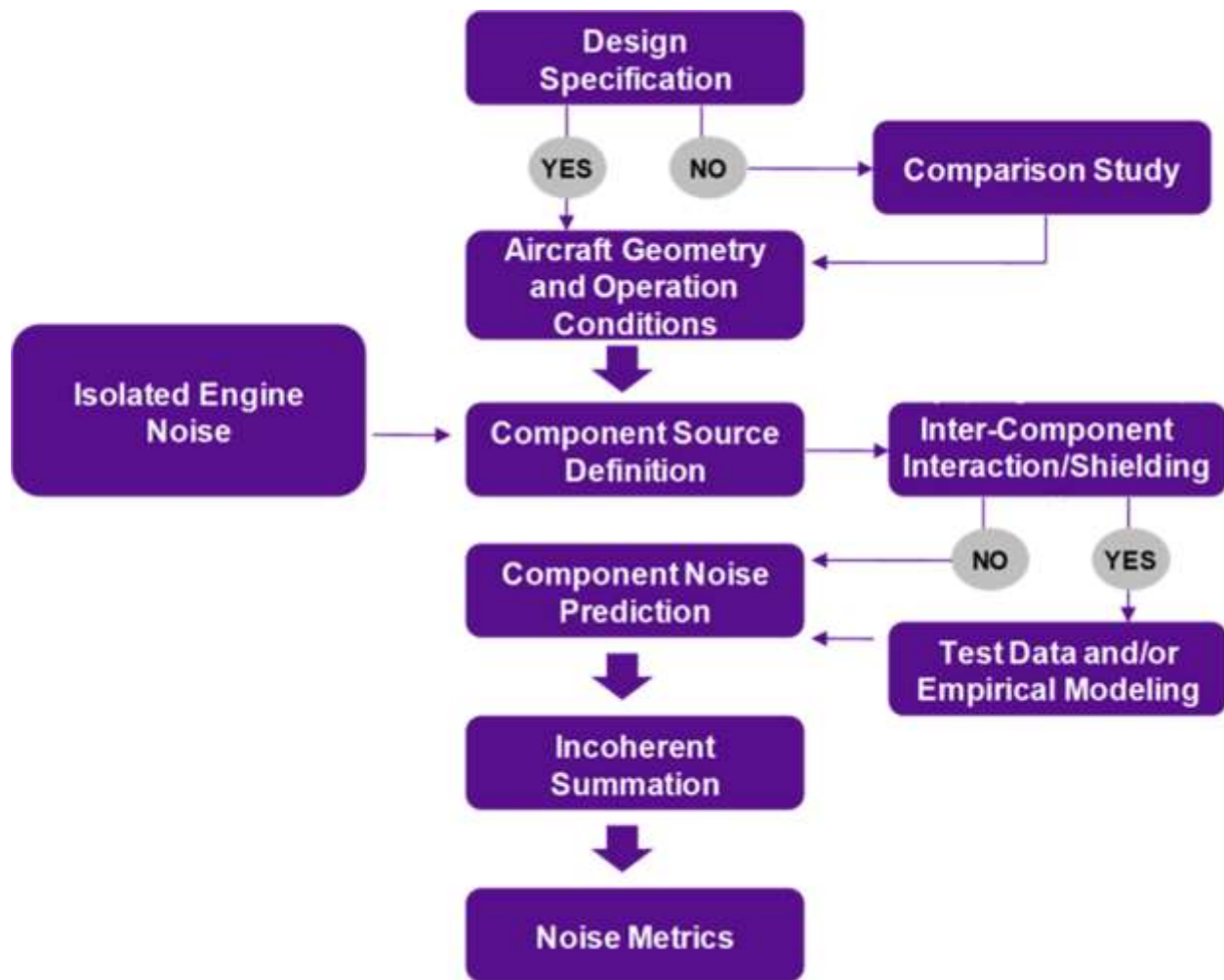
Figure 87. Overall Noise Analysis Process
