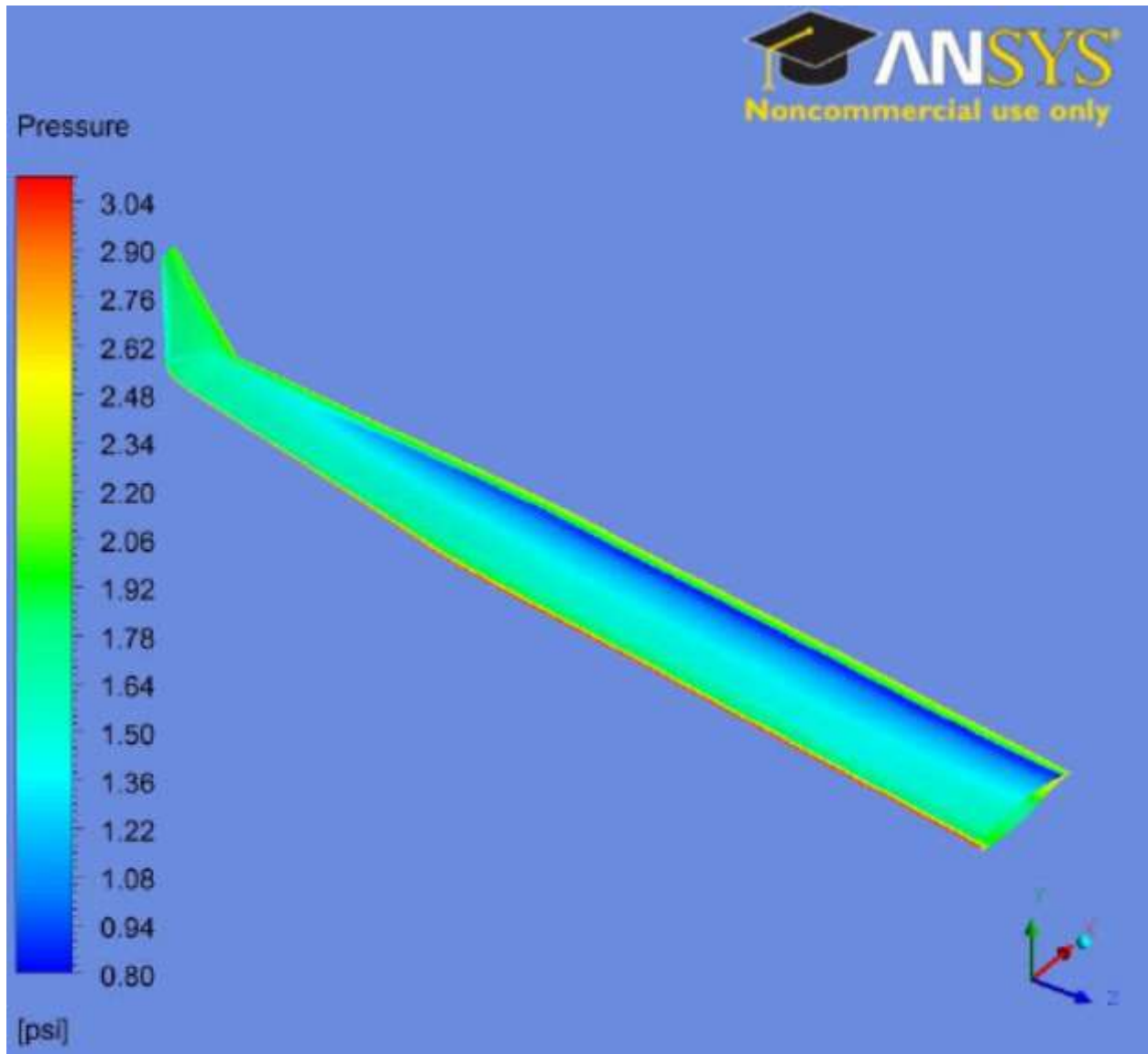
Figure 74. Fluent Prediction of Top Surface Pressure Contours of SUGAR Wing with Fully-Swept VGRWT/NCE Tip
