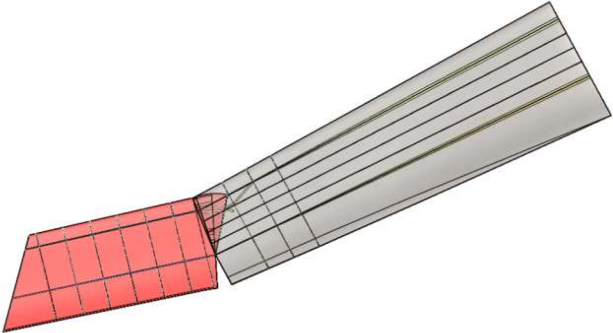
Figure 51. Wingtip with NCE Swept Forward 15°
