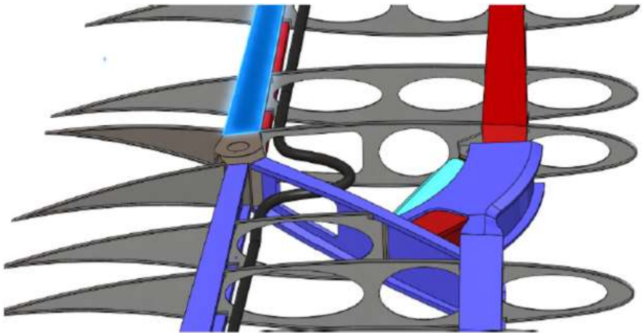
Figure 42. Space for electrical and hydraulic line routing with representative flexible line (black).
