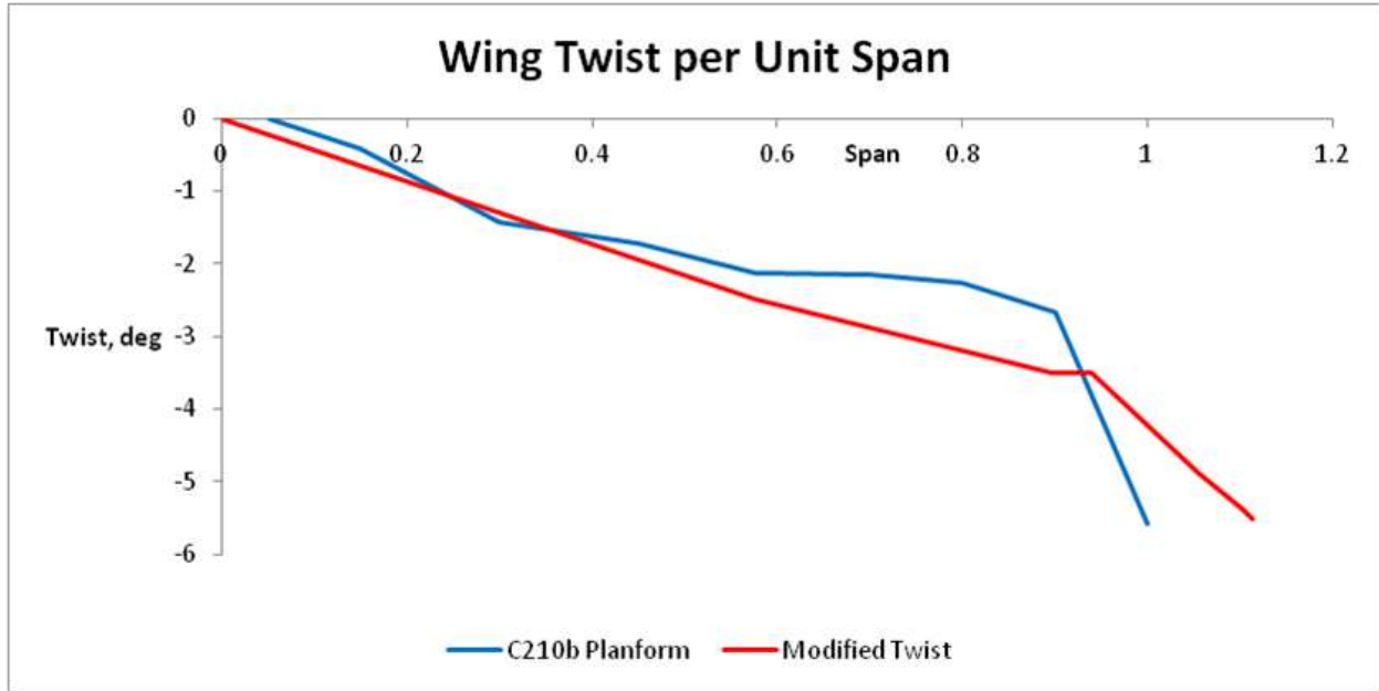
Figure 10. Twist per Unit Span
