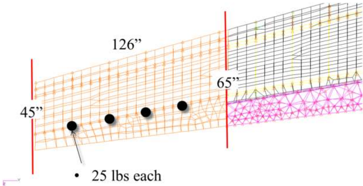
Figure 133. A study was conducted to evaluate the effect of an aft shift in the wing center of gravity on flutter speed. Ballast weight was added along the aileron hingeline.
