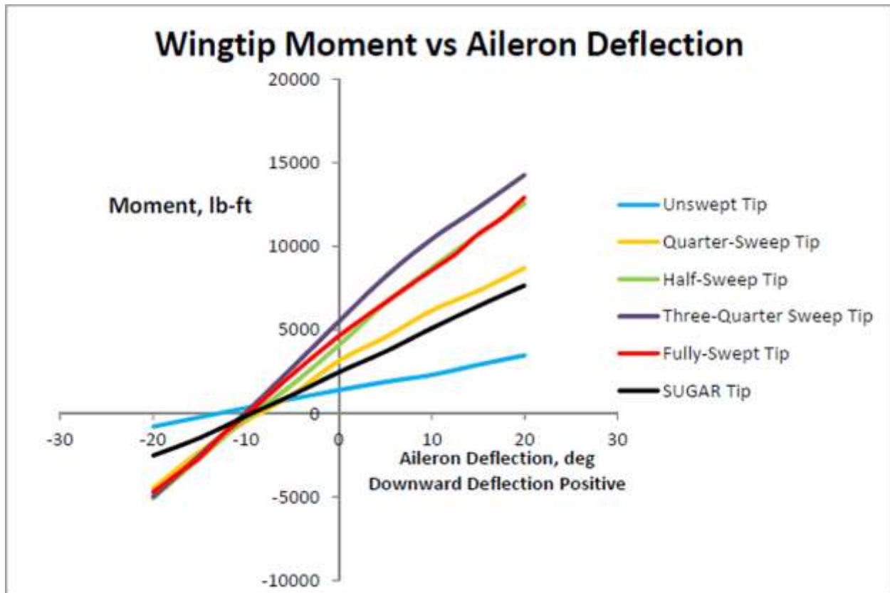
Figure 81. Wingtip Moment as a Function of Sweep and Aileron Deflection
