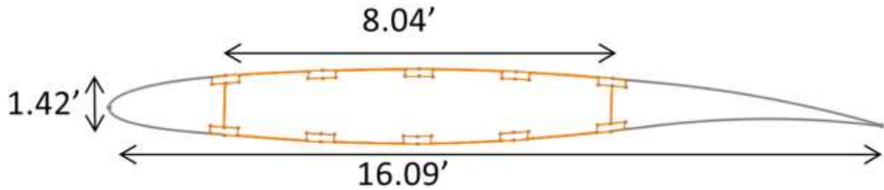
Figure 48. Sketch of Wing Box and Skin at node 27. The Wing Box is Highlighted.
