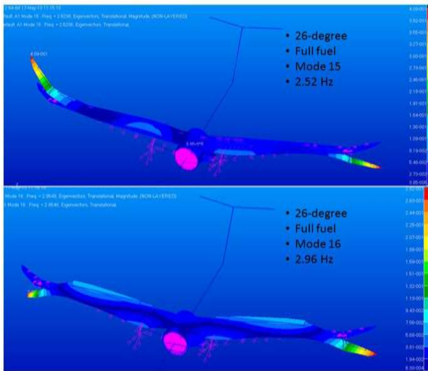
Figure C-16. Full-fuel: Structural mode 15 and 16 for 26-deg NCE.
