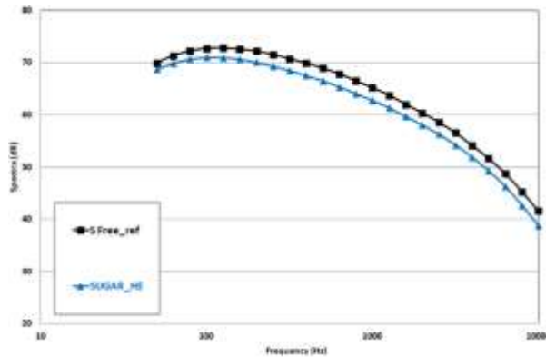
Figure 100. SUGAR Free vs. SUGAR Flap Noise Comparison at Approach
