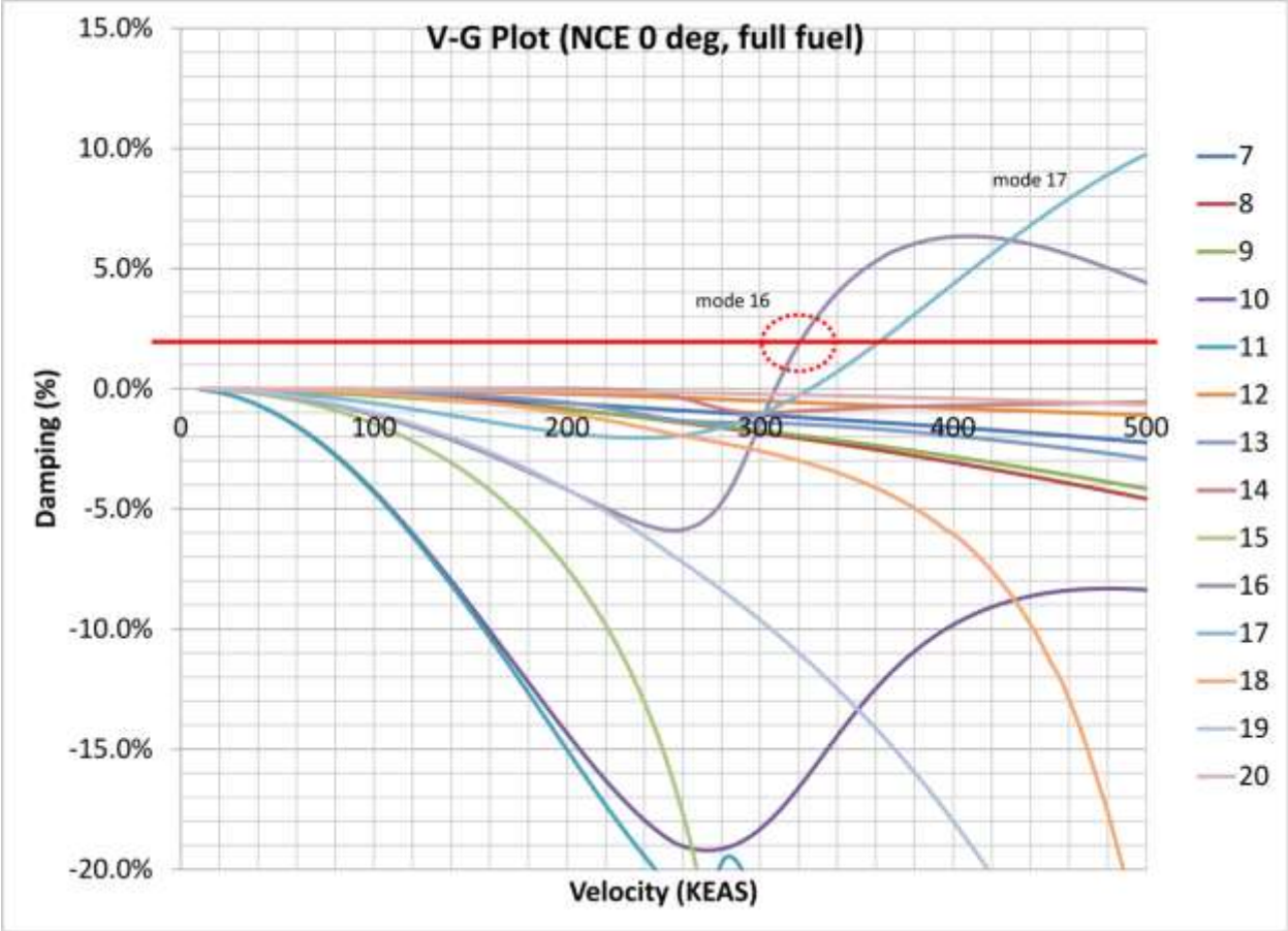
Figure 122. V-G plot for NCE 0-degree full fuel case.
