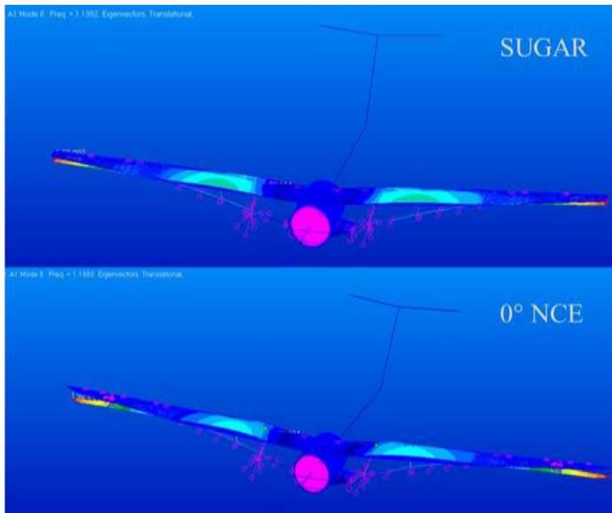
Figure C-2. Full-fuel: Structural mode 8 for baseline SUGAR (1.14 Hz) and 0-deg NCE (1.14) Hz.
