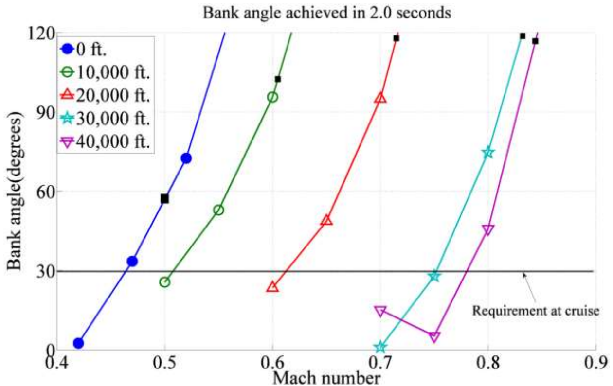
Figure 24. Bank Angles Achieved by Design 1 at Various Altitudes and Mach Numbers along Flight Path
