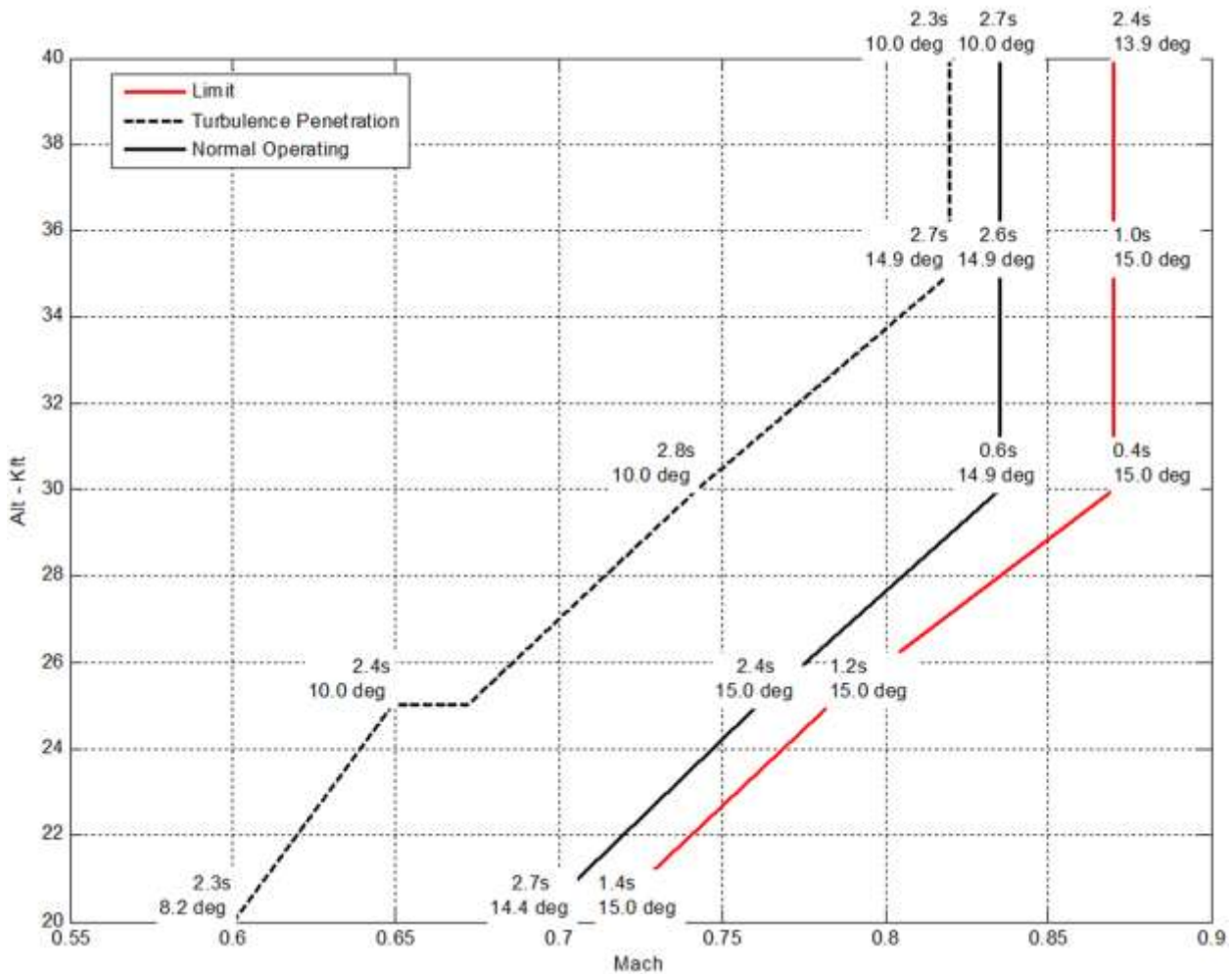
Figure 154. TBW Design 2 Representative Climb and Cruise Roll Performance.
