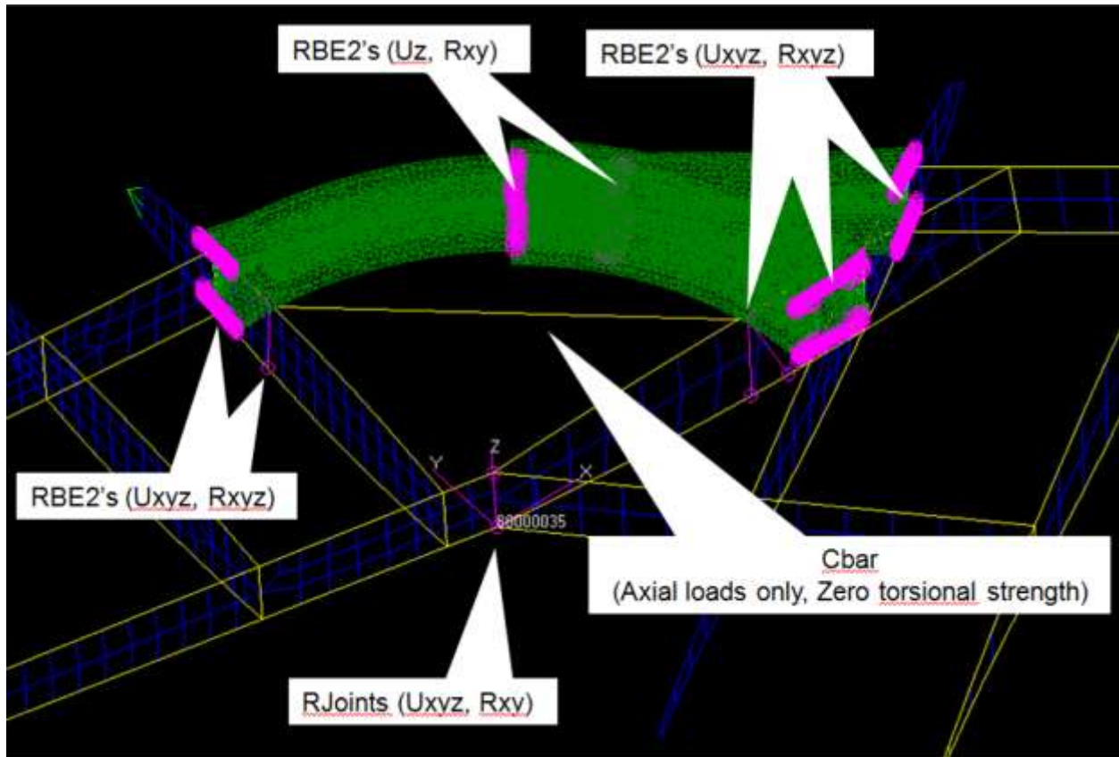
Figure 111. MPC elements used to model the track and beam interface, track and beam attachment points, rear pivot joint, and wingtip sweep actuator attachment points. Constrained degrees of freedom are listed for each element group and are referenced to the local coordinate system defining the wing sweep pivot axis.
