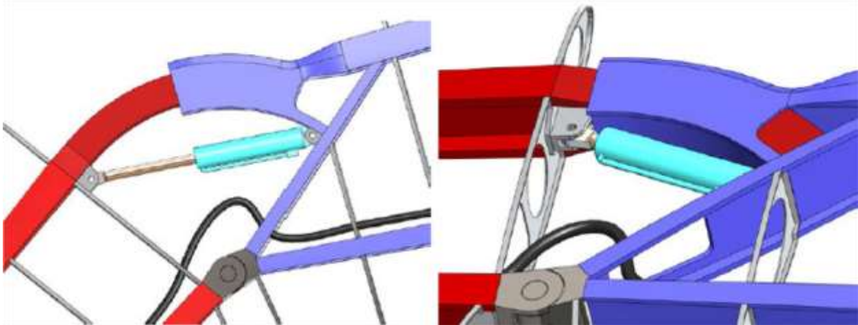
Figure 41. Representative actuator in the extended/swept (left) and retracted/unswept (right) positions.
