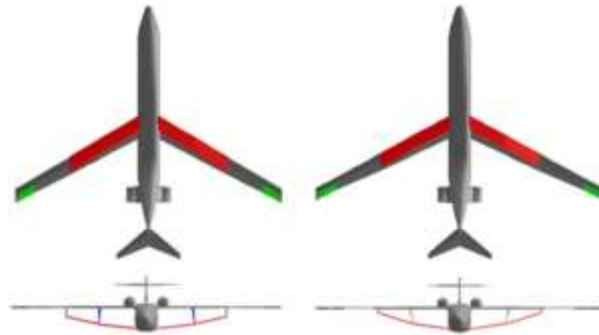
Figure 27. Selected TBW Designs: TBW Design 1(left) and TBW Design 2(right)
