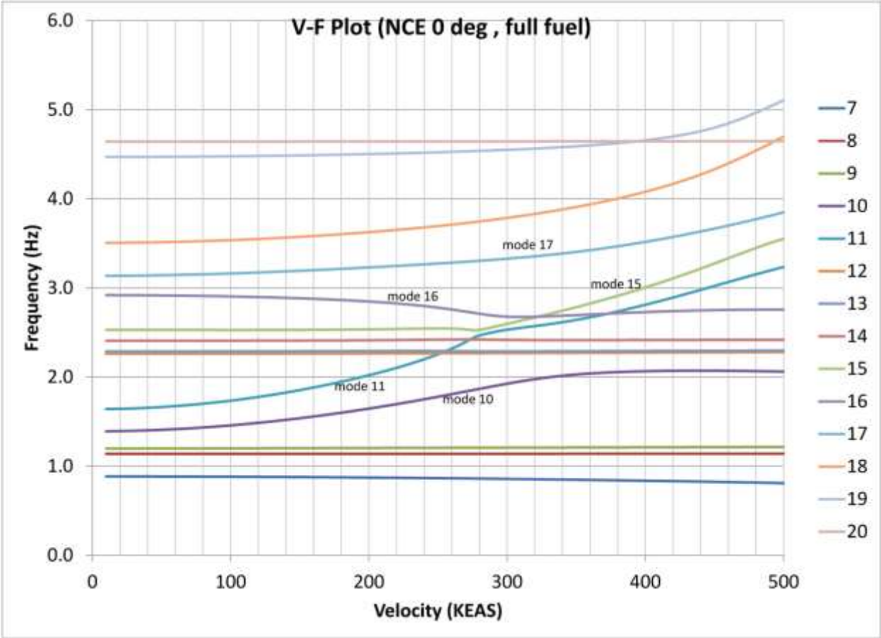
Figure 121. V-F plot for NCE 0-degree full fuel case.
