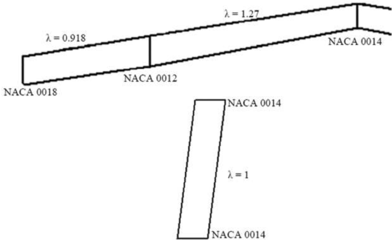
Figure 66. Details of Strut (Top) and Jury (Bottom) Tornado Models ( \lambda = taper ratio)
