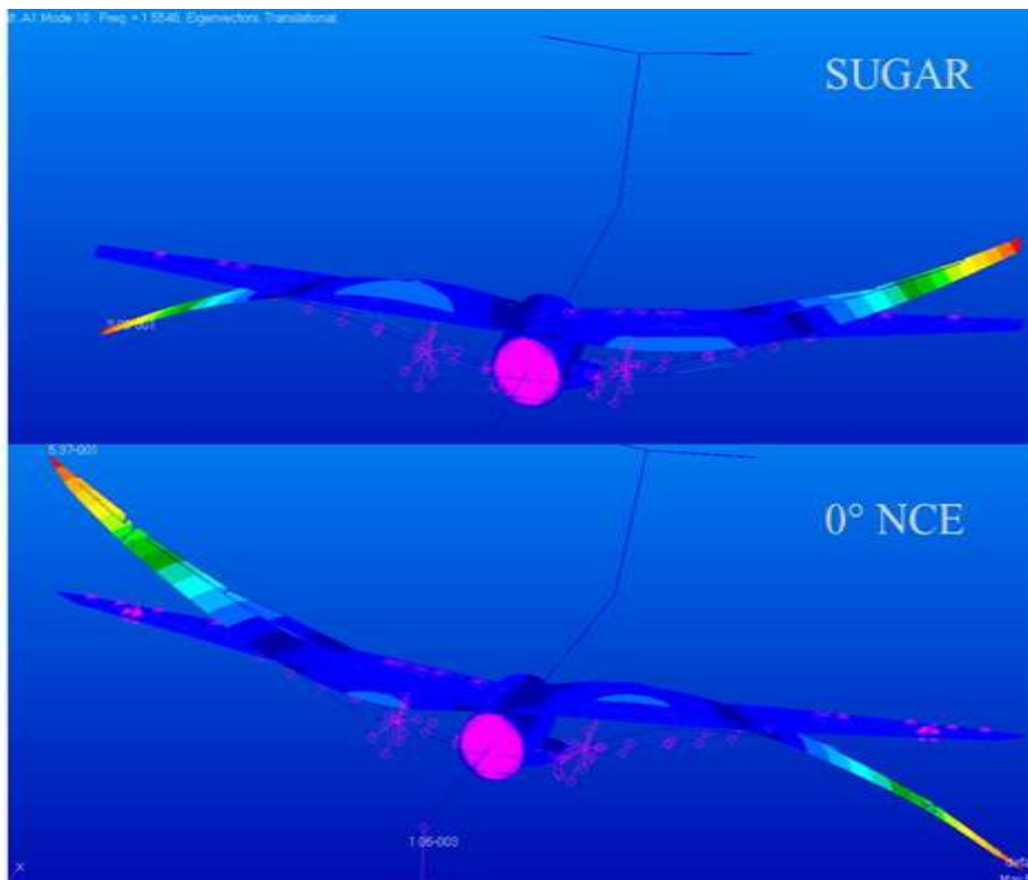
Figure C-4. Full-fuel: Structural mode 10 for baseline SUGAR (1.66 Hz) and 0-deg NCE (1.64) Hz.
