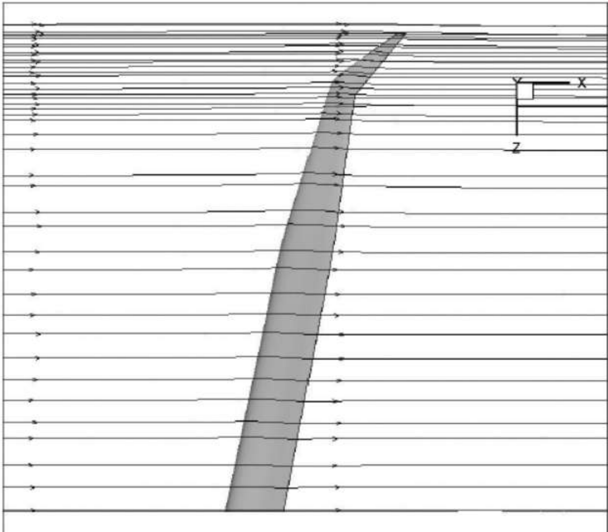
Figure 76. Fluent Prediction of Streamlines over SUGAR Wing with Fully-Swept VGRWT/NCE Tip
