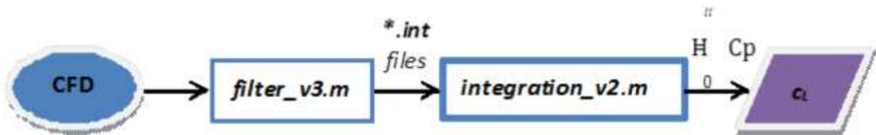
Figure 92. Post-Processing of CFD++ Data for Computing Sectional Lift Coefficient
