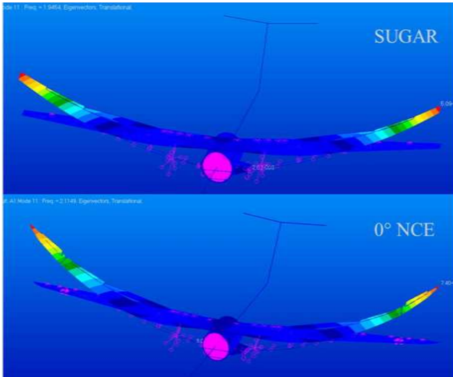
Figure C-5. Full-fuel: Structural mode 11 for baseline SUGAR (1.95 Hz) and 0-deg NCE (2.11) Hz.
