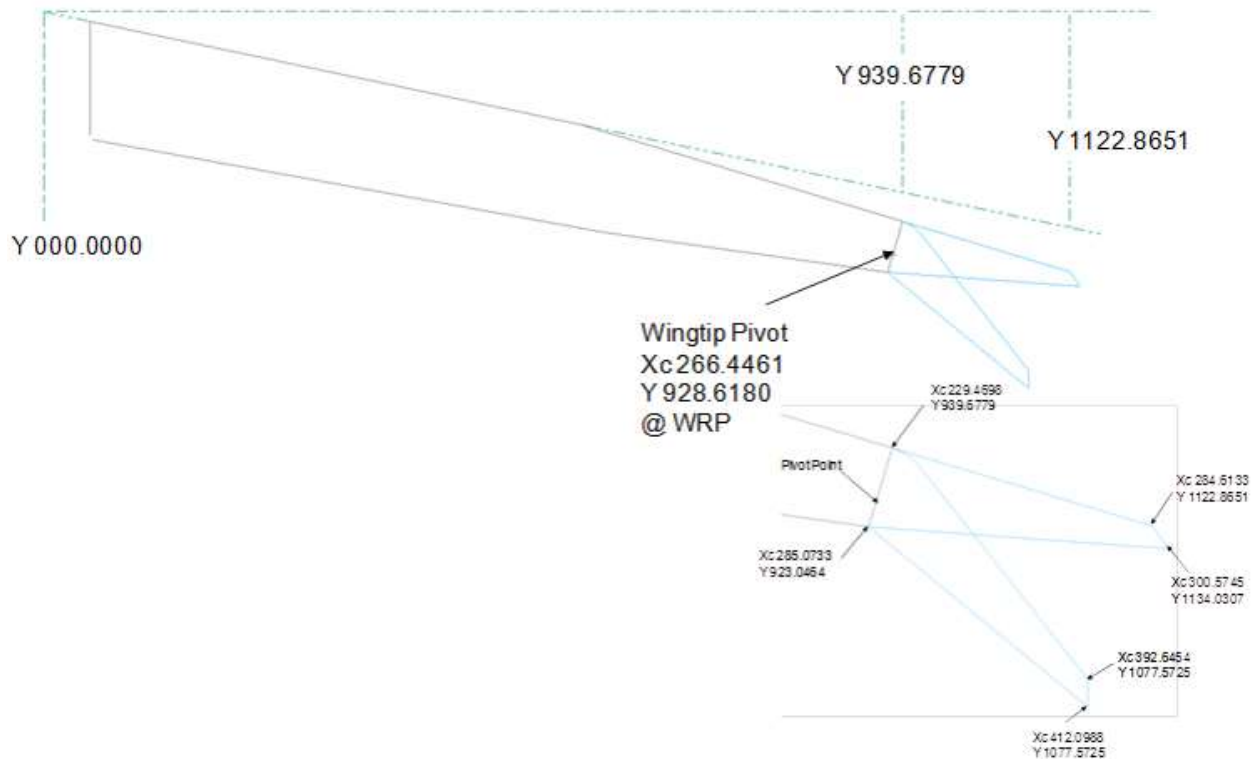
Figure 5. SUGAR Wing with VGRWT Geometry Selected to Maintain Effective Span
