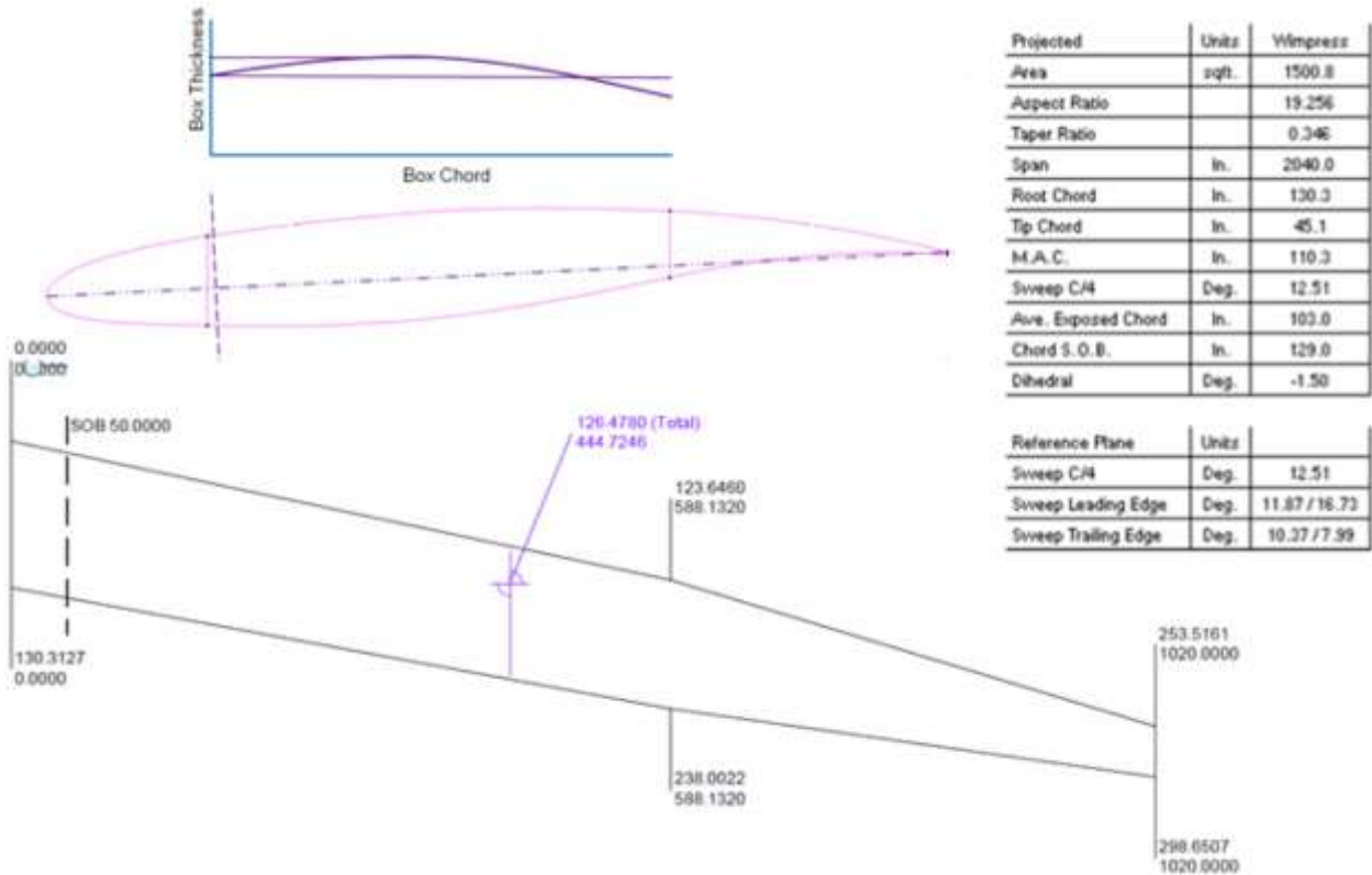
Figure 4. Baseline Wing – SUGAR 765-095-RC, C210b
