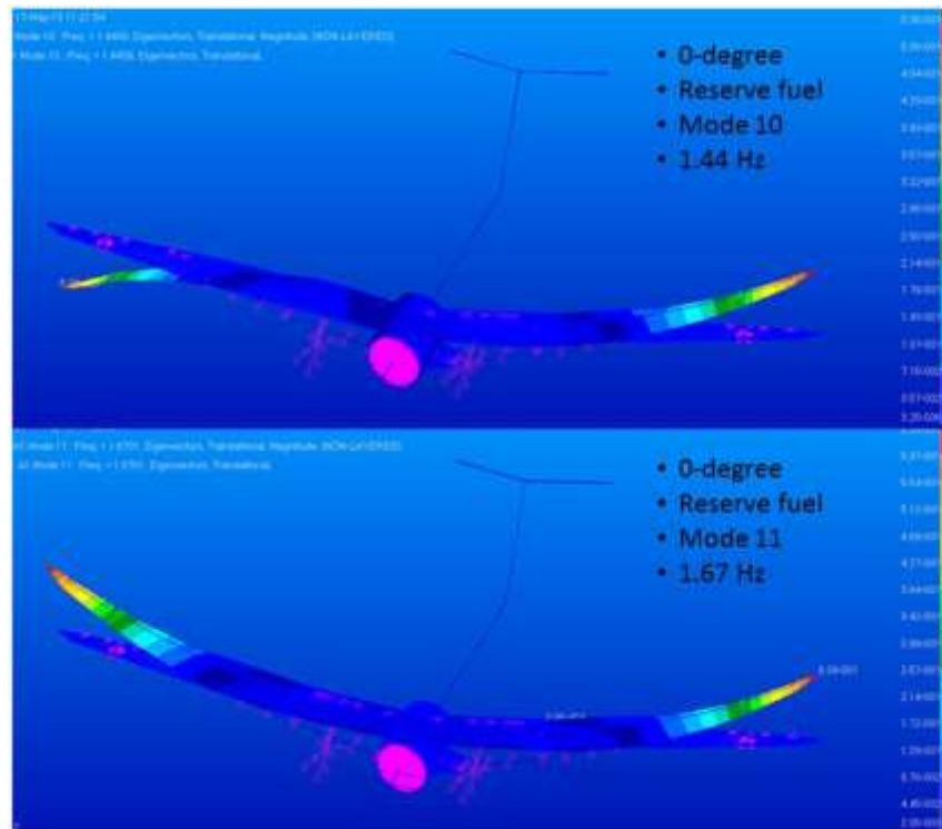
Figure C-13. Reserve-fuel: Structural mode 10 and 11 for 0-deg NCE.
