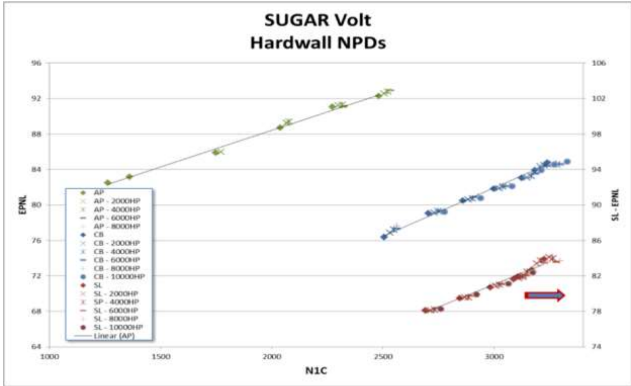
Figure 101. GE Noise-Power-Distance (NPD) Predictions for Hardwall Engine
