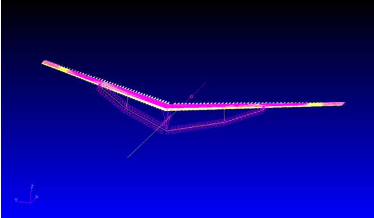
Figure 143. Full Span Structural Model
