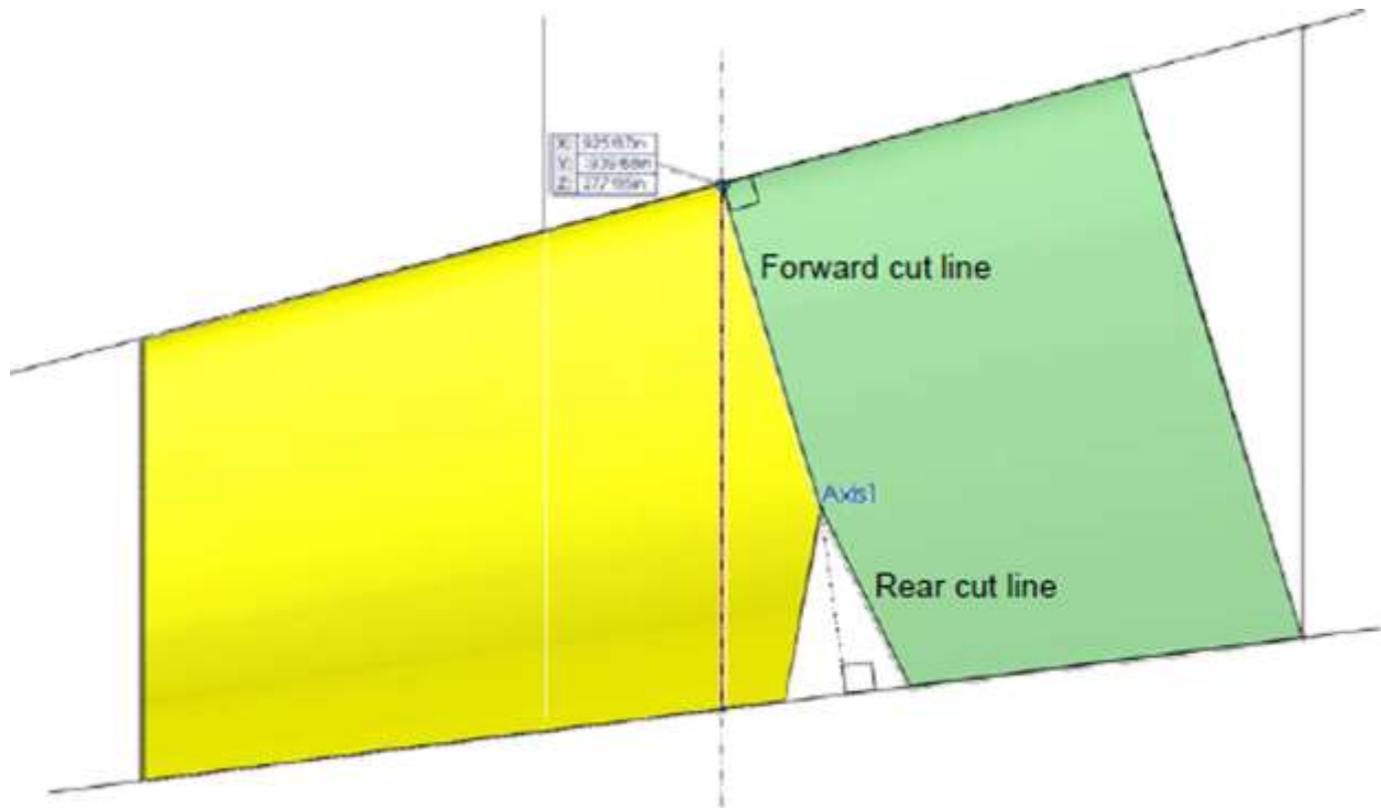
Figure 32. Overview of cutline geometry showing the axis of rotation (Axis 1), the fixed root wing (green), variable wingtip (yellow), and rear fairing clearance cut (white).
