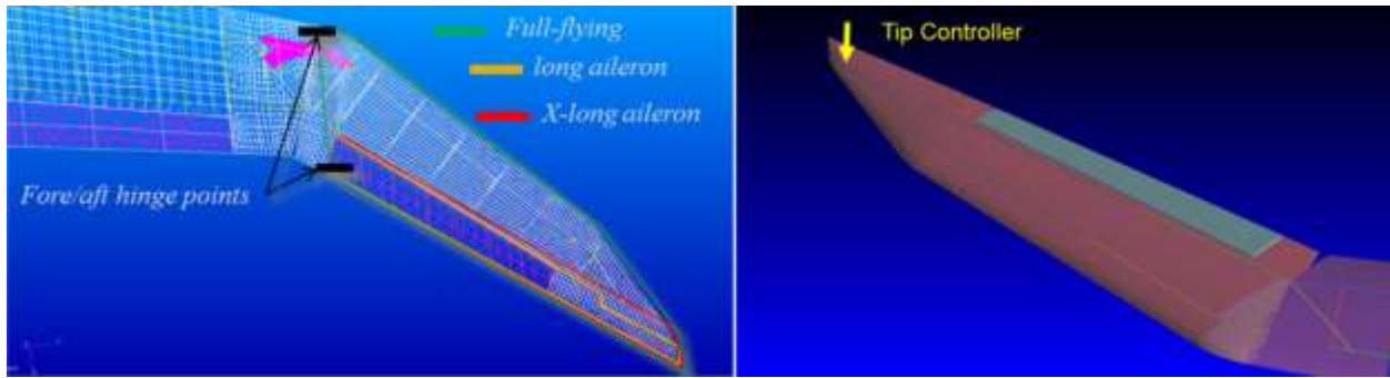
Figure 137. Various control surface arrangements were considered for their ability to achieve the desired aileron reversal control. These variations included ailerons of different sizes, full-flying aileron wingtips with fore (or aft) hinge points, and a point force controller located at the very distal end of the wing.
