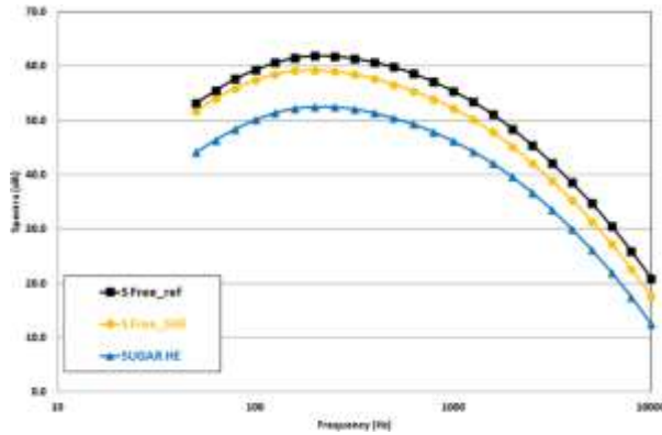
Figure 96. SUGAR Free vs. SUGAR Slat Noise Comparison at Approach
