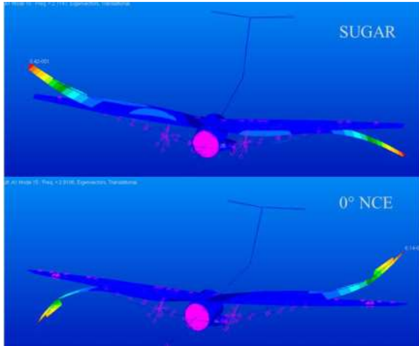
Figure C-9. Full-fuel: Structural mode 15 for baseline SUGAR (2.71 Hz) and 0-deg NCE (2.81) Hz.
