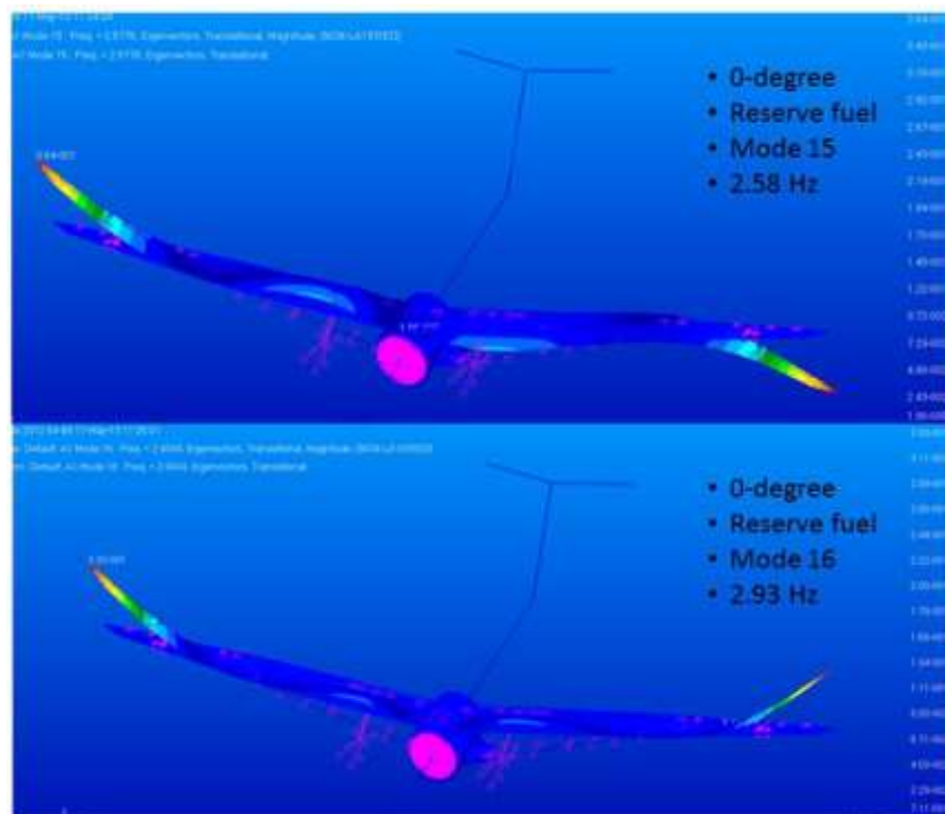
Figure C-14. Reserve-fuel: Structural mode 15 and 16 for 0-deg NCE.
