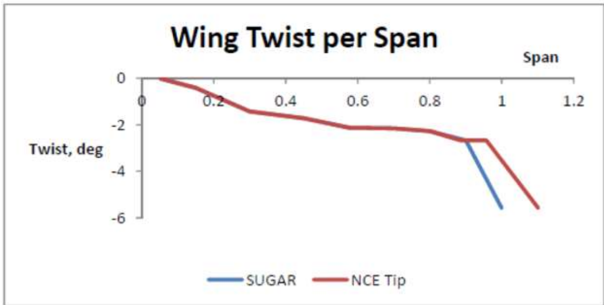
Figure 61. Wing Thickness and Twist per Span for SUGAR and VGRWT/NCE Tip
