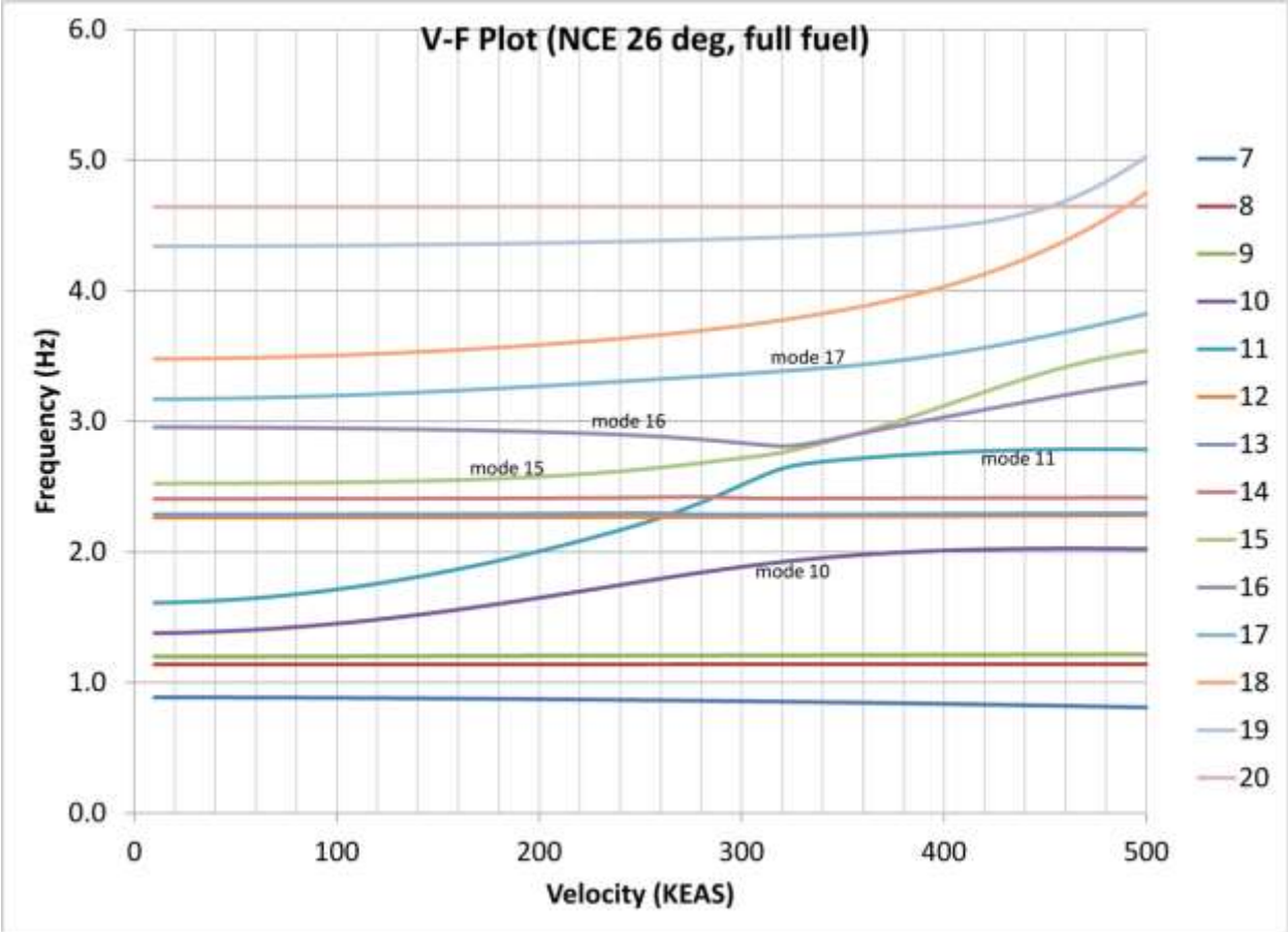
Figure 124. V-F plot for NCE 26-degree full fuel case.
