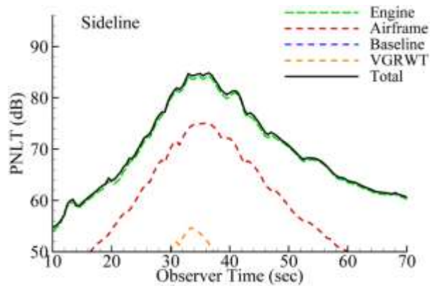
Figure 104. SUGAR/RGWRT Sideline Aircraft Noise
