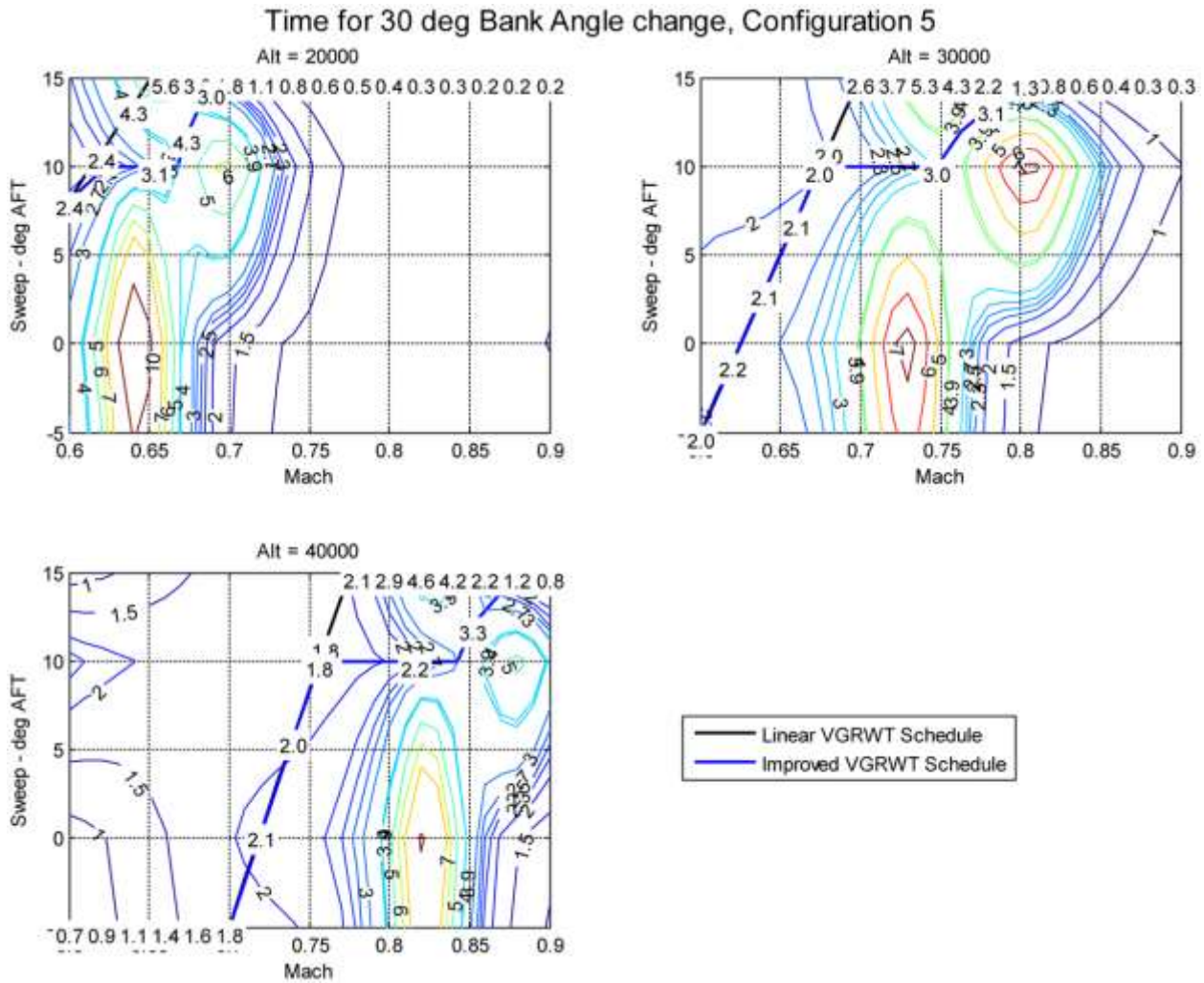
Figure 152. TBW Design 2 Time for 30 deg Bank Angle Change.
