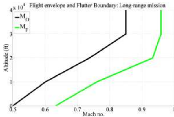
Figure 21. "Boeing 777-like" Vehicle Flight Envelope and Flutter Boundary
