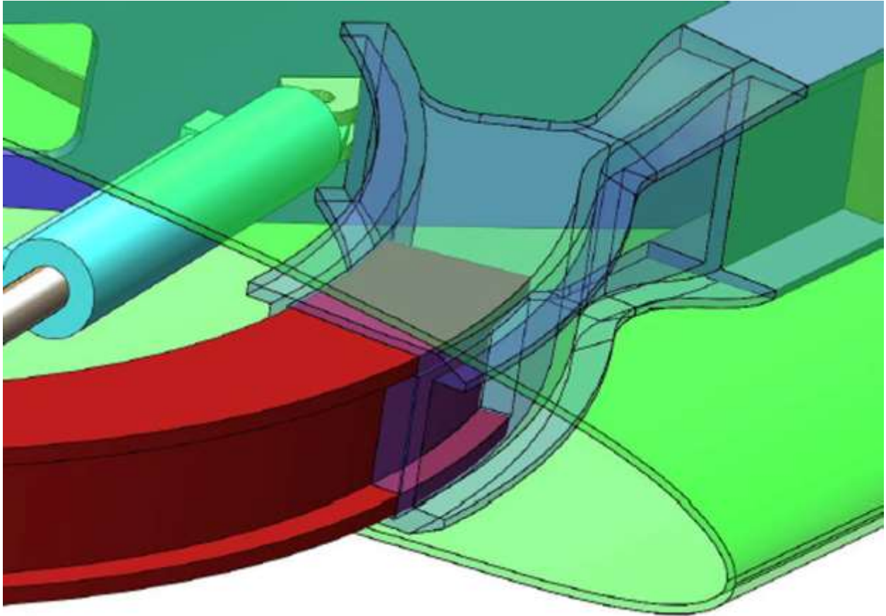
Figure 35. Forward track and beam structure looking in from the wingtip with the wingtip fairing hidden.
