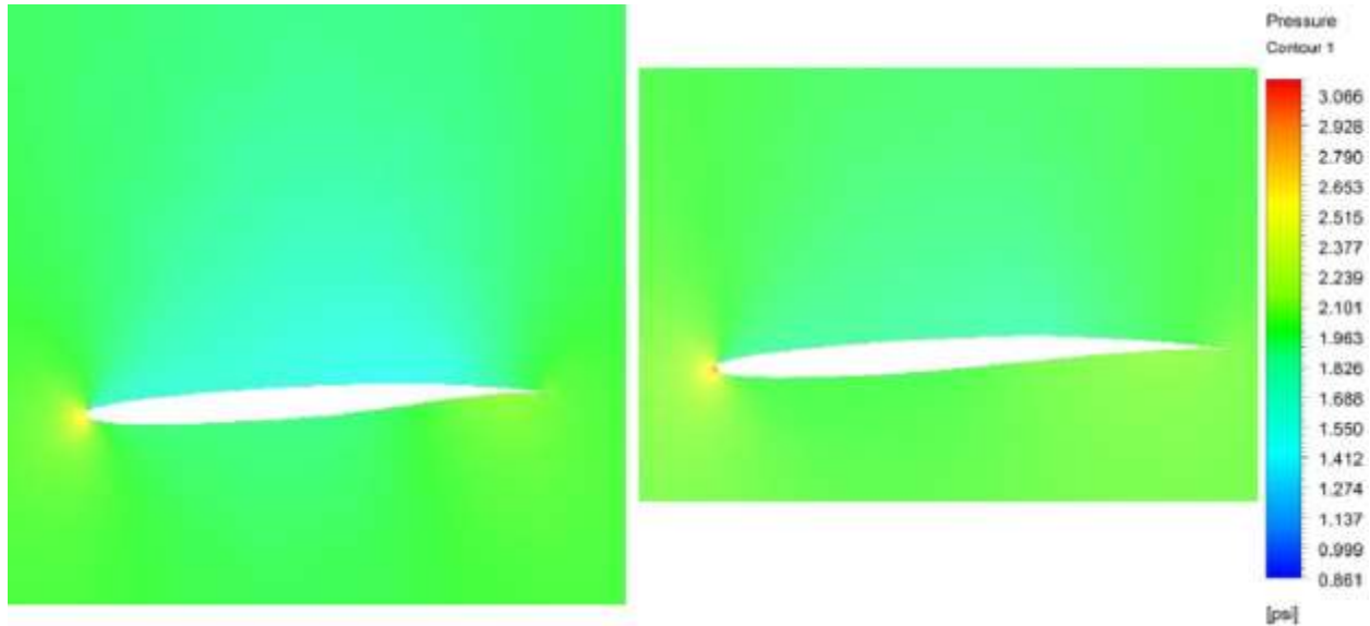
Figure 85. Fluent Prediction of Pressure Contours of Unswept (Left) and Fully-Swept (Right) VGRWT/NCE Wingtip at Main Wing/Wingtip Junction
