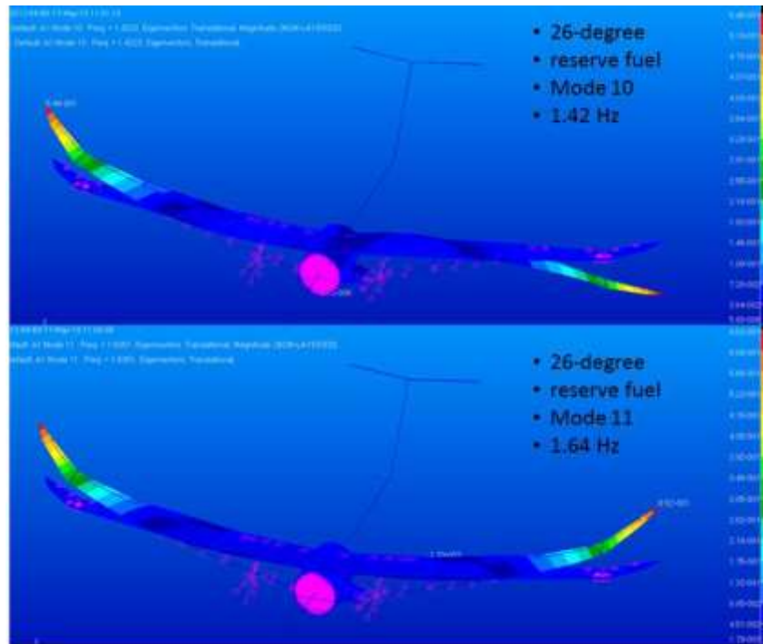
Figure C-17. Reserve-fuel: Structural mode 10 and 11 for 26-deg NCE.
