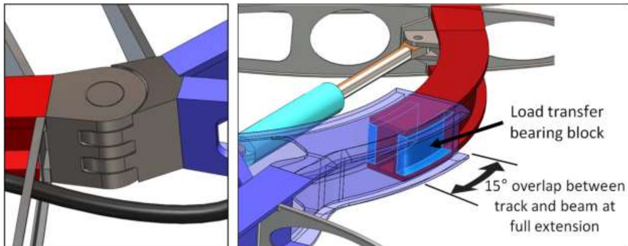
Figure 110. Kinematic model of variable sweep mechanisms showing rear spar pinned hinge pivot joint (left) and forward track and beam (right) with bearing blocks highlighted (light blue) and track structure set to be transparent (clear blue).
