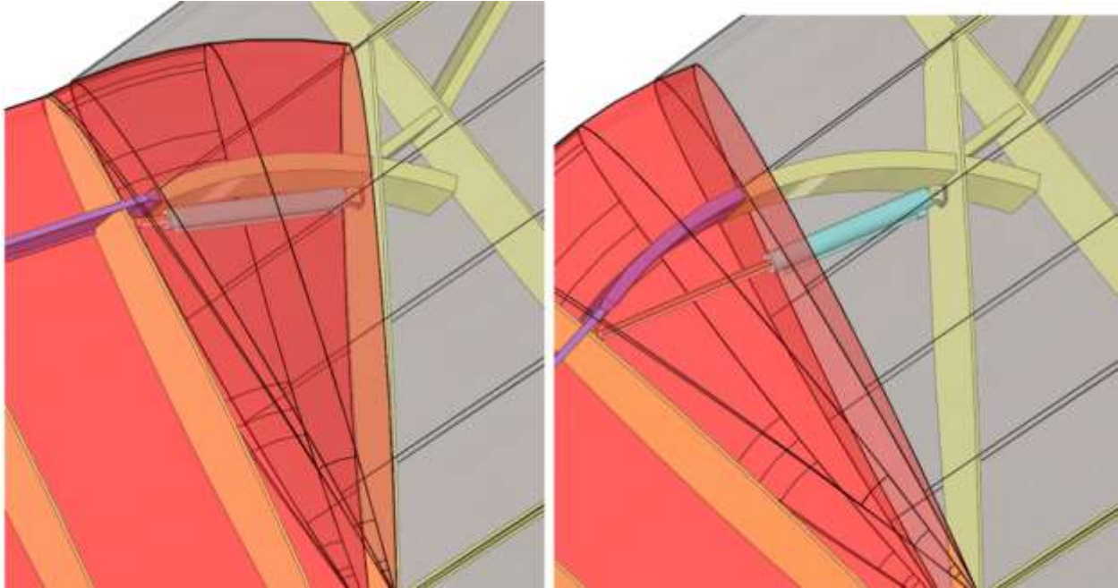
Figure 55. NCE-Wing Joint Showing Actuator Attachment to Wing Rib. Left - NCE Swept Forward 15°; Right - NCE Swept Aft 10°
