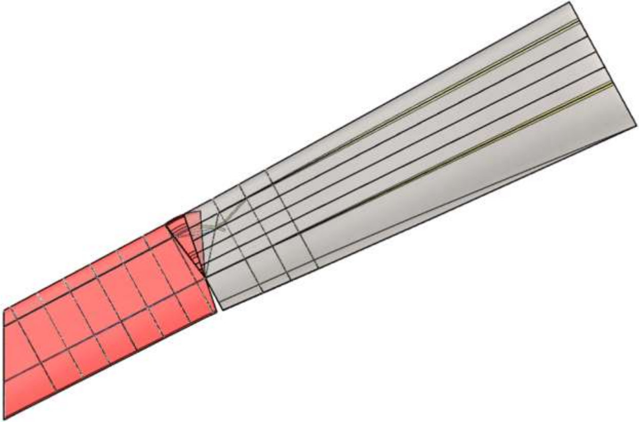
Figure 49. Wingtip with NCE at Zero Sweep
