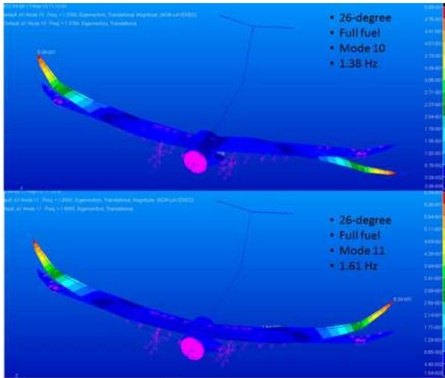
Figure C-15. Full-fuel: Structural mode 10 and 11 for 26-deg NCE.
