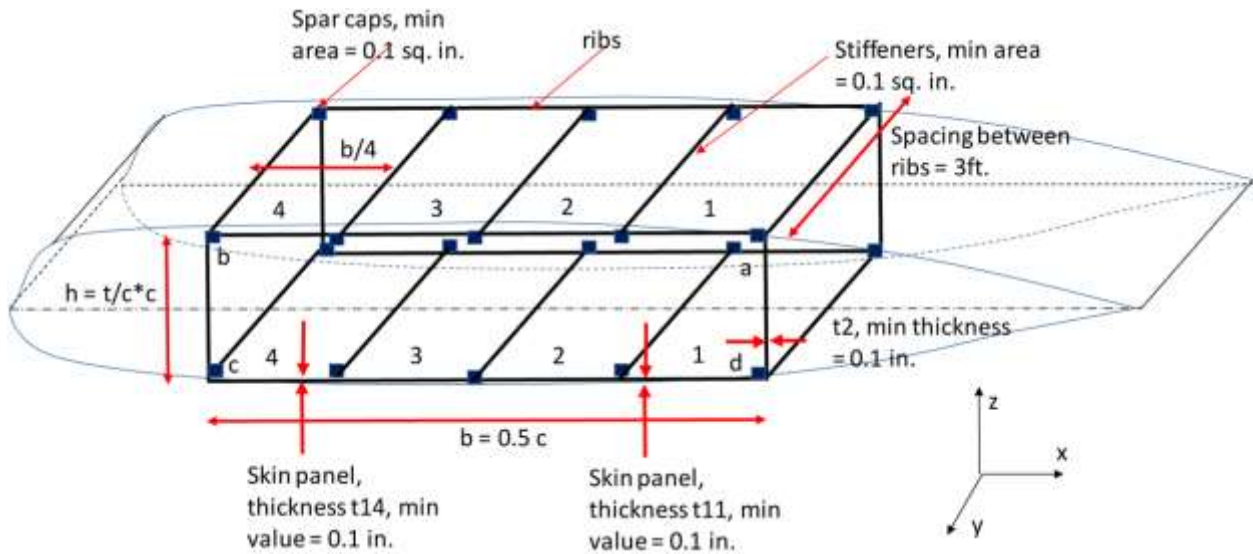
Figure 44. MDO Output Explanation Graphic Provided by VT and Edited by NextGen to Correct Errors and Improve Understanding. Spar Caps and Stiffeners (stringers) have the Same Area in Calculations
