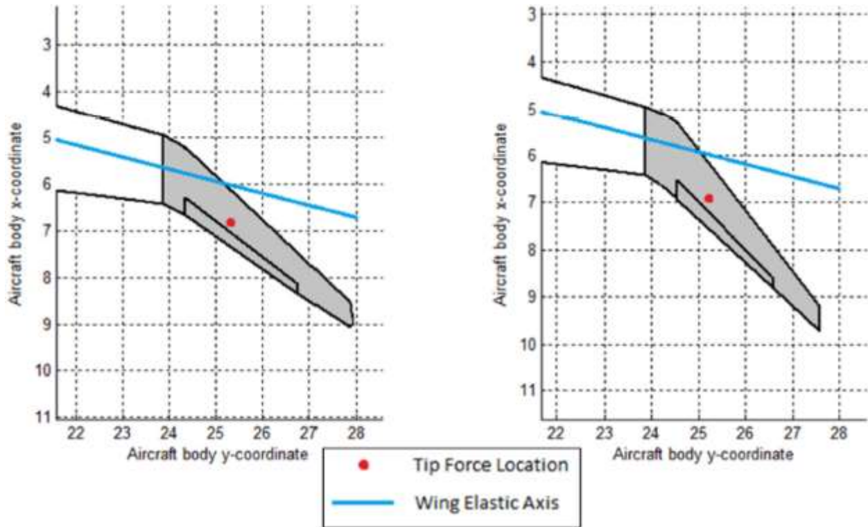
Figure 79. Three-Quarter Sweep VGRWT/NCE Tip (Left) and Full-Sweep VGRWT/NCE Tip (Right) Force Location (Dimensions in Meters)
