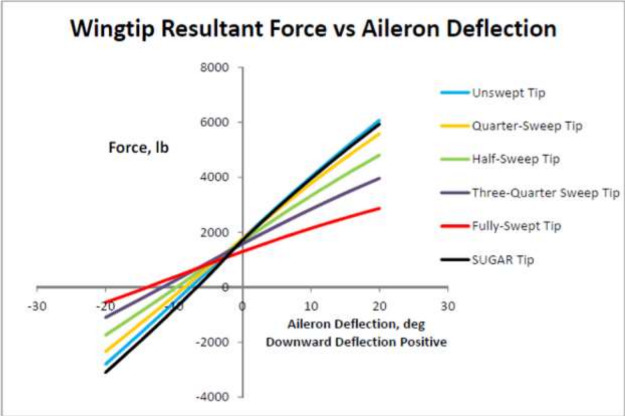
Figure 80. Wingtip Resultant Force as a Function of Sweep and Aileron Deflection
