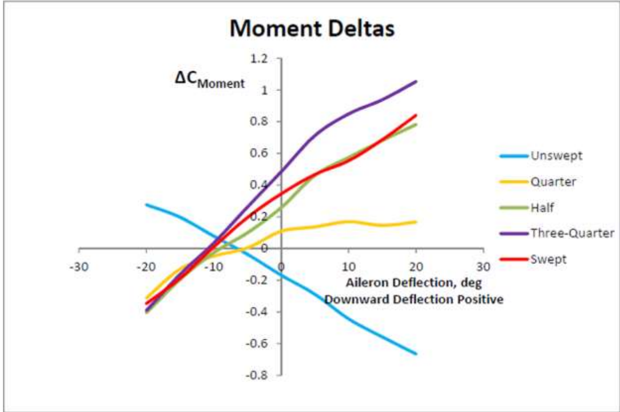
Figure 83. Wingtip Moment Coefficient Deltas for VGRWT/NCE Tip as a Function of Sweep and Aileron Deflection
