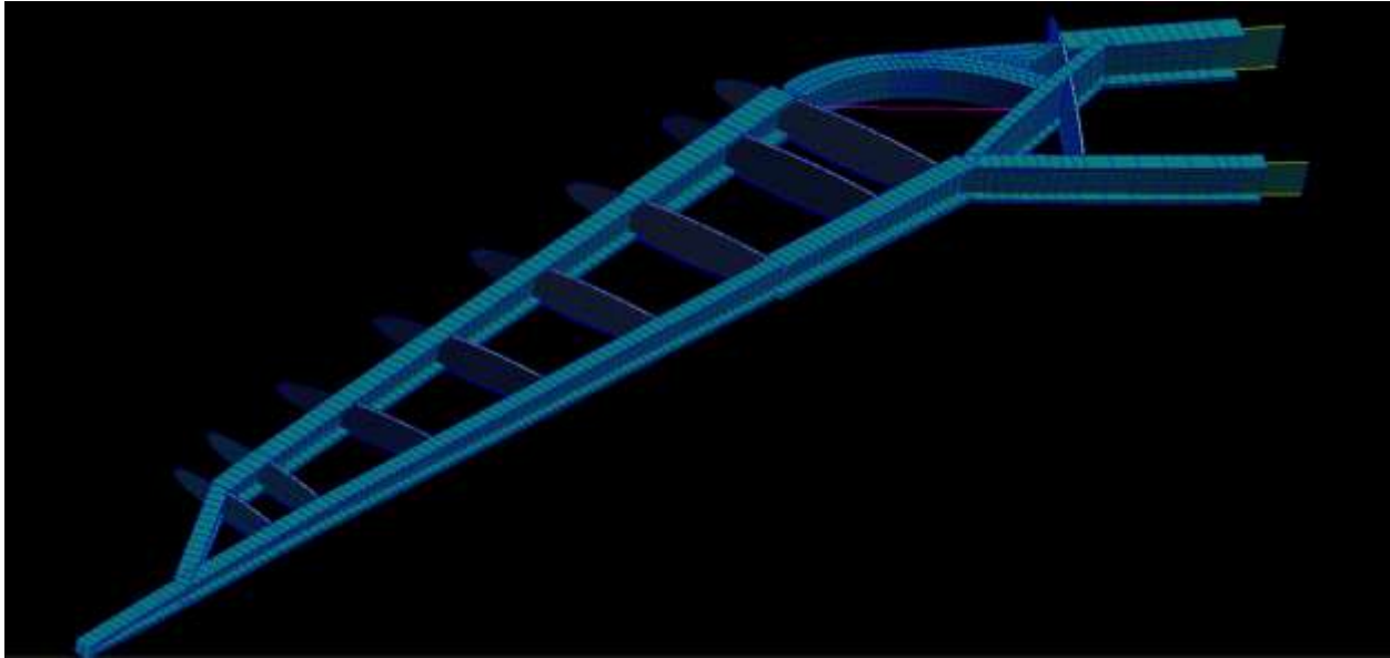
Figure 109. NCE wingtip internal structural mesh showing element basic layout with 2-D beam element dimensions displayed.
