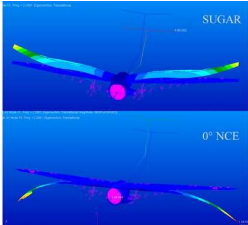
Figure C-7. Full-fuel: Structural mode 13 for baseline SUGAR (2.28 Hz) and 0-deg NCE (2.29) Hz.
