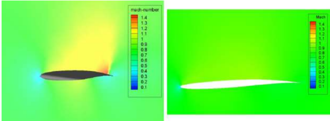
Figure 75. Fluent Prediction of Velocity Profile at Wing Root (Left) and Main Wing/VGRWT Junction (Right)
