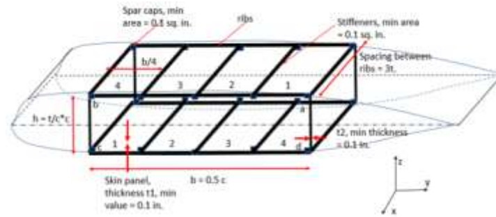
Figure 18(b). New VT MDO Structural Model for Improved Torsional Stiffness Evaluation
