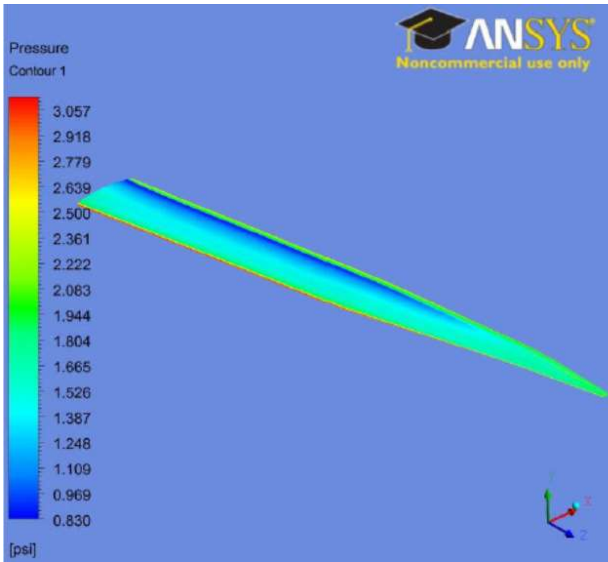
Figure 73. Fluent Prediction of Top Surface Pressure Contours of SUGAR Wing with Unswept VGRWT/NCE Tip
