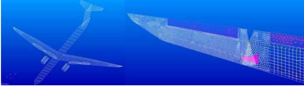
Figure 116. A new aero-mesh (left) was developed for the 0-degree NCE FEM (right).
