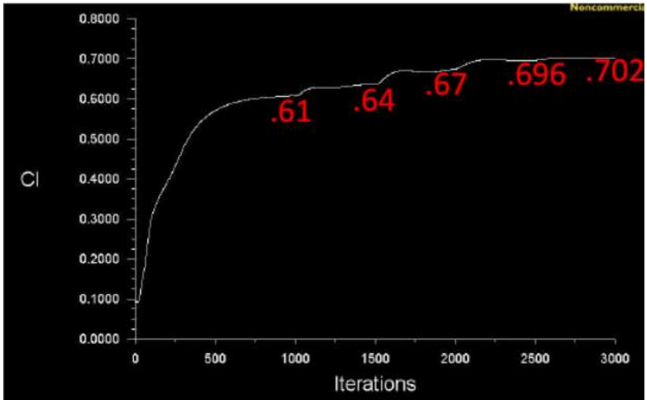
Figure 70. Adaptive Gridding Convergence for Unswept VGRWT/NCE Tip Case (CL in Red)
