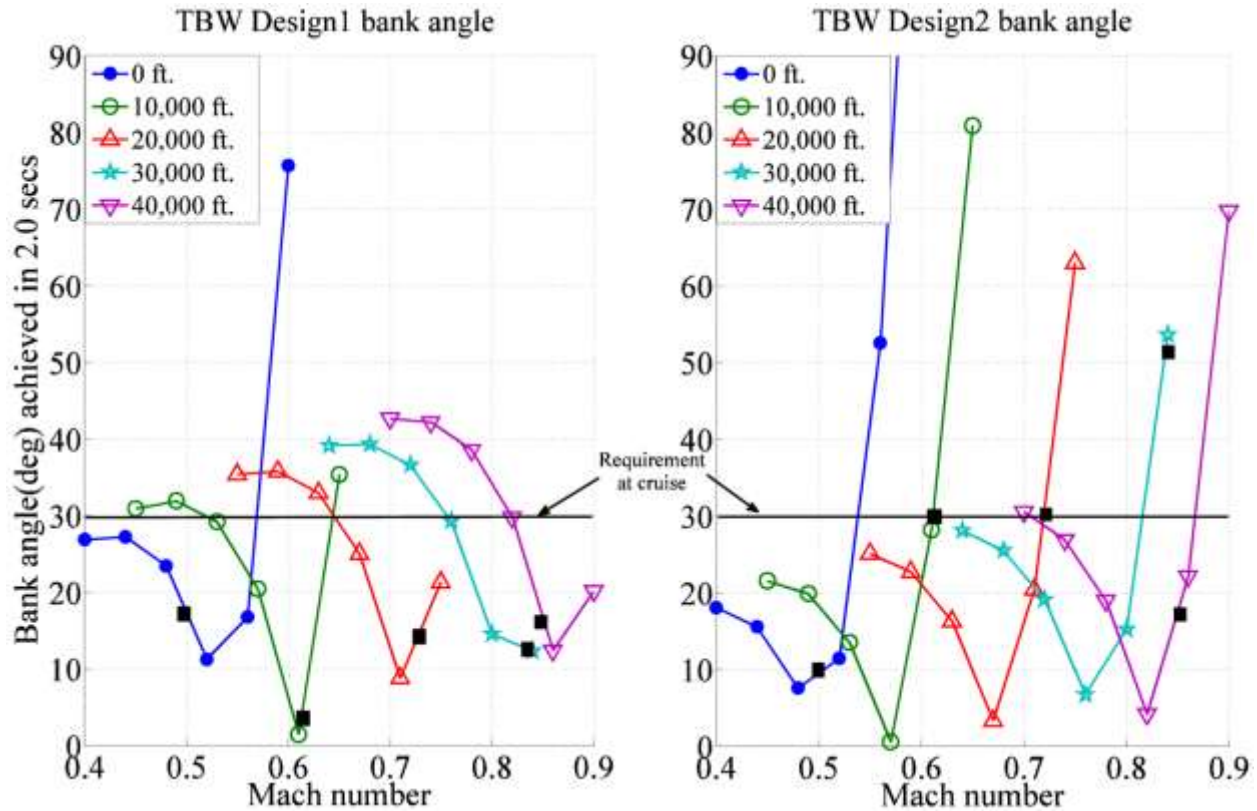
Figure 28. Bank Angles Achieved by TBW Design 1 and TBW Design 2 In 2.0 Seconds with Conventional Aileron
