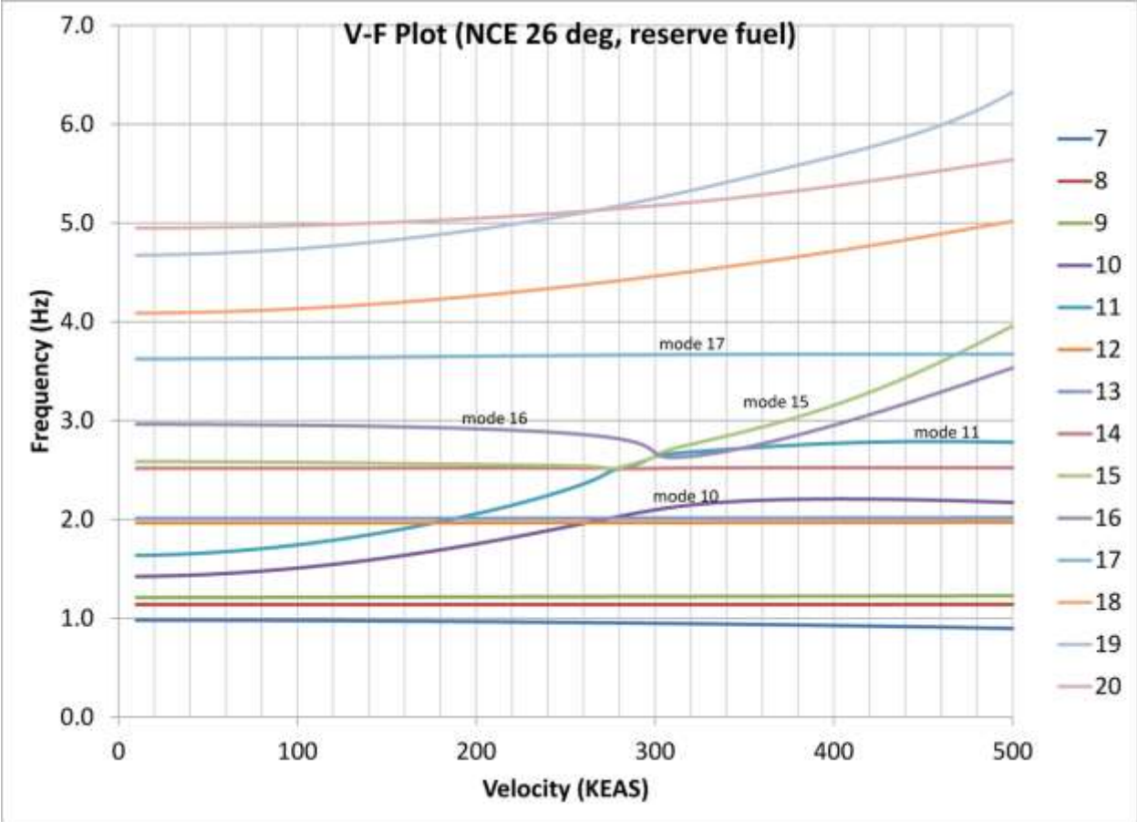
Figure 131. V-F plot for NCE 26-degree reserve fuel case.
