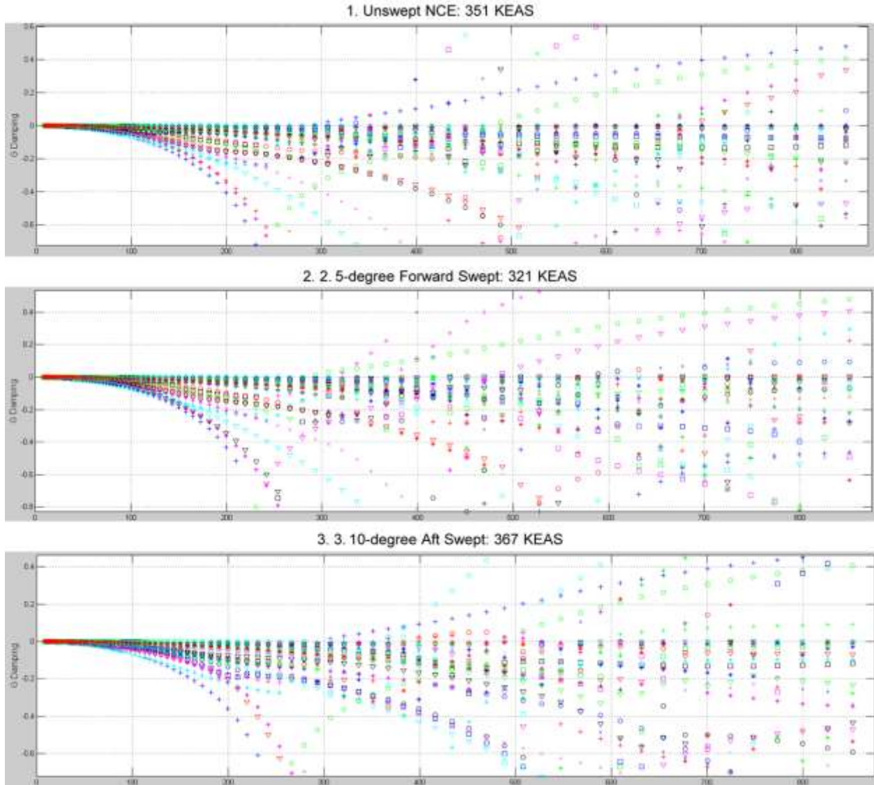
Figure 149. V-G Diagram for Dual Aisle Aircraft with Unswept, 5° Forward Swept, and 10° Aft Swept Novel Control Effector Wing Tip
