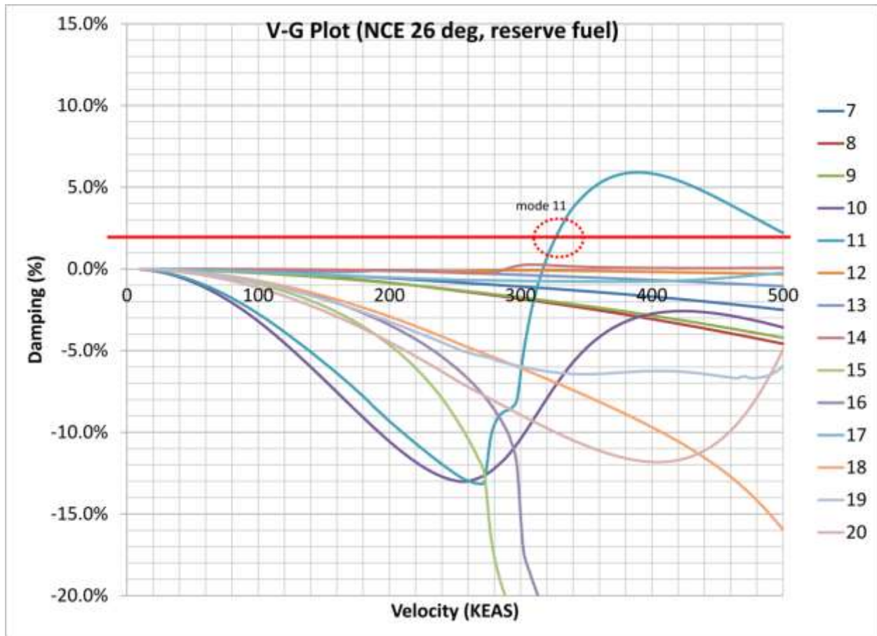
Figure 132. V-G plot for NCE 26-degree reserve fuel case.
