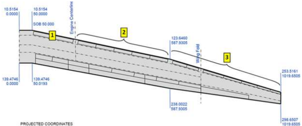
Figure 95. SUGAR Slat System Definition for Noise Analysis
