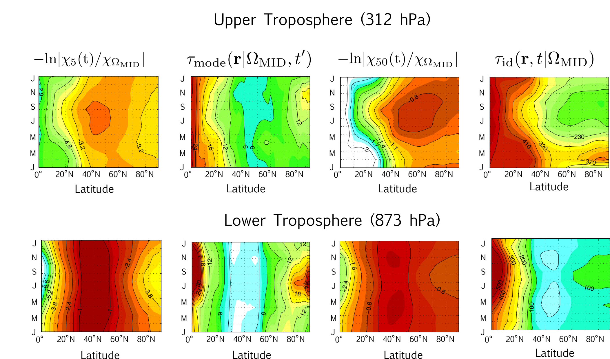
Figure 5: The seasonal cycles \chi_{\tau_c}(\mathbf{r}, t|\Omega_{MID})/\chi_{\Omega_{MID}} for \tau_c = 5 days (column 1) and \tau_c = 50 days (column 3). The seasonal cycles of the modal age and the ideal age (equivalent to the mean age) are shown in columns 2 and 4.
