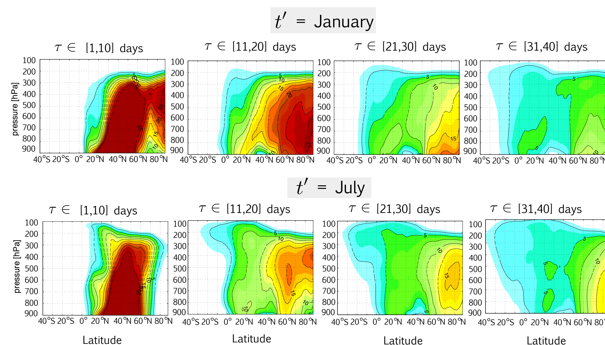
Figure 3: The zonal mean BIR fraction, f_{\tau_1}^{\tau_2}(\mathbf{r}|\Omega_{MID}, t') , corresponding to source times t' = January 1 (top) and t' = July (bottom). 10-day successive transit-time bands provide a sense for the fast transport paths that connect the midlatitude surface to the rest of the troposphere (units: %).
