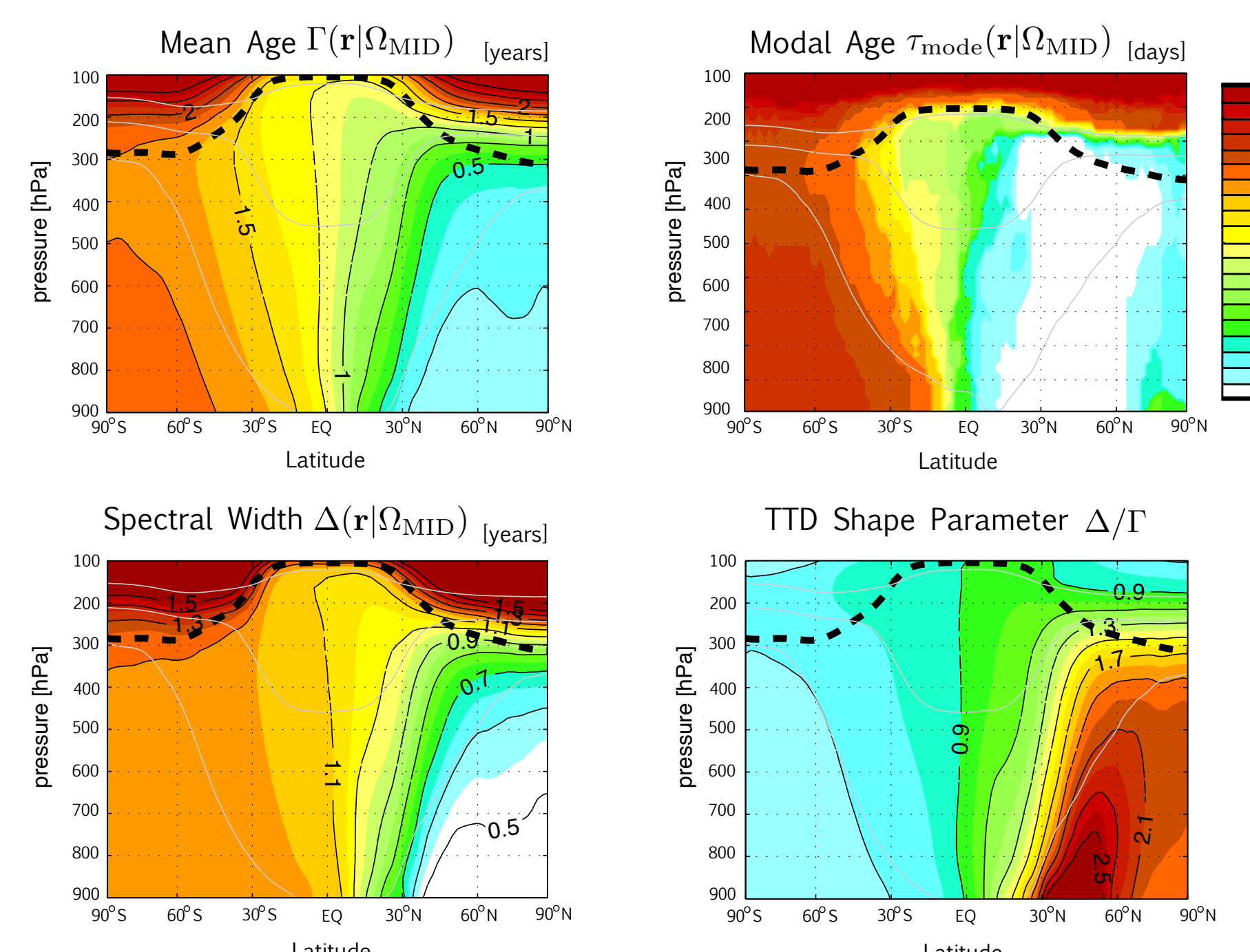
Figure 2: The mean age (top left), modal age (top right), and spectral width (bottom left), calculated from the approximation of the TTD, \mathcal{G}(\mathbf{r}, \tau|\Omega_{MID}) . The ratio \Delta/\Gamma provides a measure of the shape of the TTD (bottom right).
