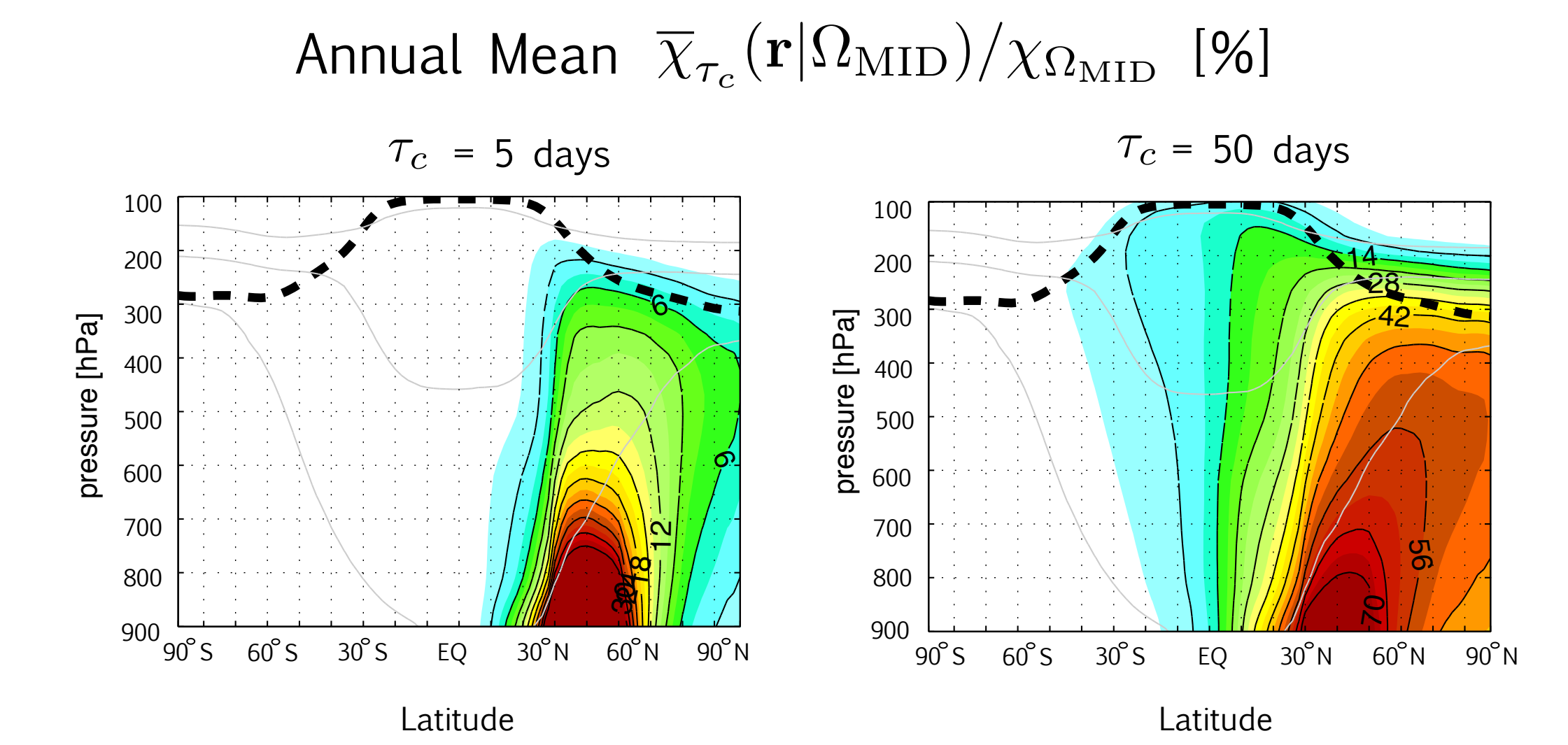
Figure 4: The annually averaged concentrations of the idealized 5-day and 50-day tracers. Reconstructions of \chi_{\tau_c} using the convolution \bar{\chi}_{\tau_c}(\mathbf{r}|\Omega_{MID})/\chi_{\Omega_{MID}} \equiv \int_0^{\infty} d\tau \mathcal{G}(\mathbf{r}, \tau|\Omega_{MID}) e^{-\tau/\tau_c} compare well with the explicitly calculated tracers.
