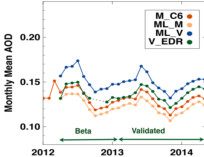
0.55 \mu\text{m} AOD, Ocean
