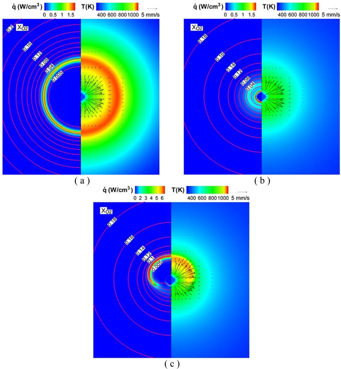
Figure 2: Calculated structure of zero-gravity n-heptane flames in quiescent air (the field of view: 80 mm \times 80 mm): (a) near-extinction diffusion flame, t = 6 s; (b) near-reignition cool flame, t = 24 s; and (c) reignited propagating flame, t = 25 s
