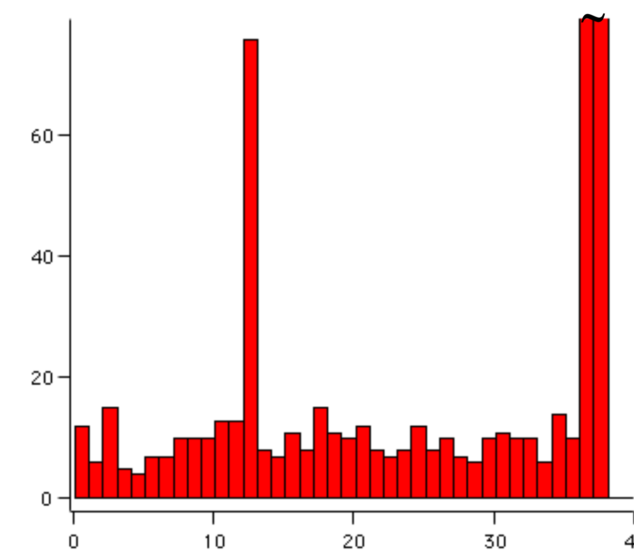
Number of events on each channel in coincidence with an anti-co event. The two anti-co channels are at 36, 37, and their data are cut off. Channel 12, the calibration pixel, is illuminated by an internal collimated source; it exhibits false coincidence.
