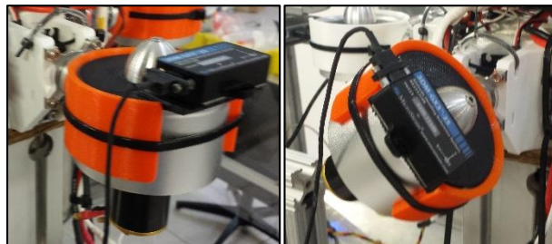
Figure 7: Microstrain IMU measuring thrust angle on Mini Free Flyer
