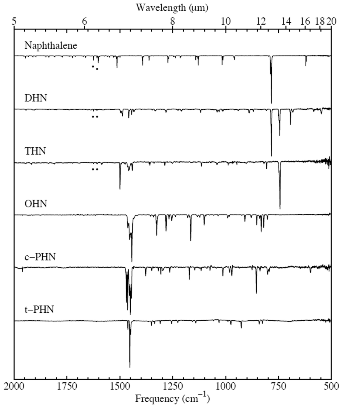
Figure 2. The 2000-500 \text{cm}^{-1} spectral region transmission spectra of molecules in Series A (naphthalene skeletal structure). The spectrum of naphthalene is from Hudgins et al. (1994). An (*) denotes bands due to trace \text{H}_2\text{O} contamination.
