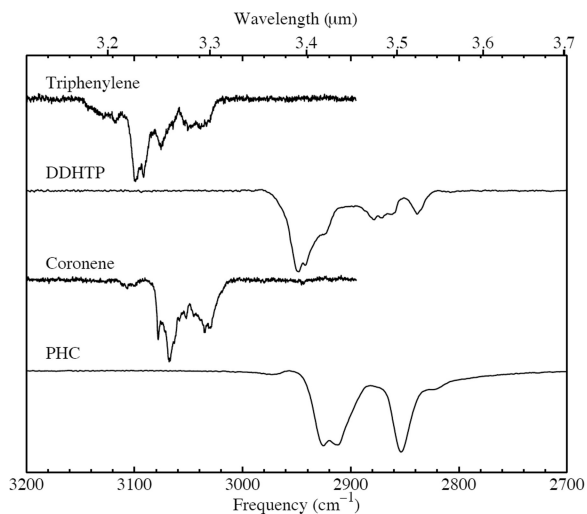
Figure A9: The 3200-2700 \text{cm}^{-1} CH stretch region transmission spectra of molecules in Series F. The spectrum of triphenylene is taken from Hudgins & Sandford (1998a) and coronene is taken from Hudgins & Sandford (1998b).
