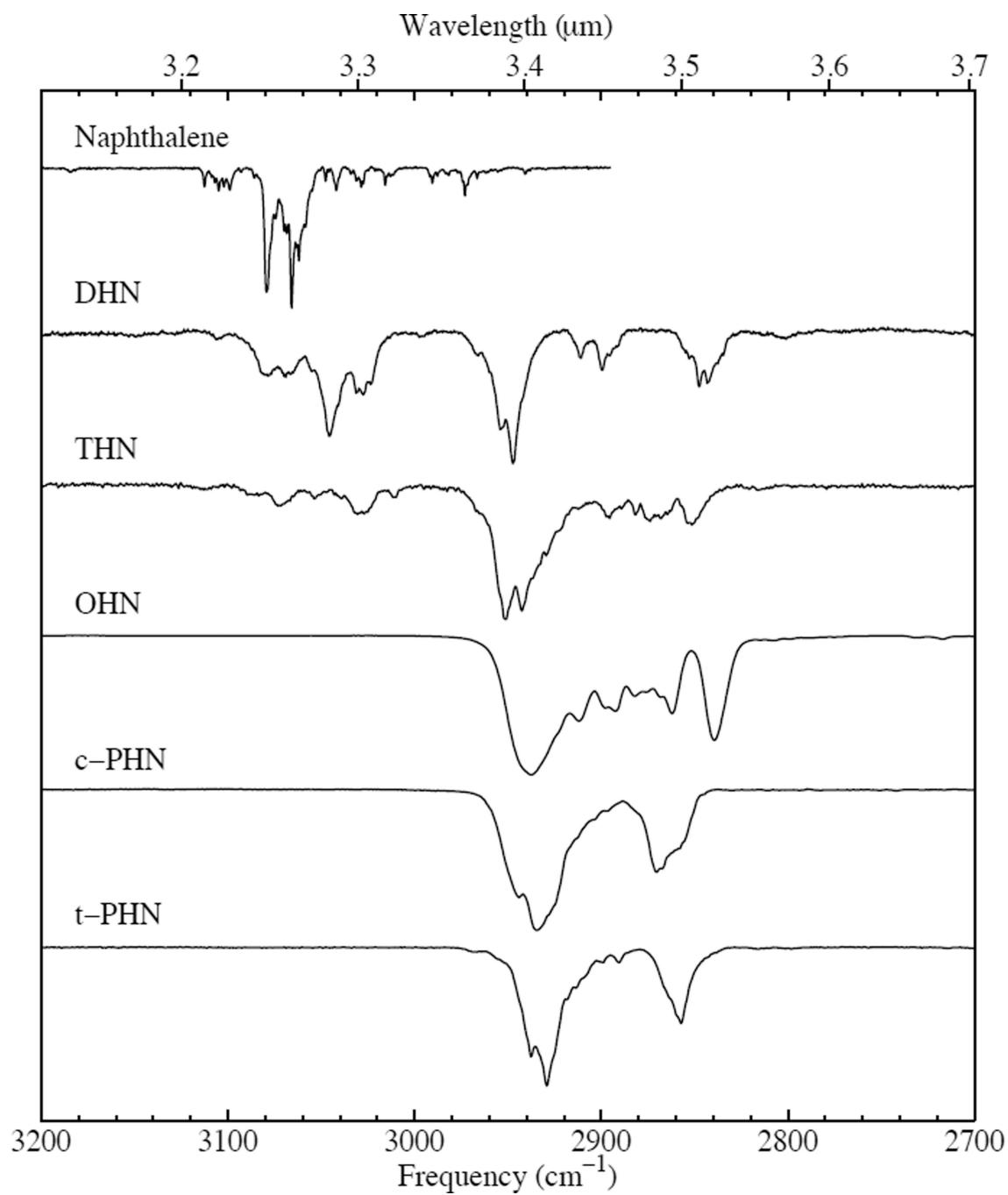
Figure 1. The 3200-2700 cm -1 C-H stretch region transmission spectra of molecules in Series A (naphthalene skeletal structure). The spectrum of naphthalene is from Hudgins et al. (1994).
