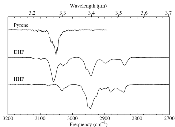
Figure A5: The 3200-2700 \text{cm}^{-1} CH stretch region spectra of molecules in Series D (pyrene skeletal structure). The spectrum of pyrene is taken from Hudgins & Sandford (1998a).
