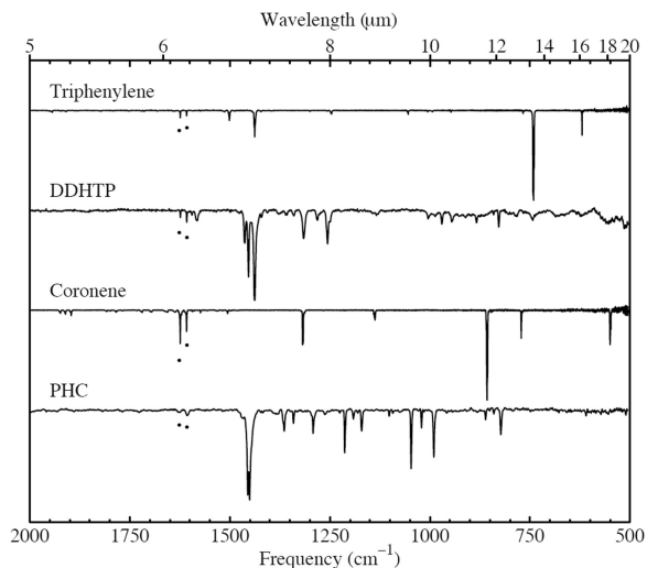
Figure A10: The 2000-500 \text{cm}^{-1} spectral region transmission spectra of molecules in Series F. The spectrum of triphenylene is taken from Hudgins & Sandford (1998a) and coronene is taken from Hudgins & Sandford (1998b). An (*) denotes bands due to trace \text{H}_2\text{O} contamination.
