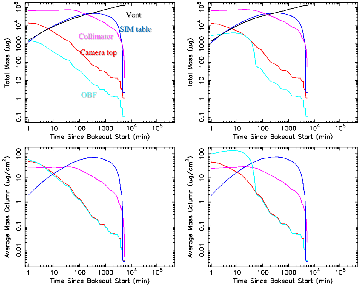
Figure 12. CCMM simulations for an ACIS room-temperature bake-out of an example molecular contaminant—octadecane, slightly de-rated to match the volatility of DOP at low temperatures (see text). Left panels show results for a warm ( +25^{\circ}\text{C} ) focal plane; right panels, for a cool ( -60^{\circ}\text{C} ) focal plane. Upper panels plot the total contaminant mass on each component; lower panels, the average mass column on each component.
