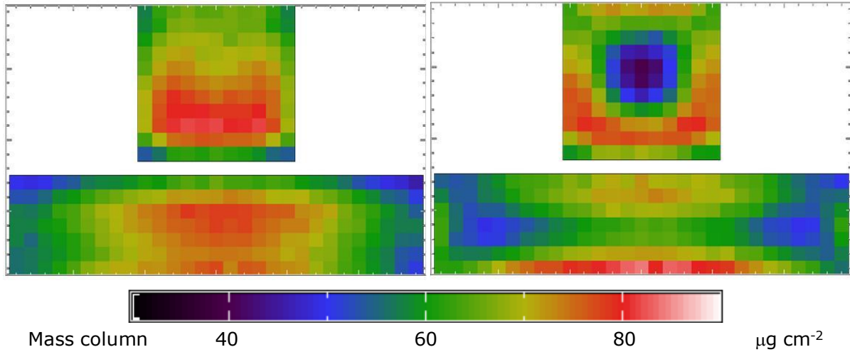
Figure 9. Distribution of mass column of accumulated contamination on the ACIS OBFs, based upon molecular-transport simulations for a contaminant of relatively low volatility (left panel) and for one of relatively moderate volatility (right panel).
