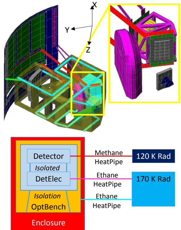
Figure 2. WFI Instrument Cycle 3 Thermal Model: The optical bench includes two planar ethane heatpipes (cyan) to isothermize, which are connected to a 170 K picture frame radiator. Two methane heatpipes (red) connect the FPA to a central 120 K radiator. Two ethane heatpipes (magenta) connect the FPA cold electronics to the 170 K radiator. A low conductivity composite frame separates the FPA from the cold electronics.
