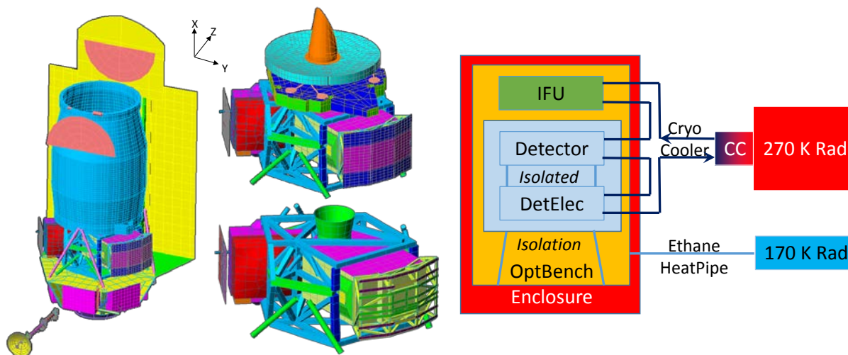
Figure 8. WFIRST Observatory Cycle 5 Thermal Model: Telescope, AMS now supported by Instrument carrier, Instrument Carrier now a truss structure with no sandwich plate on top, WFI with 270 K and 170K radiators and no instrument side avionics, and CGI (Top Middle), and Instrument Carrier, CGI and WFI Enclosure and Heatpipes (Bottom Middle) and WFI Thermal Block Diagram (Right)
