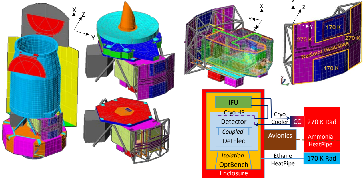
Figure 4. WFIRST Observatory Cycle 4 Thermal Model: Telescope, AMS, Instrument Carrier no longer includes truss; WFI with 270 K and 170K radiators and instrument side avionics, and CGI (Top Right), and Instrument Carrier, CGI and WFI Enclosure and Heatpipes (Bottom Right).
