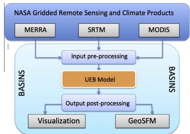
Fig. 2. General modeling framework of HIMALA BASINS system, integrating UEB with GeoSFM.
