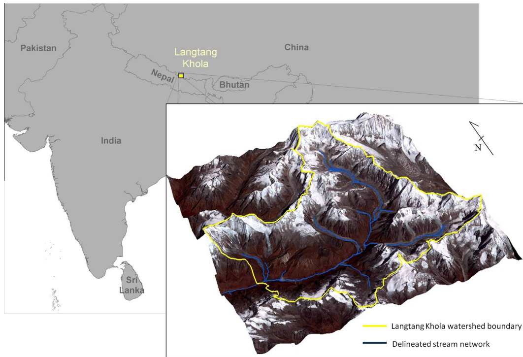
Fig. 1. Langtang Khola watershed in the Koshi in Nepal where HIMALA BASINS test data was developed and evaluated.
