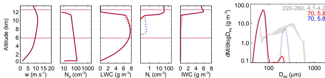
Figure 6. As in Fig. 4 for simulations that also include a pseudo-Hallett–Mossop source producing 1 std \text{cm}^{-3} splinters with baseline updraft strength scaled by factors of 0.5 (red solid line), 1.0 (blue dotted line, same as in Fig. 5), and 1.5 (green dashed line). Note that vertical scale for ice PSDs is logarithmic in preceding figures so that insubstantial larger mode is evident, but is linear hereafter.
