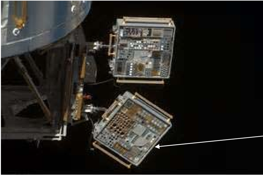
Laser Markable Aluminum Labels Installed on MISSE 6A
